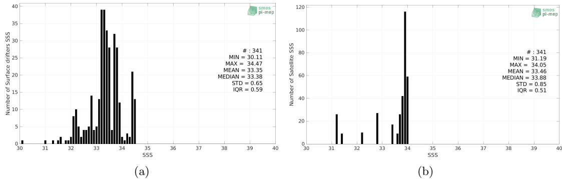
Figure 2: Histograms of SSS from Surface drifters (a) and SMAP SSS L3 v5 - Monthly (RSS) (b) considering all match-up pairs per bins of 0.1 over the Arctic Ocean Pi-MEP region and for the full satellite product period.
