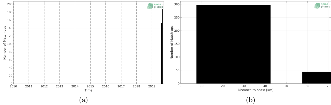
Figure 1: Number of match-ups between Surface drifters and SMAP SSS L3 v5 - Monthly (RSS) SSS as a function of time (a) and as function of the distance to coast (b) over the Arctic Ocean Pi-MEP region and for the full satellite product period.
