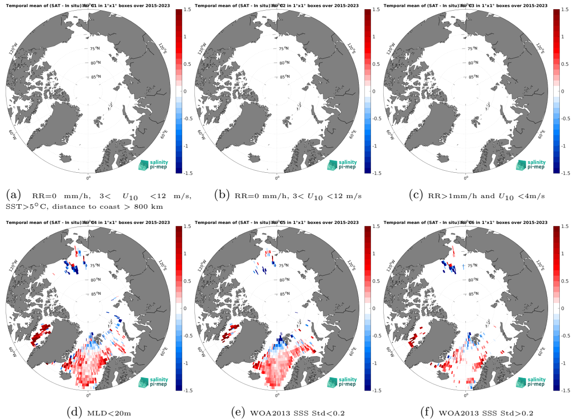
Figure 12: Temporal mean gridded over spatial boxes of size 1^{\circ}\times 1^{\circ} of \Delta\text{SSS} (SMAP SSS L3 v5 - Monthly (RSS) - Argo) for 6 different subdatasets corresponding to: RR=0 mm/h, 3 < U_{10} < 12 m/s, SST > 5^{\circ}\text{C} , distance to coast > 800 km (a), RR=0 mm/h, 3 < U_{10} < 12 m/s (b), RR > 1 mm/h and U_{10} < 4 m/s (c), MLD < 20\text{m} (d), WOA2013 SSS Std < 0.2 (e), WOA2013 SSS Std > 0.2 (f).
