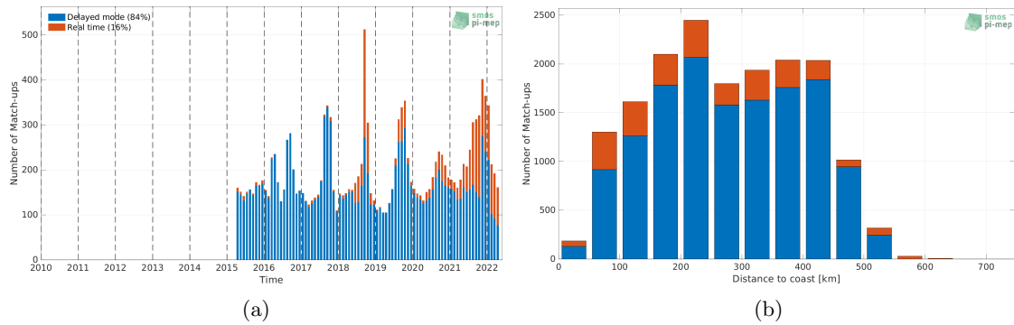
Figure 1: Number of match-ups between Argo and SMAP SSS L3 v5 - Monthly (RSS) SSS as a function of time (a) and as function of the distance to coast (b) over the Arctic Ocean Pi-MEP region and for the full satellite product period.
