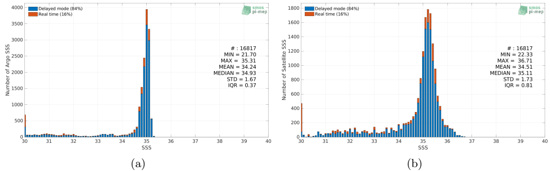
Figure 2: Histograms of SSS from Argo (a) and SMAP SSS L3 v5 - Monthly (RSS) (b) considering all match-up pairs per bins of 0.1 over the Arctic Ocean Pi-MEP region and for the full satellite product period.
