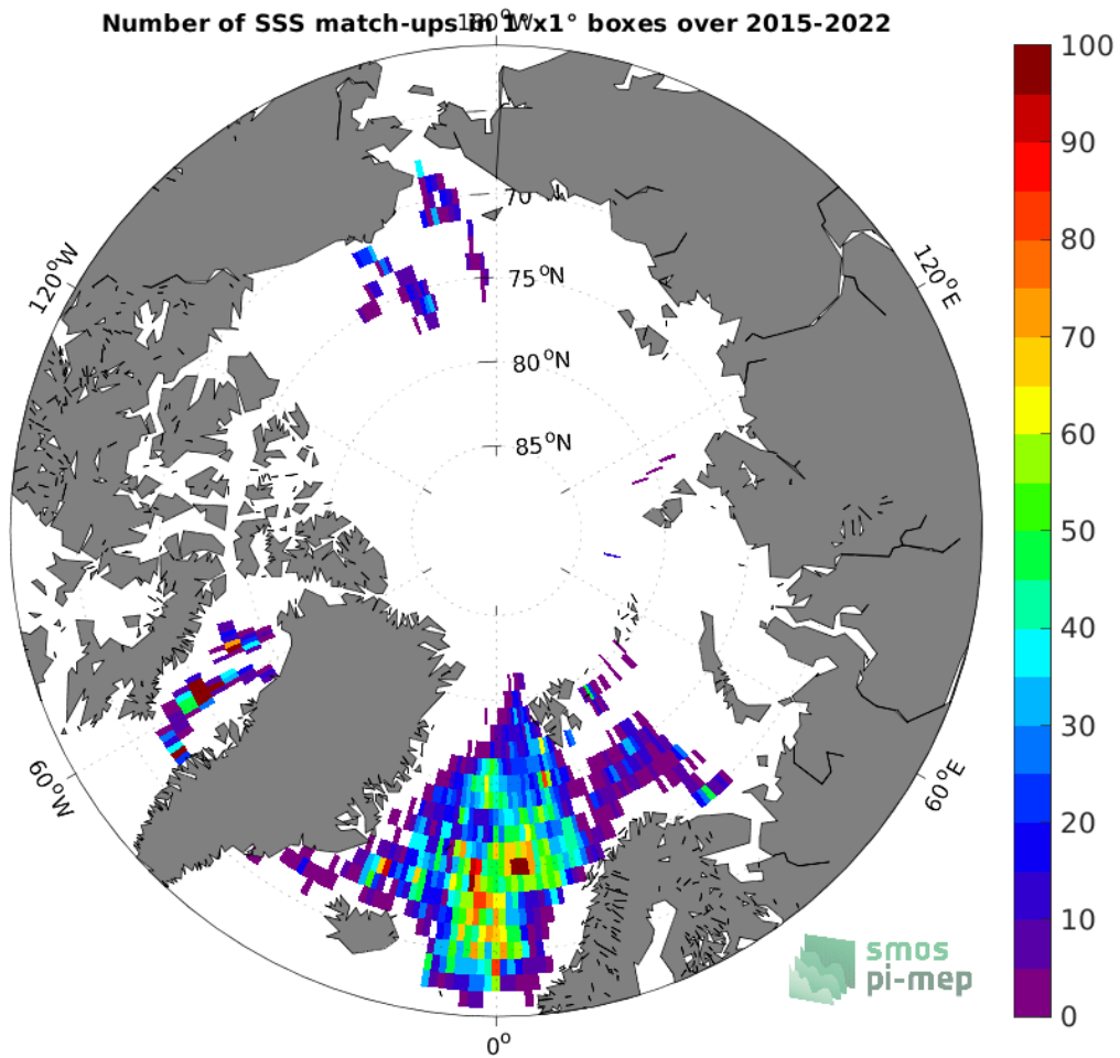
Figure 4: Number of SSS match-ups between Argo SSS and the SMAP SSS L3 v5 - Monthly (RSS) SSS product for the Arctic Ocean Pi-MEP region over 1^\circ \times 1^\circ boxes and for the full satellite product period.
