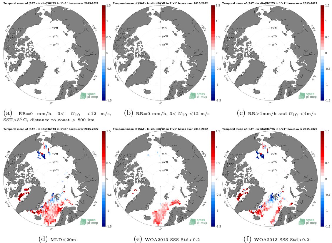
Figure 12: Temporal mean gridded over spatial boxes of size 1^{\circ}\times 1^{\circ} of \Delta\text{SSS} (SMAP SSS L3 v5 - Monthly (RSS) - Argo) for 6 different subdatasets corresponding to:RR=0 mm/h, 3 < U_{10} < 12 m/s, SST > 5^{\circ}\text{C} , distance to coast > 800 km (a), RR=0 mm/h, 3 < U_{10} < 12 m/s (b), RR > 1\text{mm/h} and U_{10} < 4\text{m/s} (c),MLD < 20\text{m} (d),WOA2013 SSS Std < 0.2 (e),WOA2013 SSS Std > 0.2 (f).
