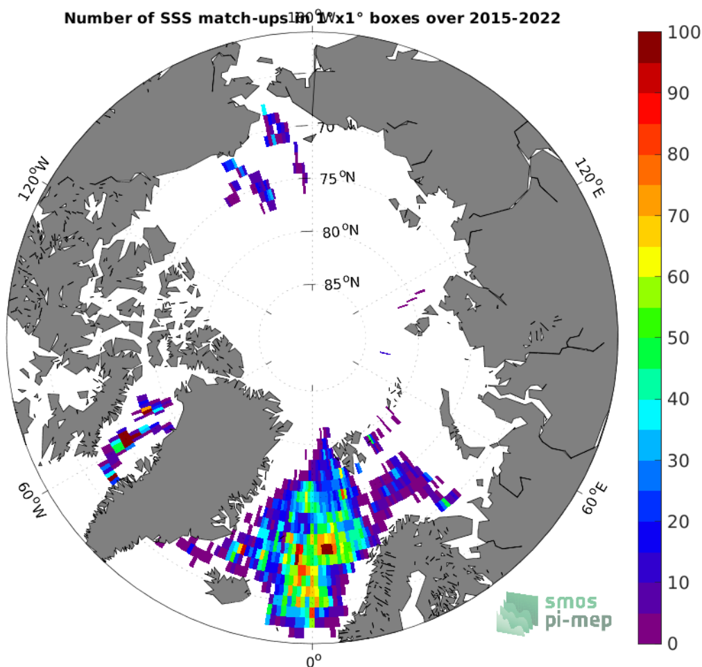
Figure 4: Number of SSS match-ups between Argo SSS and the SMAP SSS L3 v5 - Monthly (RSS) SSS product for the Arctic Ocean Pi-MEP region over 1^{\circ} \times 1^{\circ} boxes and for the full satellite product period.
