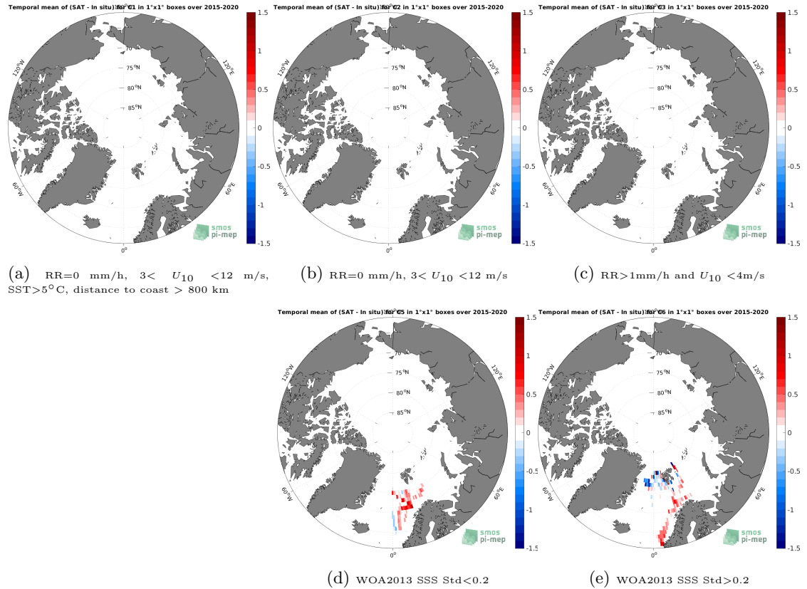
Figure 12: Temporal mean gridded over spatial boxes of size 1^{\circ}\times 1^{\circ} of \Delta\text{SSS} (SMAP SSS L3 v4 - 8-Day running (RSS) - TSG (Polarstern)) for 5 different subdatasets corresponding to:RR=0 mm/h, 3 < U_{10} < 12 m/s, \text{SST} > 5^{\circ}\text{C} , distance to coast > 800 km (a), RR=0 mm/h, 3 < U_{10} < 12 m/s (b), RR > 1 mm/h and U_{10} < 4 m/s (c), WOA2013 SSS Std < 0.2 (d), WOA2013 SSS Std > 0.2 (e).
