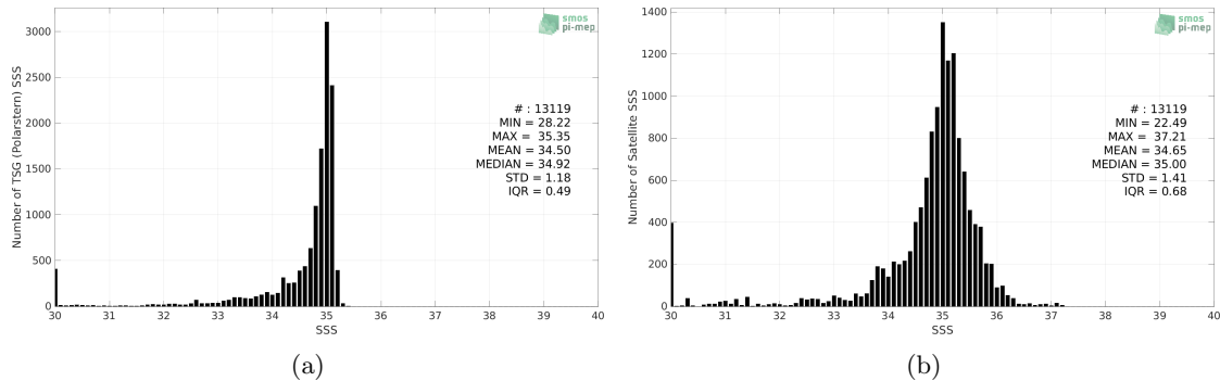
Figure 2: Histograms of SSS from TSG (Polarstern) (a) and SMAP SSS L3 v4 - 8-Day running (RSS) (b) considering all match-up pairs per bins of 0.1 over the Arctic Ocean Pi-MEP region and for the full satellite product period.
