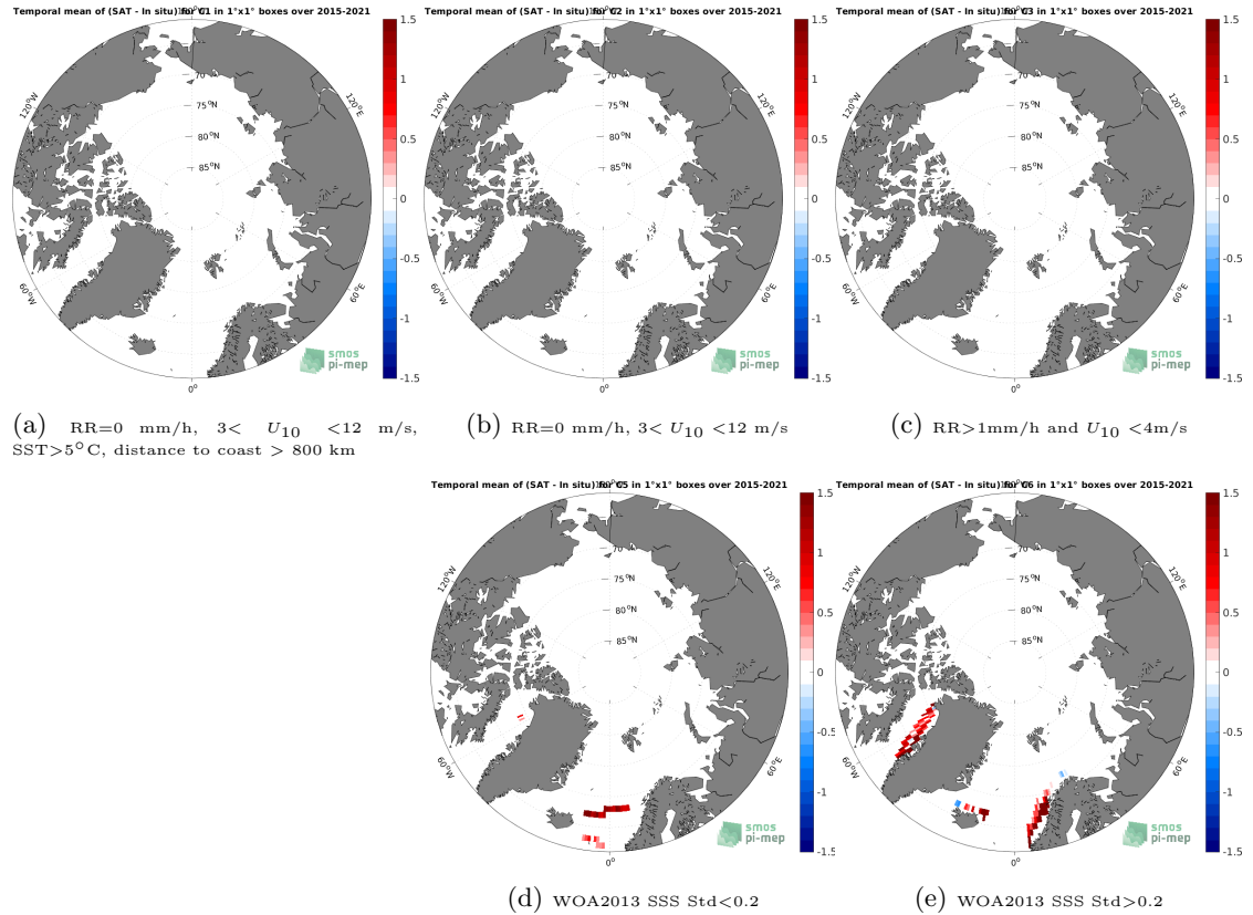
Figure 12: Temporal mean gridded over spatial boxes of size 1^{\circ}\times 1^{\circ} of \Delta\text{SSS} (SMAP SSS L3 v4 - 8-Day running (RSS) - TSG (LEGOS-DM)) for 5 different subdatasets corresponding to:RR=0 mm/h, 3 < U_{10} < 12 m/s, SST >5^{\circ}\text{C} , distance to coast > 800 km (a), RR=0 mm/h, 3 < U_{10} < 12 m/s (b), RR >1 mm/h and U_{10} < 4 m/s (c), WOA2013 SSS Std <0.2 (d), WOA2013 SSS Std >0.2 (e).
