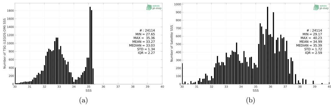
Figure 2: Histograms of SSS from TSG (LEGOS-DM) (a) and SMAP SSS L3 v4 - 8-Day running (RSS) (b) considering all match-up pairs per bins of 0.1 over the Arctic Ocean Pi-MEP region and for the full satellite product period.
