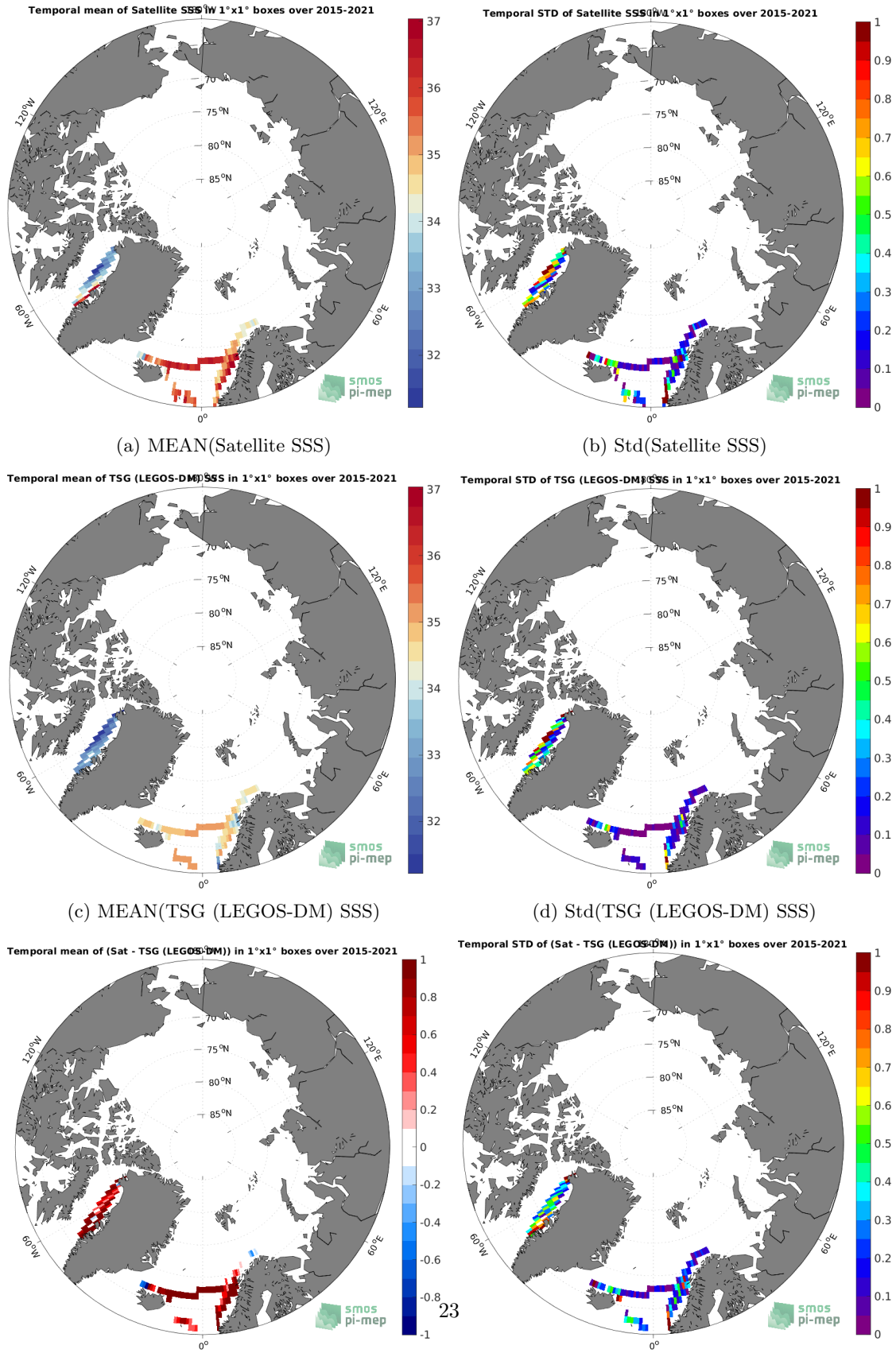
Figure 6: Temporal mean (left) and Std (right) of SSS from SMAP SSS L3 v4 - 8-Day running (RSS) (top), TSG (LEGOS-DM) (middle), and of \Delta SSS (Satellite - TSG (LEGOS-DM)). Only match-up pairs are used to generate these maps.
