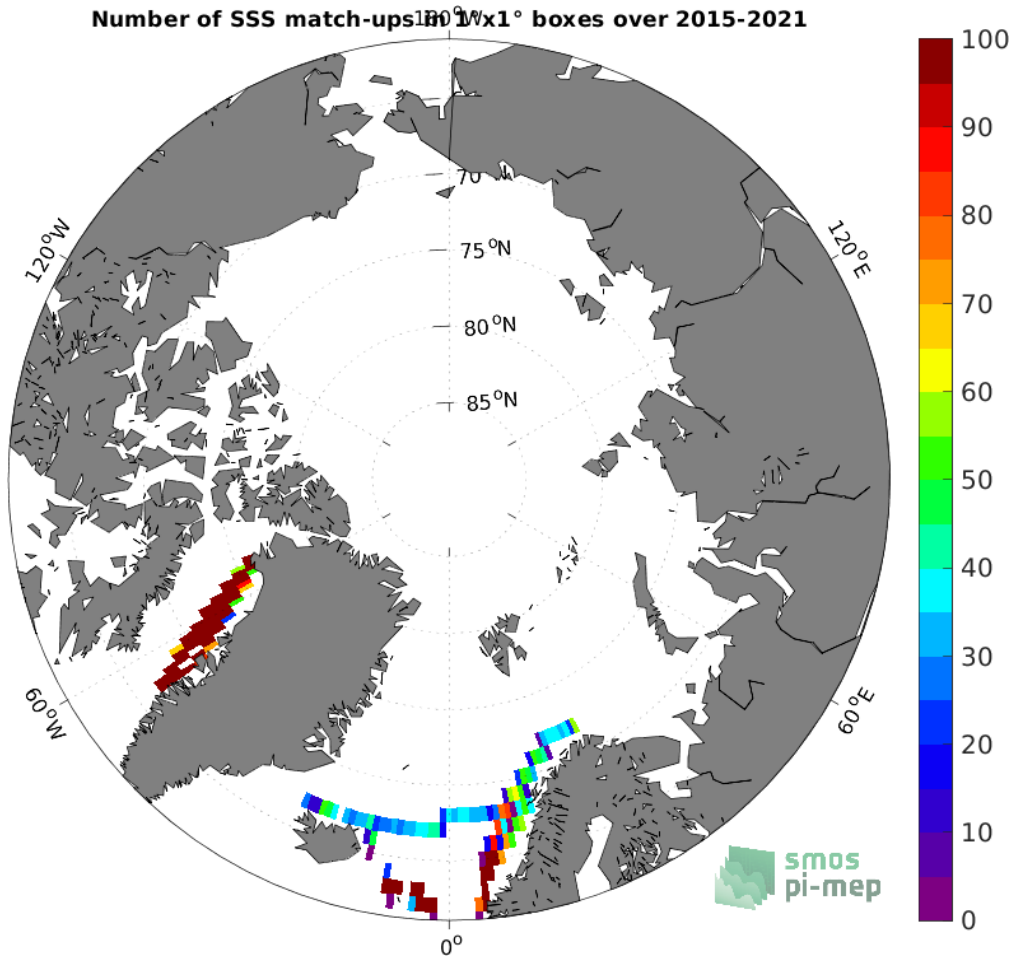
Figure 4: Number of SSS match-ups between TSG (LEGOS-DM) SSS and the SMAP SSS L3 v4 - 8-Day running (RSS) SSS product for the Arctic Ocean Pi-MEP region over 1^\circ \times 1^\circ boxes and for the full satellite product period.
