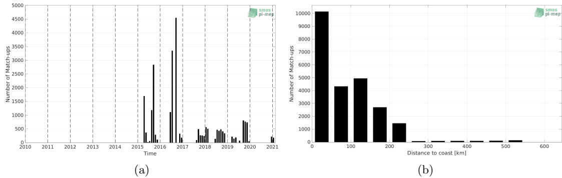
Figure 1: Number of match-ups between TSG (LEGOS-DM) and SMAP SSS L3 v4 - 8-Day running (RSS) SSS as a function of time (a) and as function of the distance to coast (b) over the Arctic Ocean Pi-MEP region and for the full satellite product period.
