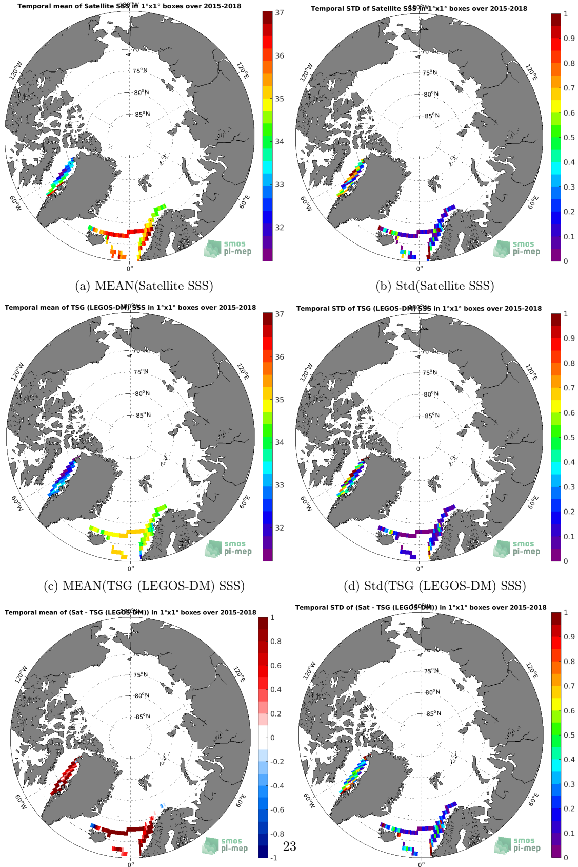
(e) MEAN( \Delta SSS) (Satellite - TSG (LEGOS-DM)) (f) Std( \Delta SSS) (Satellite - TSG (LEGOS-DM)) Figure 6: Temporal mean (left) and Std (right) of SSS from SMAP SSS L3 v4 - 8-Day running (RSS) (top), TSG (LEGOS-DM) (middle), and of \Delta SSS (Satellite - TSG (LEGOS-DM)). Only match-up pairs are used to generate these maps.
