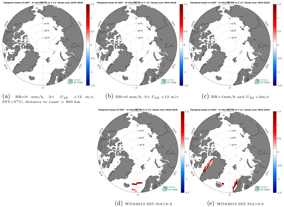
Figure 12: Temporal mean gridded over spatial boxes of size 1^{\circ}\times 1^{\circ} of \Delta\text{SSS} (SMAP-L3-RSS-V4-8DAY-RUNNING - TSG-LEGOS-DM) for 5 different subdatasets corresponding to:RR=0 mm/h, 3 < U_{10} < 12 m/s, SST > 5^{\circ}\text{C} , distance to coast > 800 km (a), RR=0 mm/h, 3 < U_{10} < 12 m/s (b), RR > 1 mm/h and U_{10} < 4 m/s (c), WOA2013 SSS Std < 0.2 (d), WOA2013 SSS Std > 0.2 (e).
