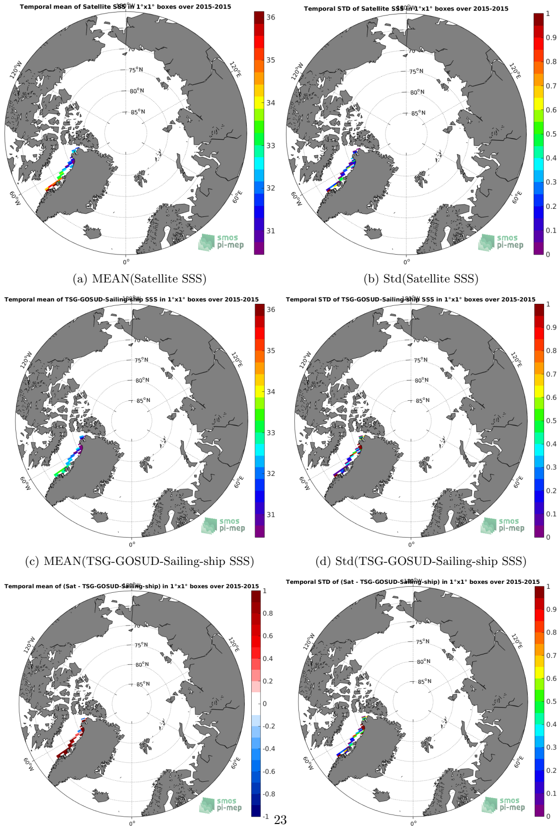
Figure 6: Temporal mean (left) and Std (right) of SSS from SMAP-L3-RSS-V4-8DAY-RUNNING (top), TSG-GOSUD-Sailing-ship (middle), and of \Delta SSS (Satellite - TSG-GOSUD-Sailing-ship). Only match-up pairs are used to generate these maps.
