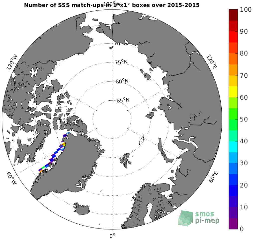
Figure 4: Number of SSS match-ups between TSG-GOSUD-Sailing-ship SSS and the SMAP-L3-RSS-V4-8DAY-RUNNING SSS product for the Arctic Ocean Pi-MEP region over 1^{\circ} \times 1^{\circ} boxes and for the full satellite product period.
