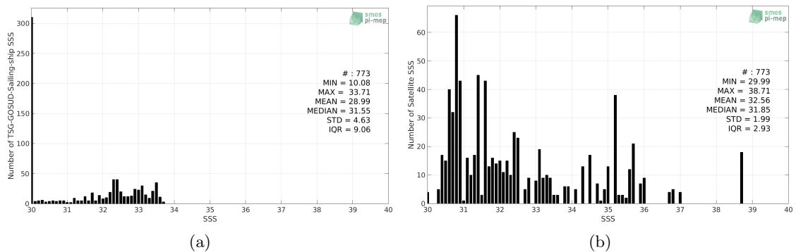
Figure 2: Histograms of SSS from TSG-GOSUD-Sailing-ship (a) and SMAP-L3-RSS-V4-8DAY-RUNNING (b) considering all match-up pairs per bins of 0.1 over the Arctic Ocean Pi-MEP region and for the full satellite product period.
