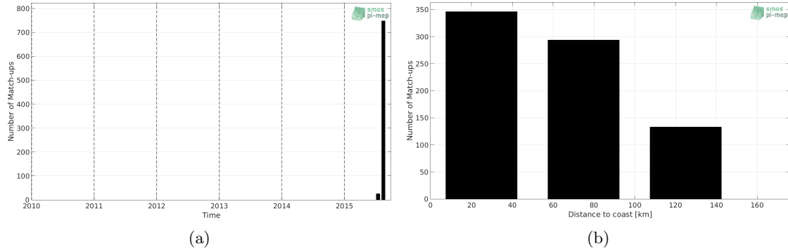
Figure 1: Number of match-ups between TSG-GOSUD-Sailing-ship and SMAP-L3-RSS-V4-8DAY-RUNNING SSS as a function of time (a) and as function of the distance to coast (b) over the Arctic Ocean Pi-MEP region and for the full satellite product period.
