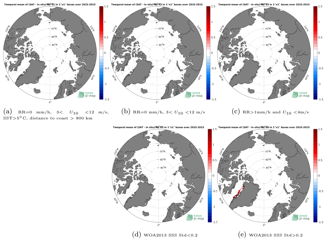
Figure 12: Temporal mean gridded over spatial boxes of size 1^\circ \times 1^\circ of \Delta SSS (SMAP-L3-RSS-V4-8DAY-RUNNING - TSG-GOSUD-Sailing-ship) for 5 different subdatasets corresponding to:RR=0 mm/h, 3 < U_{10} < 12 m/s, SST>5°C, distance to coast > 800 km (a), RR=0 mm/h, 3 < U_{10} < 12 m/s (b), RR>1mm/h and U_{10} < 4 m/s (c), WOA2013 SSS Std<0.2 (d), WOA2013 SSS Std>0.2 (e).
