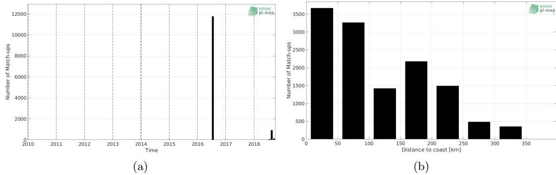
Figure 1: Number of match-ups between TSG (GOSUD-Research-vessel) and SMAP SSS L3 v4 - 8-Day running (RSS) SSS as a function of time (a) and as function of the distance to coast (b) over the Arctic Ocean Pi-MEP region and for the full satellite product period.
