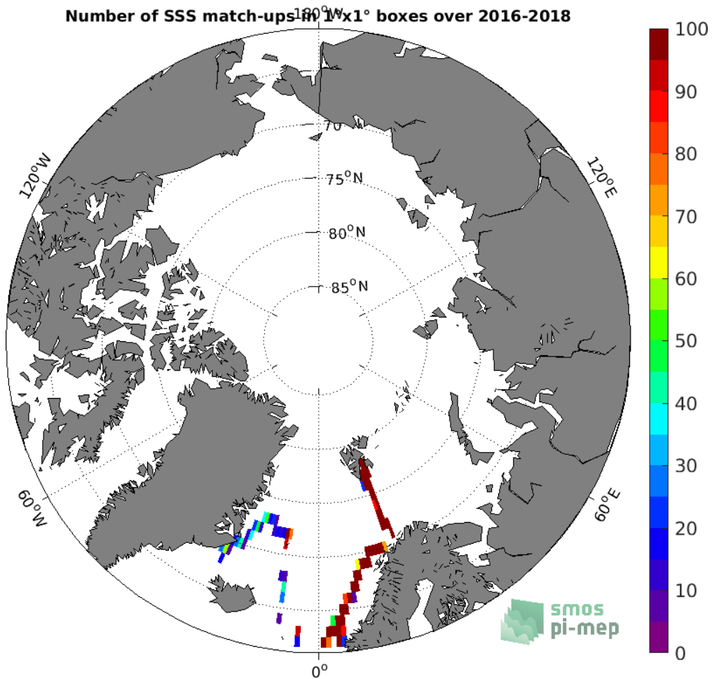
Figure 4: Number of SSS match-ups between TSG (GOSUD-Research-vessel) SSS and the SMAP SSS L3 v4 - 8-Day running (RSS) SSS product for the Arctic Ocean Pi-MEP region over 1^\circ \times 1^\circ boxes and for the full satellite product period.
