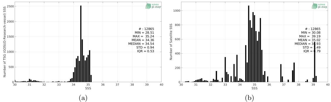
Figure 2: Histograms of SSS from TSG (GOSUD-Research-vessel) (a) and SMAP SSS L3 v4 - 8-Day running (RSS) (b) considering all match-up pairs per bins of 0.1 over the Arctic Ocean Pi-MEP region and for the full satellite product period.
