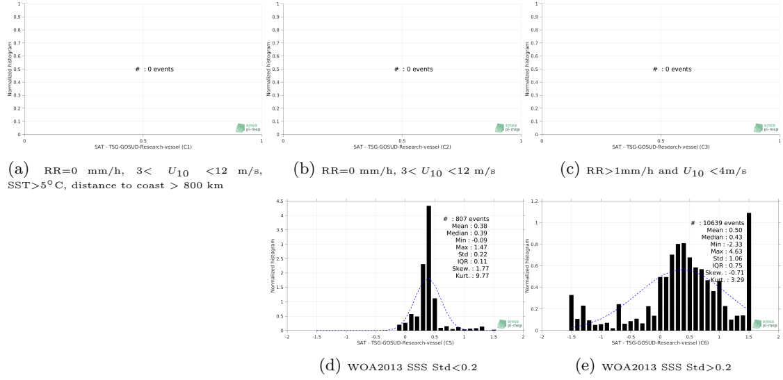
Figure 13: Normalized histogram of \Delta SSS (SMAP-L3-RSS-V4-8DAY-RUNNING - TSG-GOSUD-Research-vessel) for 5 different subdatasets corresponding to: RR=0 mm/h, 3 < U_{10} < 12 m/s, SST>5°C, distance to coast > 800 km (a), RR=0 mm/h, 3 < U_{10} < 12 m/s (b), RR>1mm/h and U_{10} < 4 m/s (c), WOA2013 SSS Std<0.2 (d), WOA2013 SSS Std>0.2 (e).
