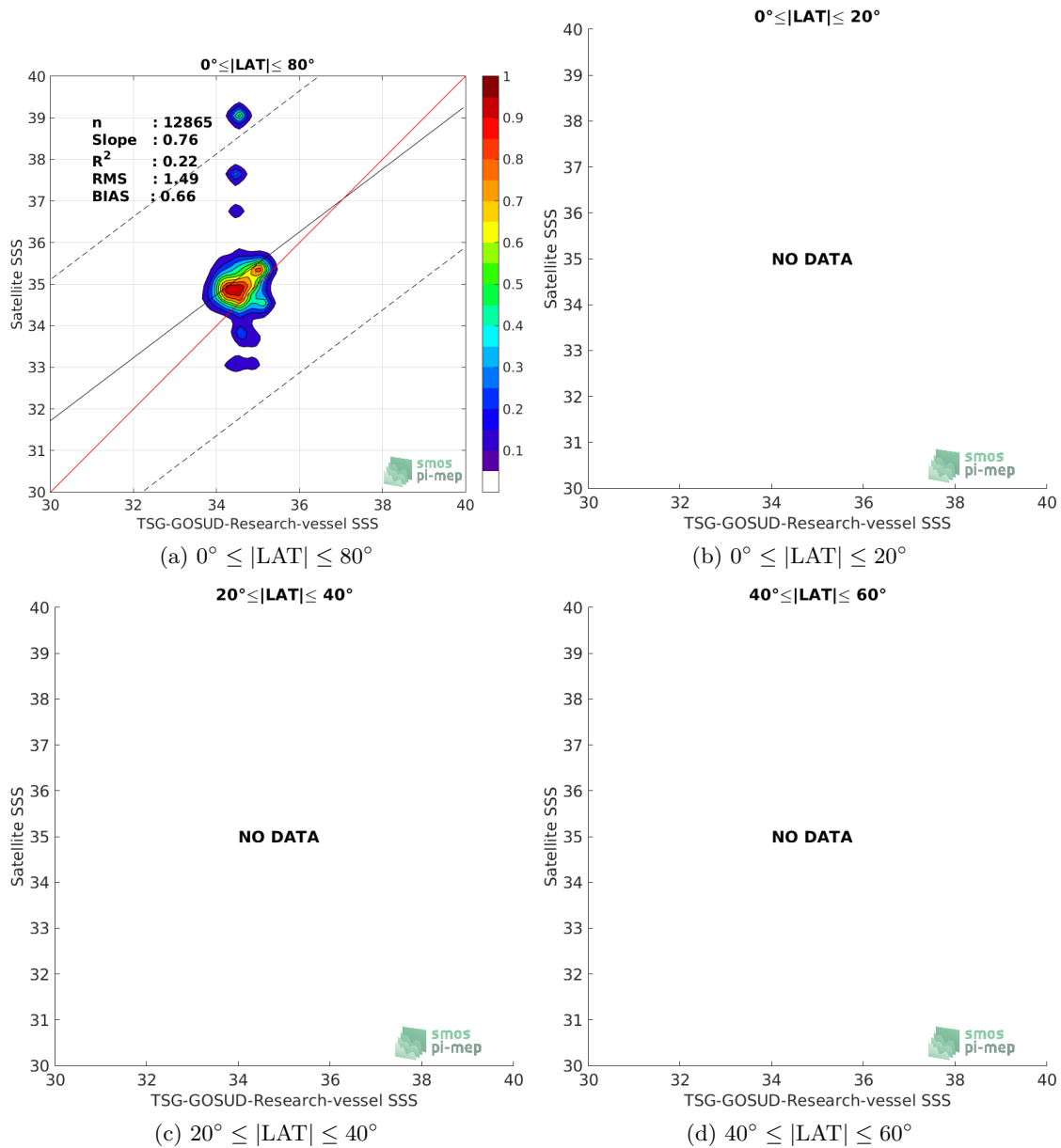
Figure 9: Contour maps of the concentration of SMAP-L3-RSS-V4-8DAY-RUNNING SSS (y-axis) versus TSG-GOSUD-Research-vessel SSS (x-axis) at match-up pairs for different latitude bands. For each plot, the red line shows x=y . The black thin and dashed lines indicate a linear fit through the data cloud and the \pm 95\% confidence levels, respectively. The number match-up pairs n , the slope and R^2 coefficient of the linear fit, the root mean square (RMS) and the mean bias between satellite and in situ data are indicated for each latitude band in each plots.
