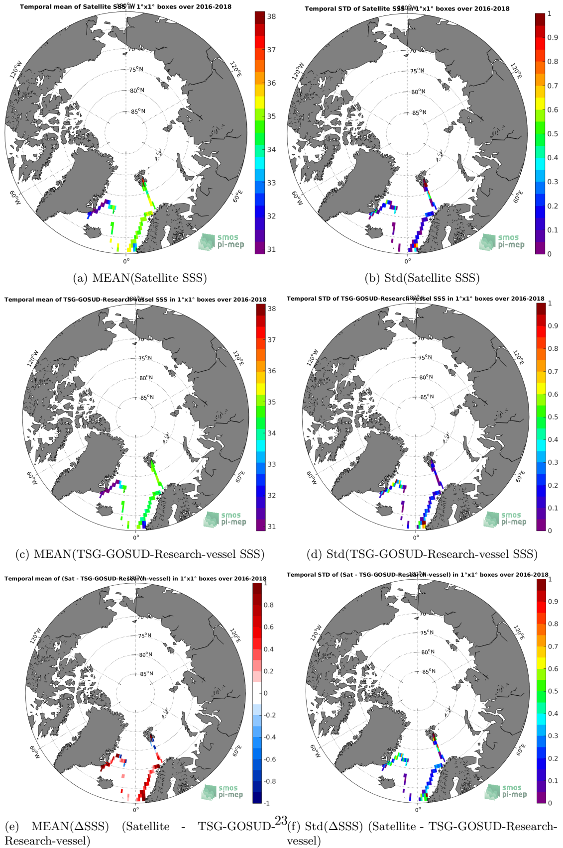
Figure 6: Temporal mean (left) and Std (right) of SSS from SMAP-L3-RSS-V4-8DAY-RUNNING (top), TSG-GOSUD-Research-vessel (middle), and of \Delta SSS (Satellite - TSG-GOSUD-Research-vessel). Only match-up pairs are used to generate these maps.
