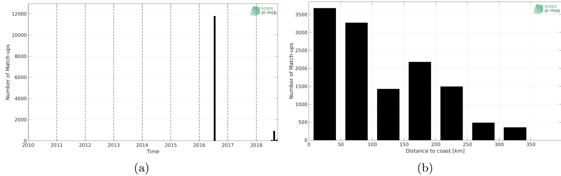
Figure 1: Number of match-ups between TSG-GOSUD-Research-vessel and SMAP-L3-RSS-V4-8DAY-RUNNING SSS as a function of time (a) and as function of the distance to coast (b) over the Arctic Ocean Pi-MEP region and for the full satellite product period.
