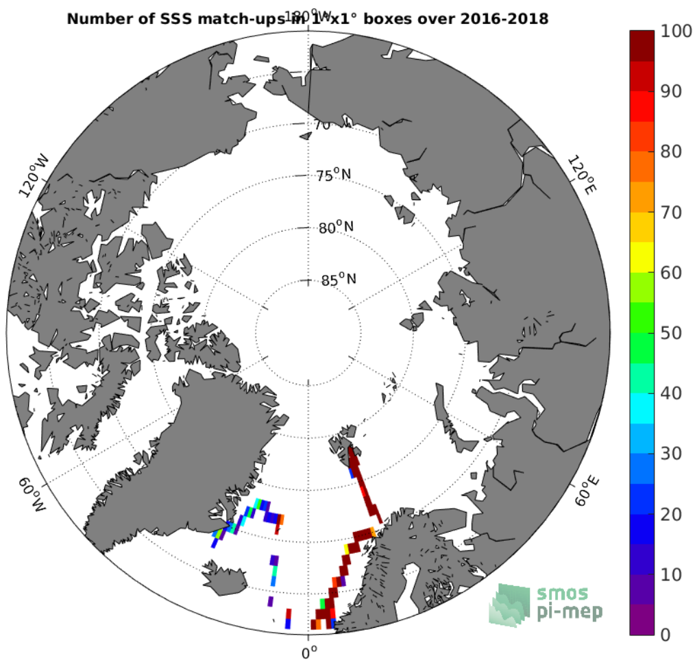
Figure 4: Number of SSS match-ups between TSG-GOSUD-Research-vessel SSS and the SMAP-L3-RSS-V4-8DAY-RUNNING SSS product for the Arctic Ocean Pi-MEP region over 1°x1° boxes and for the full satellite product period.
