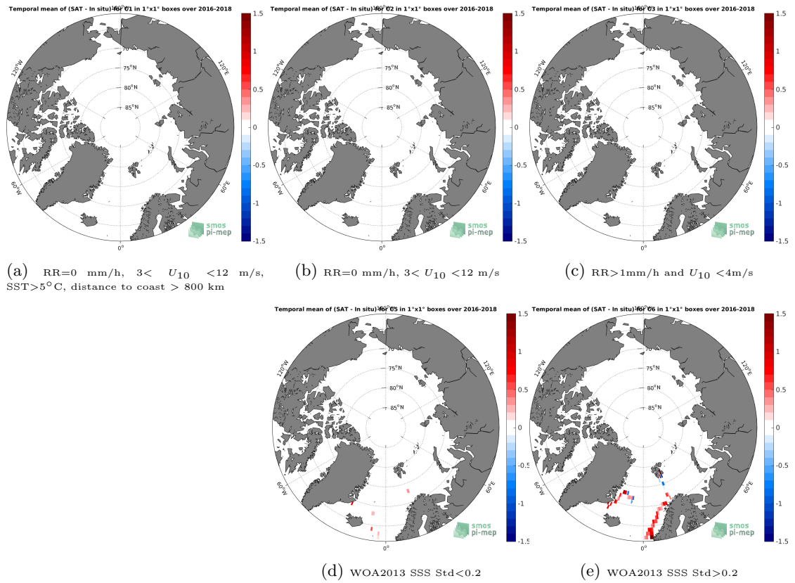
Figure 12: Temporal mean gridded over spatial boxes of size 1°x1° of \Delta SSS (SMAP-L3-RSS-V4-8DAY-RUNNING - TSG-GOSUD-Research-vessel) for 5 different subdatasets corresponding to:RR=0 mm/h, 3 < U_{10} < 12 m/s, SST>5°C, distance to coast > 800 km (a), RR=0 mm/h, 3 < U_{10} < 12 m/s (b), RR>1mm/h and U_{10} < 4 m/s (c), WOA2013 SSS Std<0.2 (d), WOA2013 SSS Std>0.2 (e).
