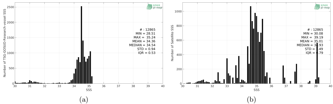
Figure 2: Histograms of SSS from TSG-GOSUD-Research-vessel (a) and SMAP-L3-RSS-V4-8DAY-RUNNING (b) considering all match-up pairs per bins of 0.1 over the Arctic Ocean Pi-MEP region and for the full satellite product period.
