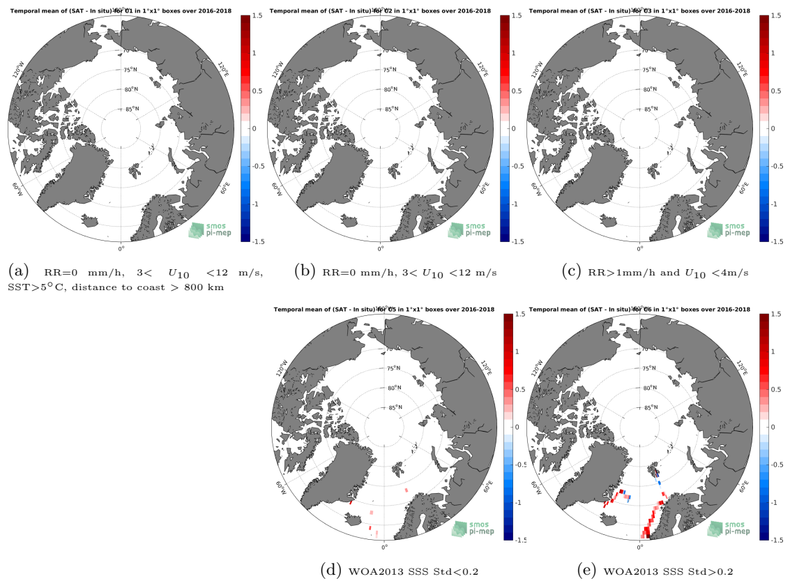
Figure 12: Temporal mean gridded over spatial boxes of size 1^\circ \times 1^\circ of \Delta SSS (SMAP-L3-RSS-V4-8DAY-RUNNING - TSG-GOSUD-Research-vessel) for 5 different subdatasets corresponding to:RR=0 mm/h, 3 < U_{10} < 12 m/s, SST>5°C, distance to coast > 800 km (a), RR=0 mm/h, 3 < U_{10} < 12 m/s (b), RR>1mm/h and U_{10} < 4 m/s (c), WOA2013 SSS Std<0.2 (d), WOA2013 SSS Std>0.2 (e).
