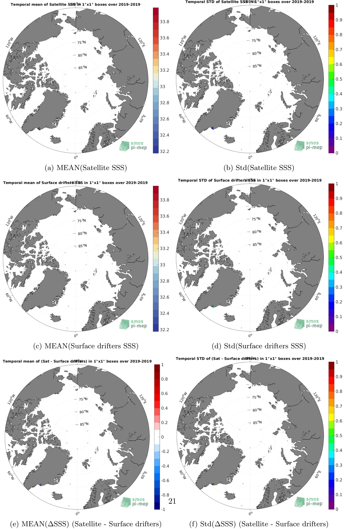
Figure 5: Temporal mean (left) and Std (right) of SSS from SMAP SSS L3 v4 - 8-Day running (RSS) (top), Surface drifters (middle), and of \Delta SSS (Satellite - Surface drifters). Only match-up pairs are used to generate these maps.
