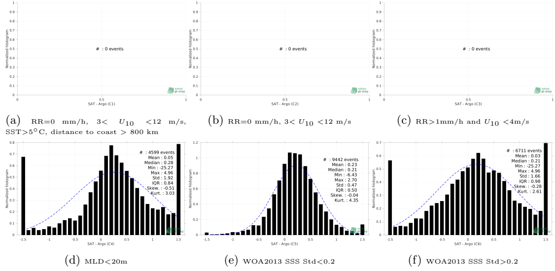
Figure 13: Normalized histogram of \Delta\text{SSS} (SMAP SSS L3 v4 - 8-Day running (RSS) - Argo) for 6 different subdatasets corresponding to: RR=0 mm/h, 3 < U_{10} < 12 m/s, SST > 5^{\circ}\text{C} , distance to coast > 800 km (a), RR=0 mm/h, 3 < U_{10} < 12 m/s (b), RR > 1\text{mm/h} and U_{10} < 4\text{m/s} (c), MLD < 20\text{m} (d), WOA2013 SSS Std < 0.2 (e), WOA2013 SSS Std > 0.2 (f).
