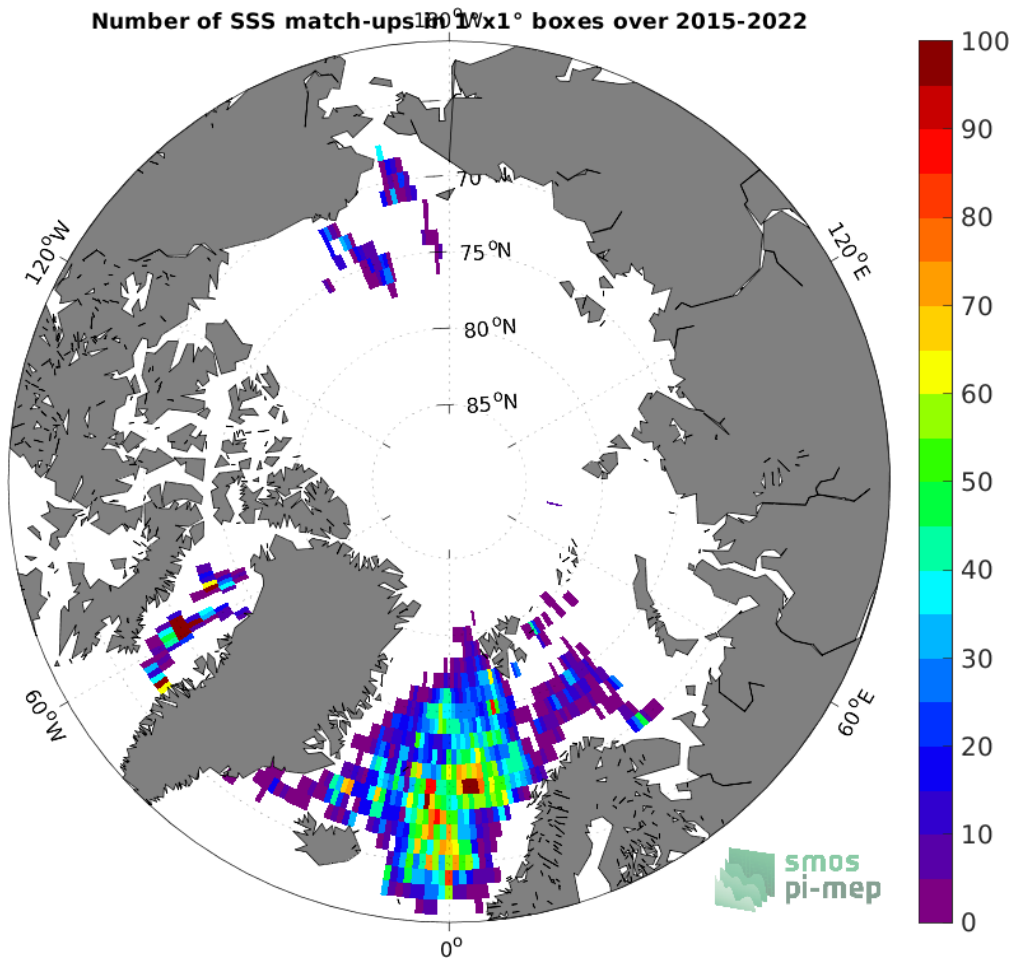
Figure 4: Number of SSS match-ups between Argo SSS and the SMAP SSS L3 v4 - 8-Day running (RSS) SSS product for the Arctic Ocean Pi-MEP region over 1^{\circ} \times 1^{\circ} boxes and for the full satellite product period.
