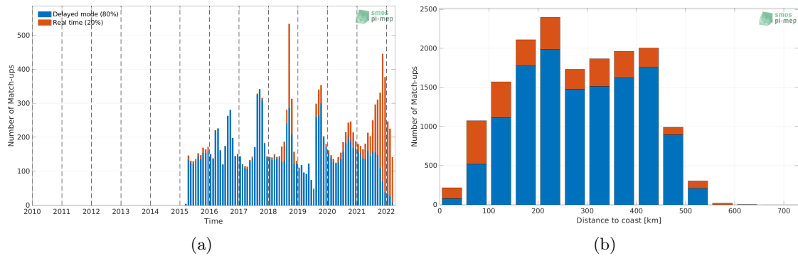
Figure 1: Number of match-ups between Argo and SMAP SSS L3 v4 - 8-Day running (RSS) SSS as a function of time (a) and as function of the distance to coast (b) over the Arctic Ocean Pi-MEP region and for the full satellite product period.
