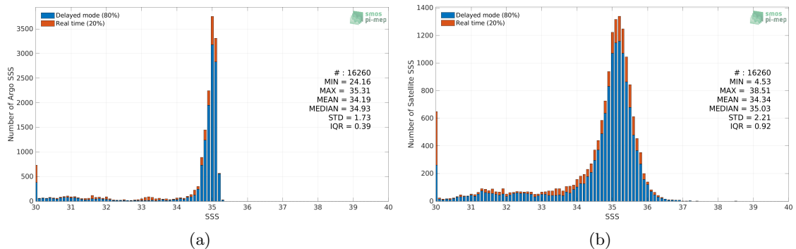
Figure 2: Histograms of SSS from Argo (a) and SMAP SSS L3 v4 - 8-Day running (RSS) (b) considering all match-up pairs per bins of 0.1 over the Arctic Ocean Pi-MEP region and for the full satellite product period.
