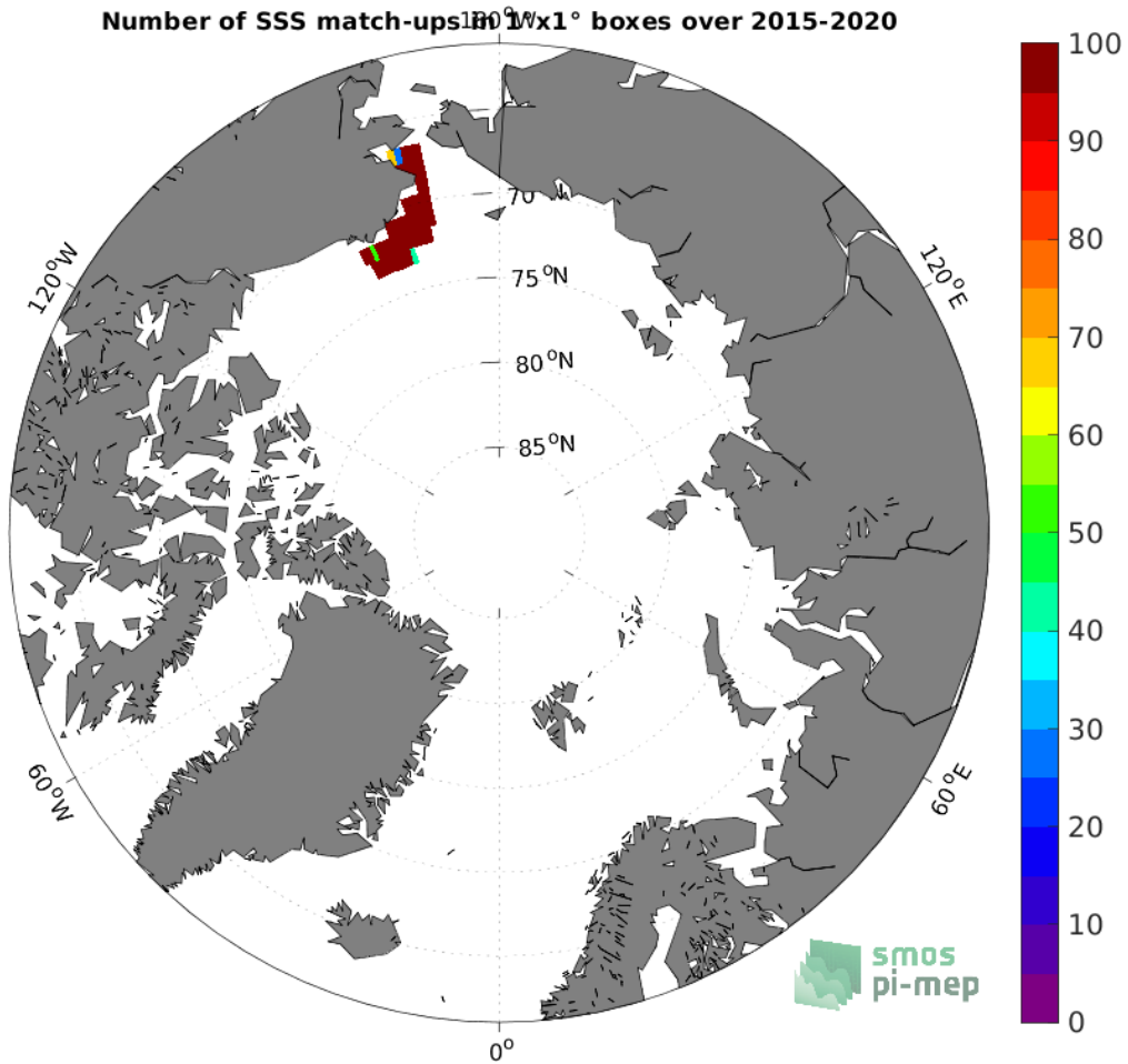
Figure 4: Number of SSS match-ups between TSG (SAMOS) SSS and the SMAP SSS L3 v4 - Monthly (RSS) SSS product for the Arctic Ocean Pi-MEP region over 1^\circ \times 1^\circ boxes and for the full satellite product period.
