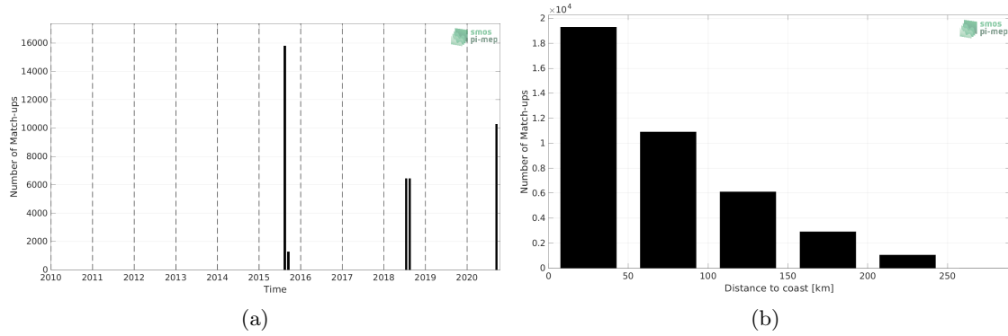
Figure 1: Number of match-ups between TSG (SAMOS) and SMAP SSS L3 v4 - Monthly (RSS) SSS as a function of time (a) and as function of the distance to coast (b) over the Arctic Ocean Pi-MEP region and for the full satellite product period.
