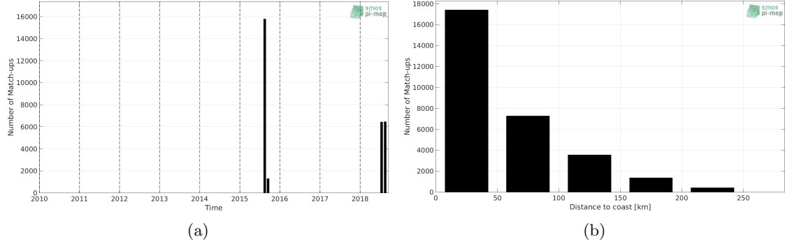
Figure 1: Number of match-ups between TSG-SAMOS and SMAP-L3-RSS-V4-MONTHLY SSS as a function of time (a) and as function of the distance to coast (b) over the Arctic Ocean Pi-MEP region and for the full satellite product period.
