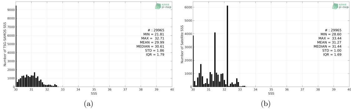
Figure 2: Histograms of SSS from TSG-SAMOS (a) and SMAP-L3-RSS-V4-MONTHLY (b) considering all match-up pairs per bins of 0.1 over the Arctic Ocean Pi-MEP region and for the full satellite product period.
