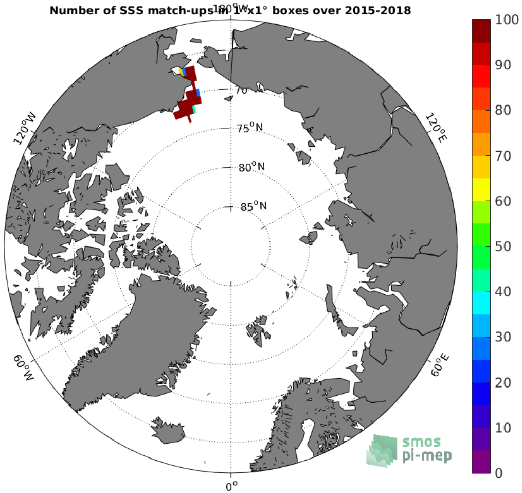
Figure 4: Number of SSS match-ups between TSG-SAMOS SSS and the SMAP-L3-RSS-V4-MONTHLY SSS product for the Arctic Ocean Pi-MEP region over 1°x1° boxes and for the full satellite product period.
