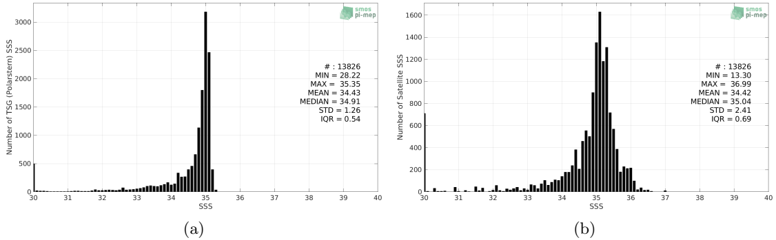
Figure 2: Histograms of SSS from TSG (Polarstern) (a) and SMAP SSS L3 v4 - Monthly (RSS) (b) considering all match-up pairs per bins of 0.1 over the Arctic Ocean Pi-MEP region and for the full satellite product period.
