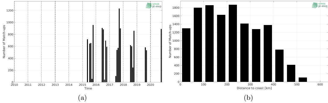
Figure 1: Number of match-ups between TSG (Polarstern) and SMAP SSS L3 v4 - Monthly (RSS) SSS as a function of time (a) and as function of the distance to coast (b) over the Arctic Ocean Pi-MEP region and for the full satellite product period.
