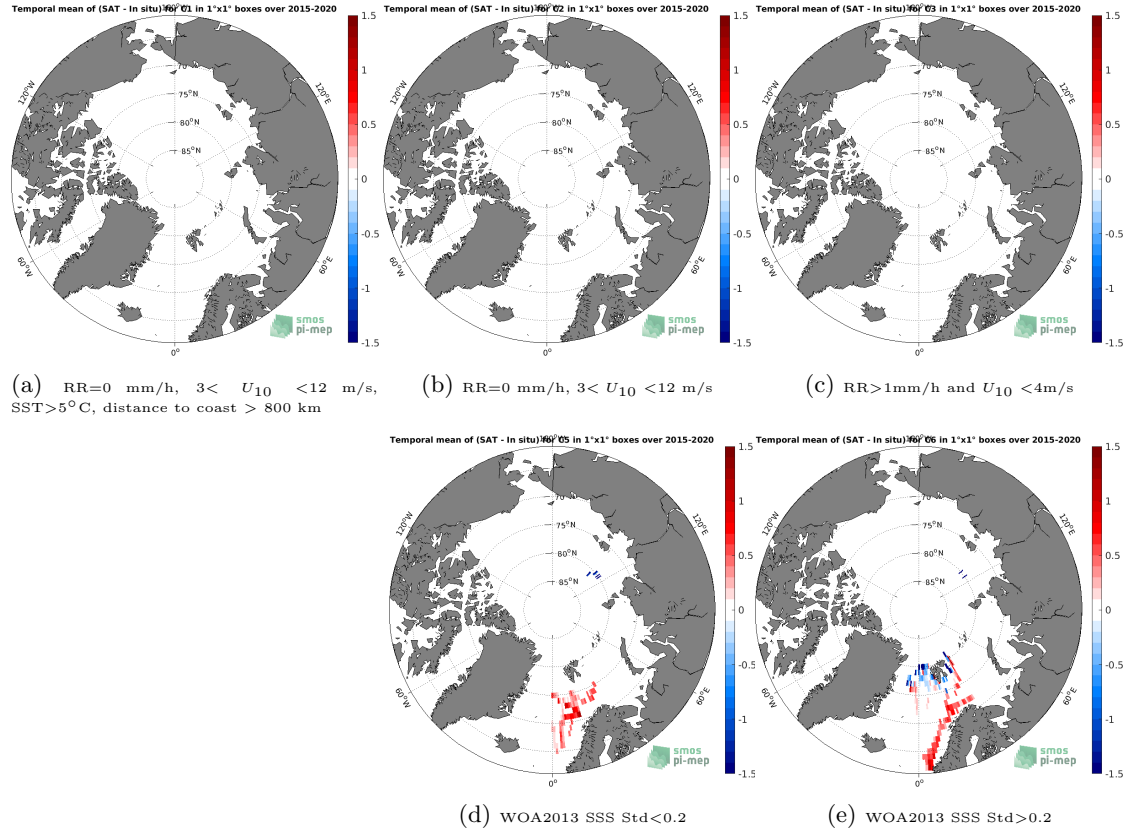
Figure 12: Temporal mean gridded over spatial boxes of size 1^{\circ}\times 1^{\circ} of \Delta\text{SSS} (SMAP SSS L3 v4 - Monthly (RSS) - TSG (Polarstern)) for 5 different subdatasets corresponding to:RR=0 mm/h, 3 < U_{10} < 12 m/s, SST >5^{\circ}\text{C} , distance to coast > 800 km (a), RR=0 mm/h, 3 < U_{10} < 12 m/s (b), RR >1 mm/h and U_{10} < 4 m/s (c), WOA2013 SSS Std <0.2 (d), WOA2013 SSS Std >0.2 (e).
