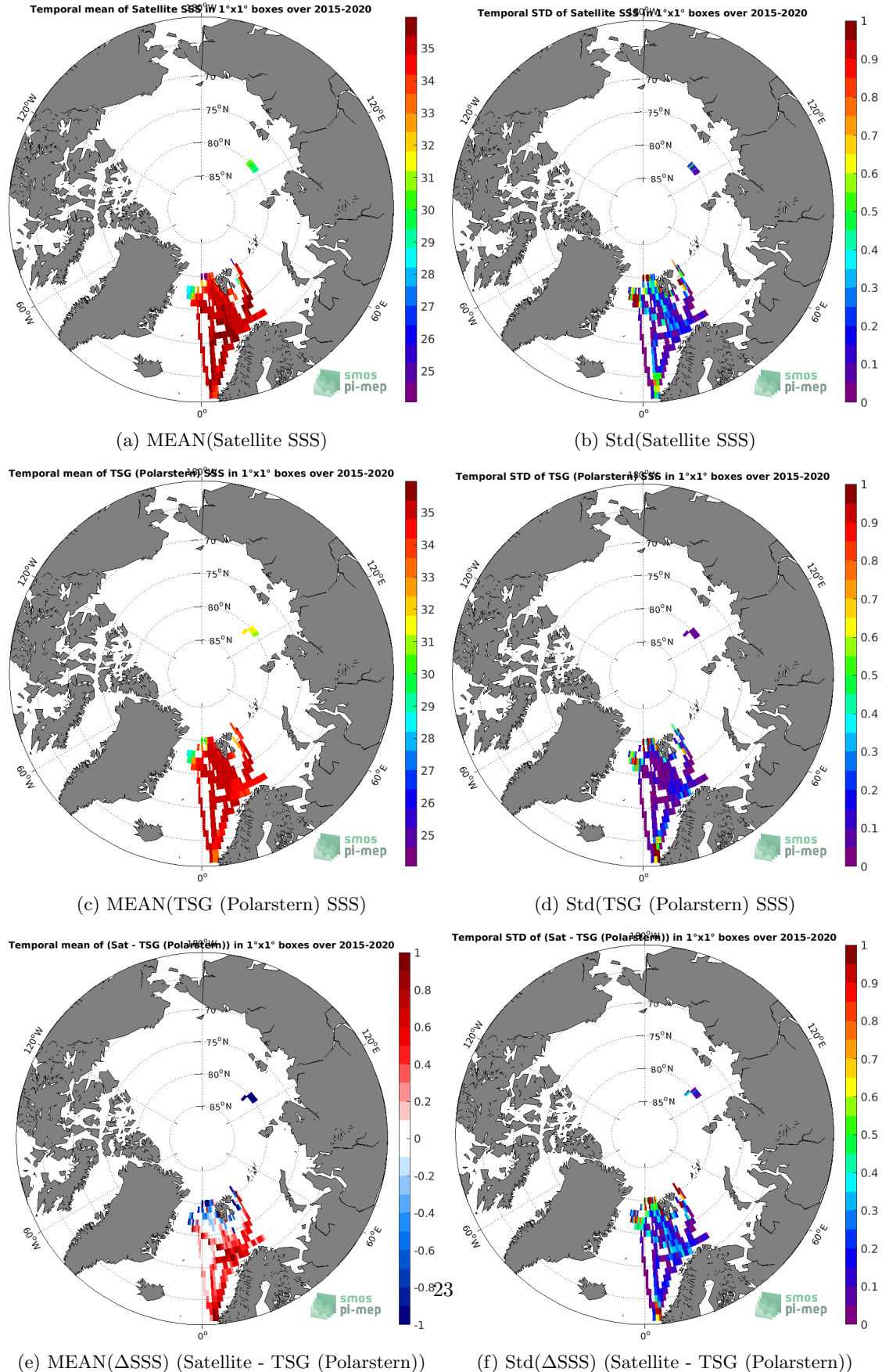
Figure 6: Temporal mean (left) and Std (right) of SSS from SMAP SSS L3 v4 - Monthly (RSS) (top), TSG (Polarstern) (middle), and of \Delta SSS (Satellite - TSG (Polarstern)). Only match-up pairs are used to generate these maps.
