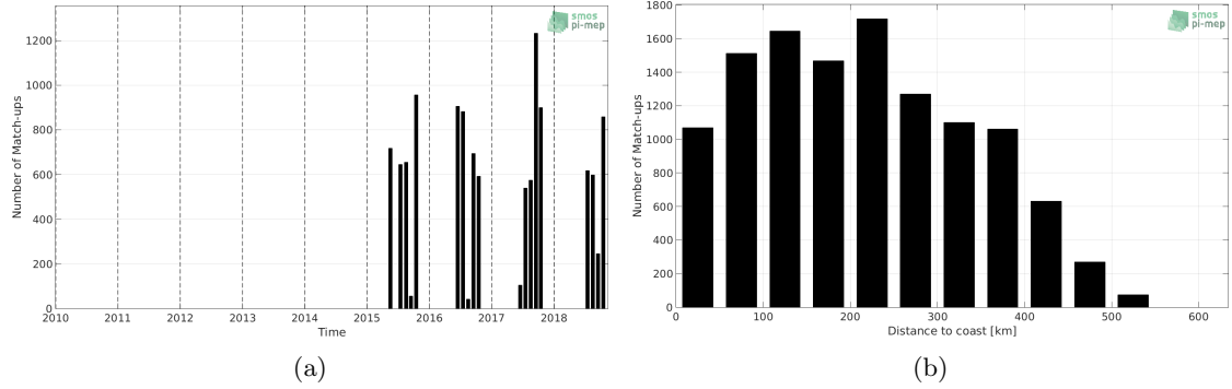
Figure 1: Number of match-ups between TSG-POLARSTERN and SMAP-L3-RSS-V4-MONTHLY SSS as a function of time (a) and as function of the distance to coast (b) over the Arctic Ocean Pi-MEP region and for the full satellite product period.
