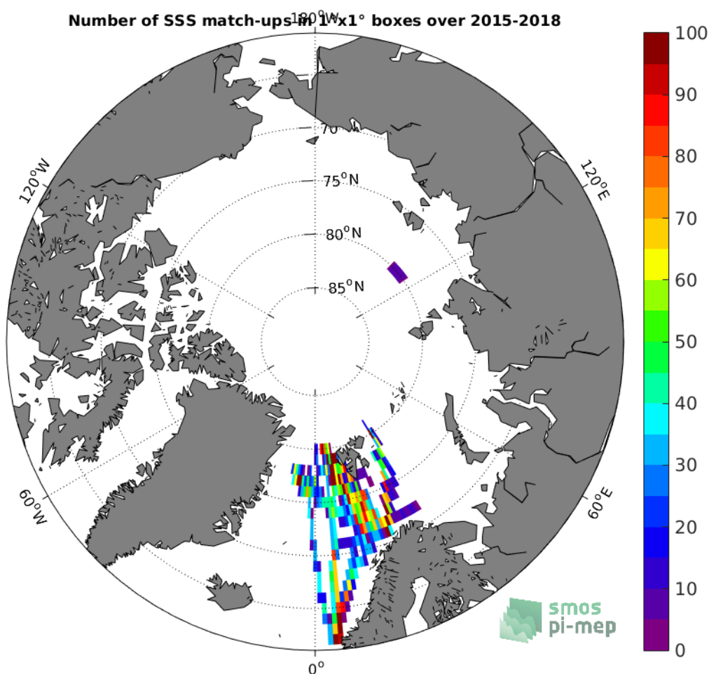
Figure 4: Number of SSS match-ups between TSG-POLARSTERN SSS and the SMAP-L3-RSS-V4-MONTHLY SSS product for the Arctic Ocean Pi-MEP region over 1°x1° boxes and for the full satellite product period.
