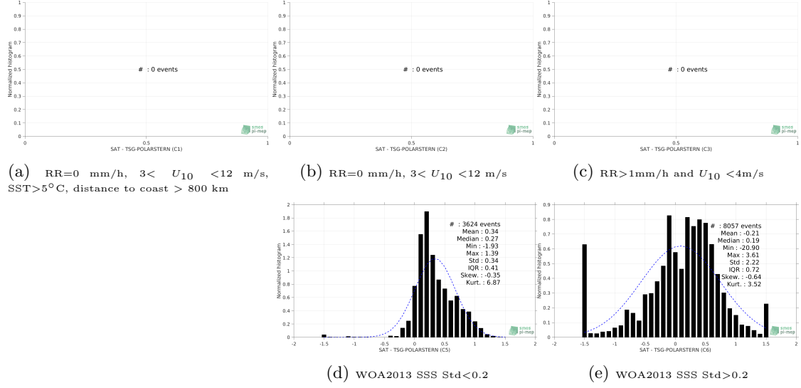
Figure 13: Normalized histogram of \Delta\text{SSS} (SMAP-L3-RSS-V4-MONTHLY - TSG-POLARSTERN) for 5 different subdatasets corresponding to: RR=0 mm/h, 3 < U_{10} < 12 m/s, SST > 5^{\circ}\text{C} , distance to coast > 800 km (a), RR=0 mm/h, 3 < U_{10} < 12 m/s (b), RR > 1\text{mm/h} and U_{10} < 4\text{m/s} (c), WOA2013 SSS Std < 0.2 (d), WOA2013 SSS Std > 0.2 (e).
