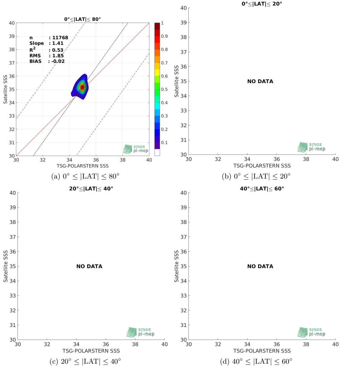
Figure 9: Contour maps of the concentration of SMAP-L3-RSS-V4-MONTHLY SSS (y-axis) versus TSG-POLARSTERN SSS (x-axis) at match-up pairs for different latitude bands. For each plot, the red line shows x=y . The black thin and dashed lines indicate a linear fit through the data cloud and the \pm 95\% confidence levels, respectively. The number match-up pairs n , the slope and R^2 coefficient of the linear fit, the root mean square (RMS) and the mean bias between satellite and in situ data are indicated for each latitude band in each plots.
