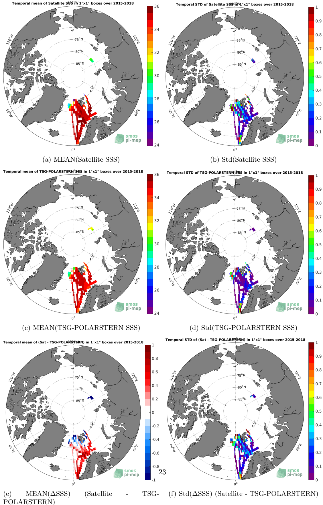
Figure 6: Temporal mean (left) and Std (right) of SSS from SMAP-L3-RSS-V4-MONTHLY (top), TSG-POLARSTERN (middle), and of \Delta SSS (Satellite - TSG-POLARSTERN). Only match-up pairs are used to generate these maps.
