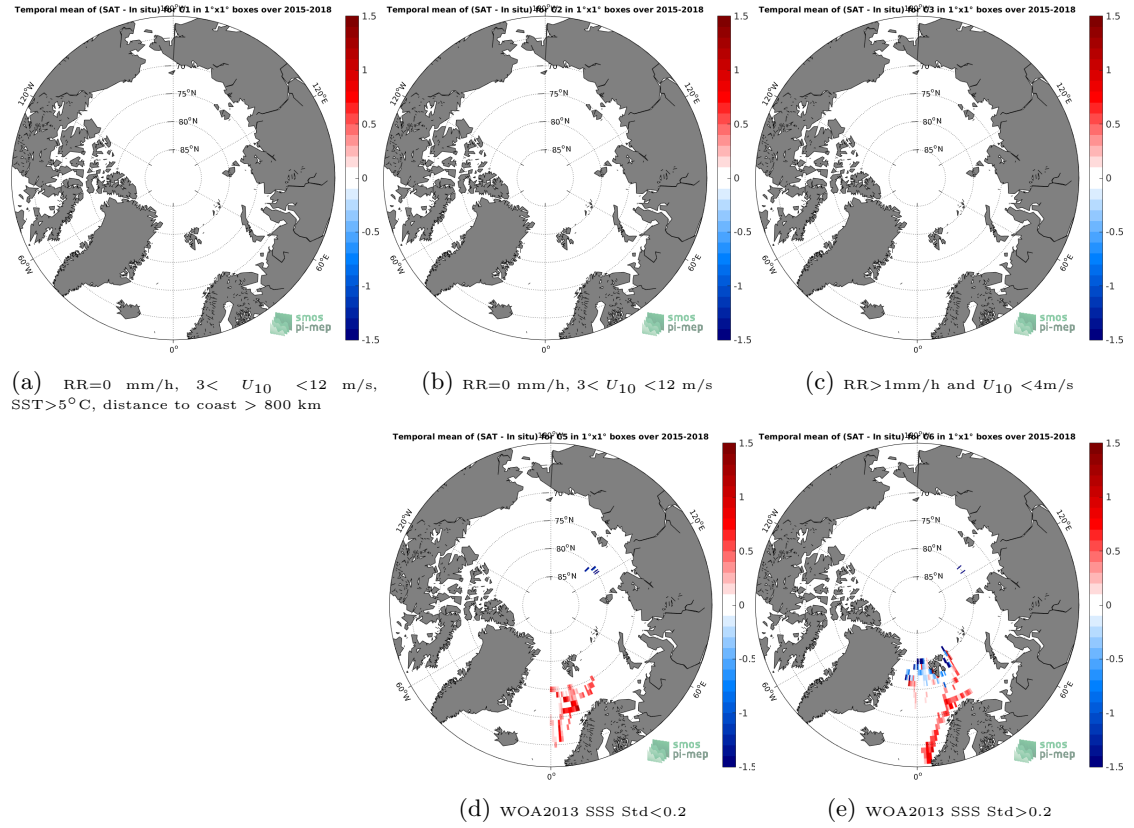
Figure 12: Temporal mean gridded over spatial boxes of size 1^\circ \times 1^\circ of \Delta SSS (SMAP-L3-RSS-V4-MONTHLY - TSG-POLARSTERN) for 5 different subdatasets corresponding to: RR=0 mm/h, 3 < U_{10} < 12 m/s, SST > 5^\circ C , distance to coast > 800 km (a), RR=0 mm/h, 3 < U_{10} < 12 m/s (b), RR > 1 mm/h and U_{10} < 4 m/s (c), WOA2013 SSS Std < 0.2 (d), WOA2013 SSS Std > 0.2 (e).
