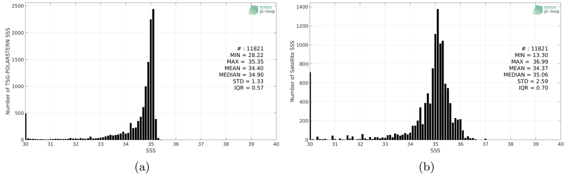
Figure 2: Histograms of SSS from TSG-POLARSTERN (a) and SMAP-L3-RSS-V4-MONTHLY (b) considering all match-up pairs per bins of 0.1 over the Arctic Ocean Pi-MEP region and for the full satellite product period.
