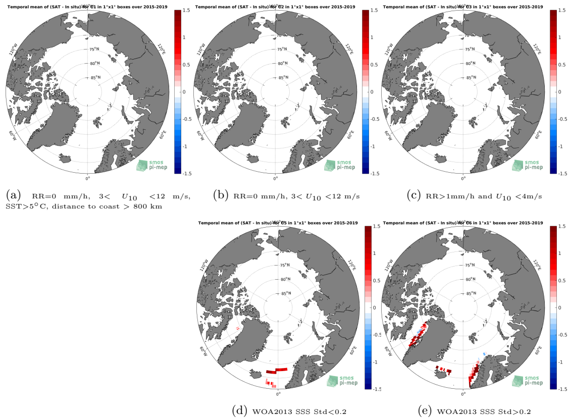
Figure 12: Temporal mean gridded over spatial boxes of size 1^{\circ}\times 1^{\circ} of \Delta\text{SSS} (SMAP SSS L3 v4 - Monthly (RSS) - TSG (LEGOS-DM)) for 5 different subdatasets corresponding to:RR=0 mm/h, 3 < U_{10} < 12 m/s, \text{SST} > 5^{\circ}\text{C} , distance to coast > 800 km (a), RR=0 mm/h, 3 < U_{10} < 12 m/s (b), RR > 1 mm/h and U_{10} < 4 m/s (c), WOA2013 SSS Std < 0.2 (d), WOA2013 SSS Std > 0.2 (e).
