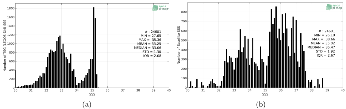
Figure 2: Histograms of SSS from TSG (LEGOS-DM) (a) and SMAP SSS L3 v4 - Monthly (RSS) (b) considering all match-up pairs per bins of 0.1 over the Arctic Ocean Pi-MEP region and for the full satellite product period.
