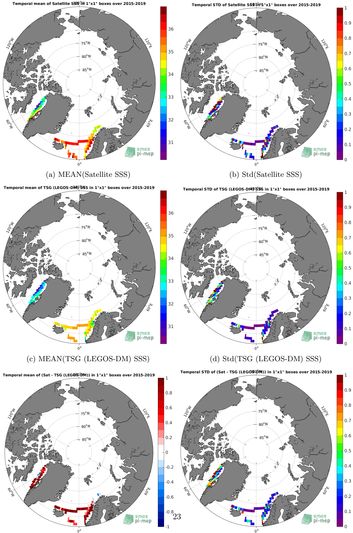
Figure 6: Temporal mean (left) and Std (right) of SSS from SMAP SSS L3 v4 - Monthly (RSS) (top), TSG (LEGOS-DM) (middle), and of \Delta SSS (Satellite - TSG (LEGOS-DM)). Only match-pairs are used to generate these maps.
