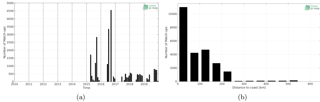
Figure 1: Number of match-ups between TSG (LEGOS-DM) and SMAP SSS L3 v4 - Monthly (RSS) SSS as a function of time (a) and as function of the distance to coast (b) over the Arctic Ocean Pi-MEP region and for the full satellite product period.
