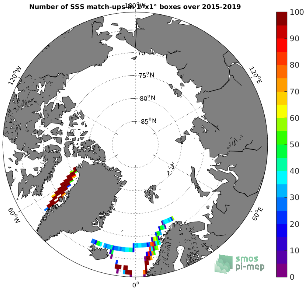
Figure 4: Number of SSS match-ups between TSG (LEGOS-DM) SSS and the SMAP SSS L3 v4 - Monthly (RSS) SSS product for the Arctic Ocean Pi-MEP region over 1^\circ \times 1^\circ boxes and for the full satellite product period.
