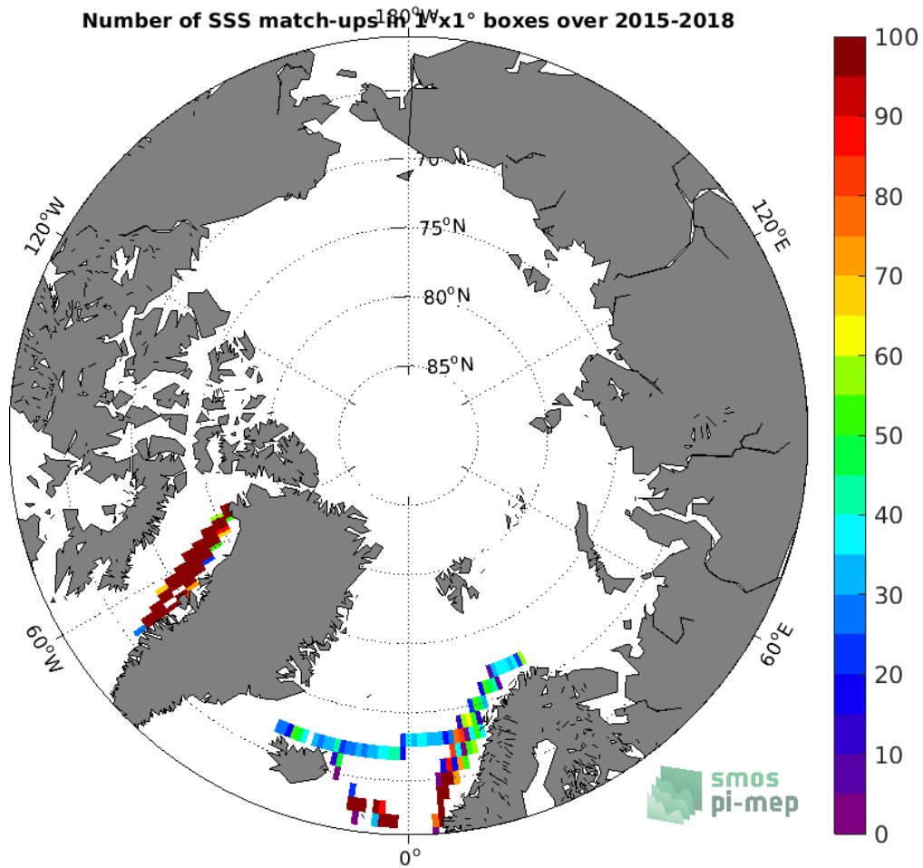
Figure 4: Number of SSS match-ups between TSG (LEGOS-DM) SSS and the SMAP SSS L3 v4 - Monthly (RSS) SSS product for the Arctic Ocean Pi-MEP region over 1°x1° boxes and for the full satellite product period.
