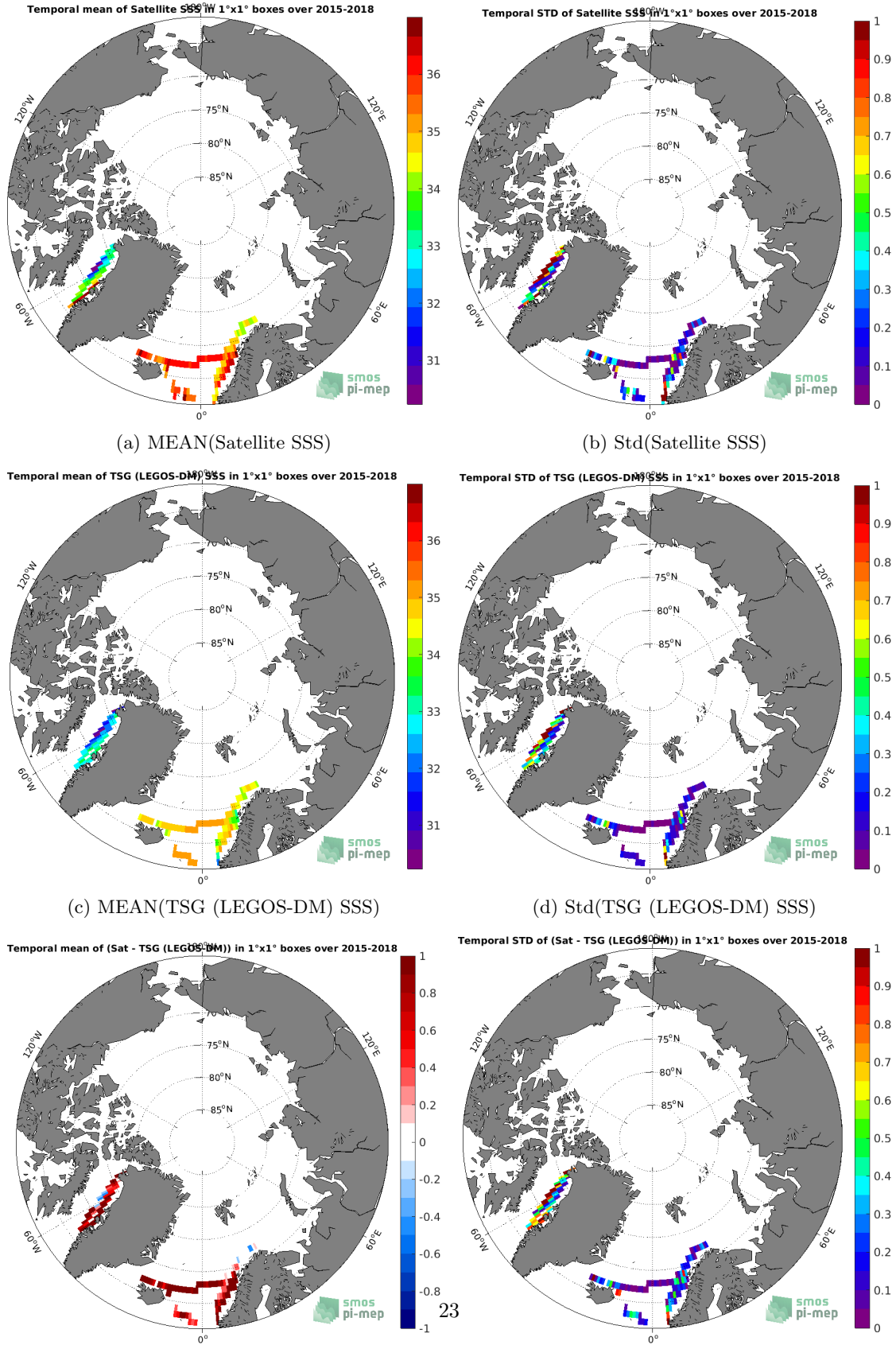
Figure 6: Temporal mean (left) and Std (right) of SSS from SMAP SSS L3 v4 - Monthly (RSS) (top), TSG (LEGOS-DM) (middle), and of \Delta SSS (Satellite - TSG (LEGOS-DM)). Only match-up pairs are used to generate these maps.
