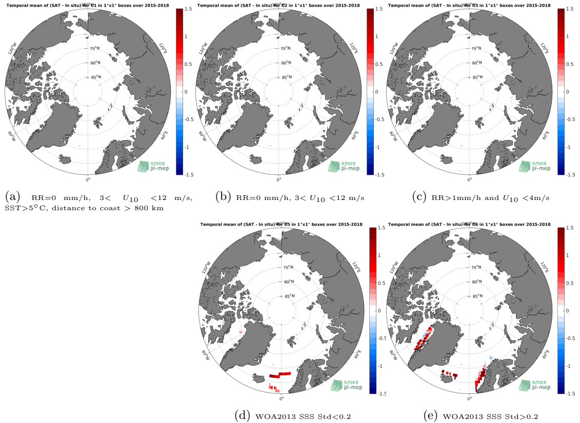
Figure 12: Temporal mean gridded over spatial boxes of size 1^{\circ}\times 1^{\circ} of \Delta\text{SSS} (SMAP-L3-RSS-V4-MONTHLY - TSG-LEGOS-DM) for 5 different subdatasets corresponding to:RR=0 mm/h, 3 < U_{10} < 12 m/s, SST > 5^{\circ}\text{C} , distance to coast > 800 km (a), RR=0 mm/h, 3 < U_{10} < 12 m/s (b), RR > 1 mm/h and U_{10} < 4 m/s (c), WOA2013 SSS Std < 0.2 (d), WOA2013 SSS Std > 0.2 (e).
