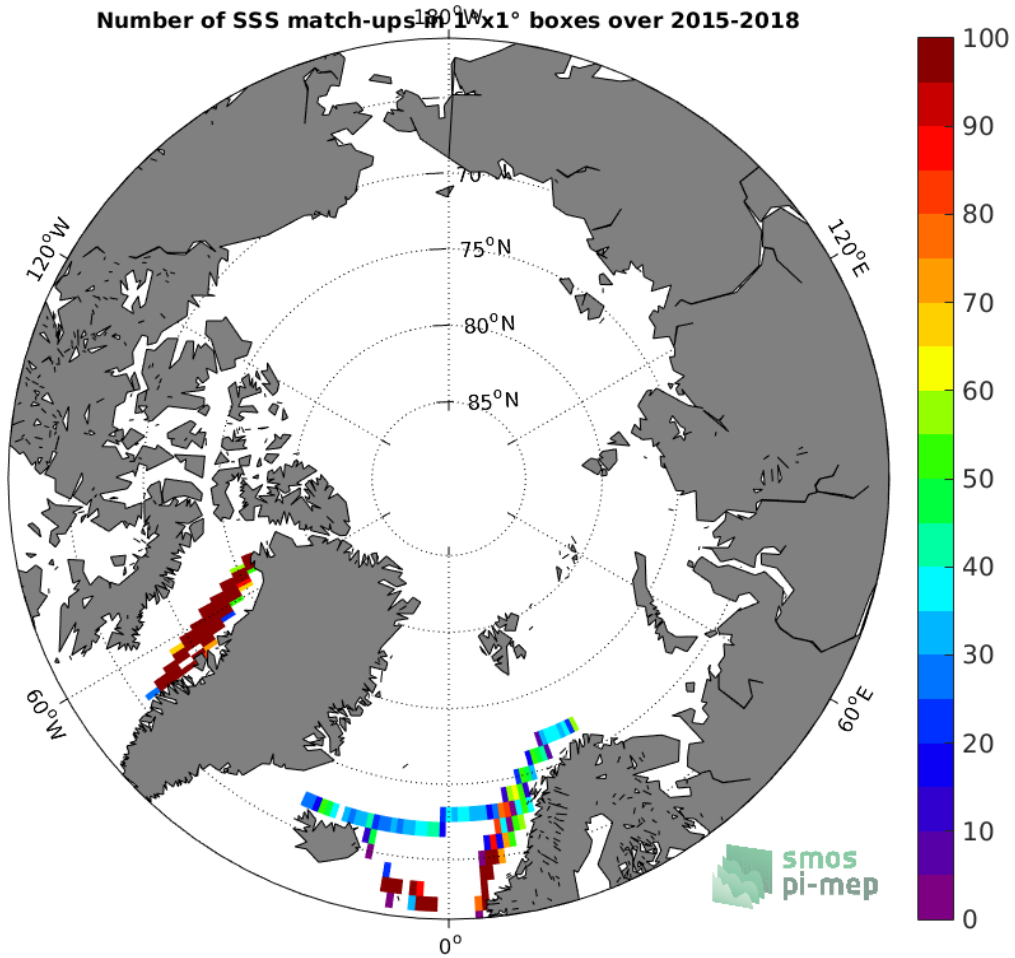
Figure 4: Number of SSS match-ups between TSG-LEGOS-DM SSS and the SMAP-L3-RSS-V4-MONTHLY SSS product for the Arctic Ocean Pi-MEP region over 1°x1° boxes and for the full satellite product period.
