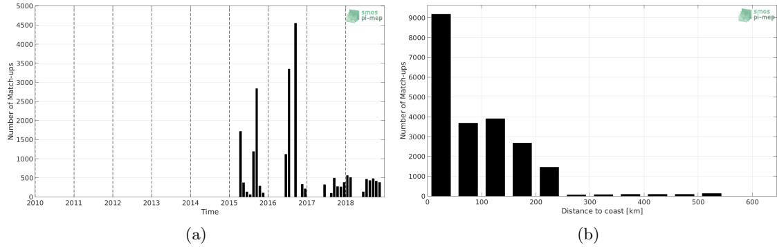
Figure 1: Number of match-ups between TSG-LEGOS-DM and SMAP-L3-RSS-V4-MONTHLY SSS as a function of time (a) and as function of the distance to coast (b) over the Arctic Ocean Pi-MEP region and for the full satellite product period.
