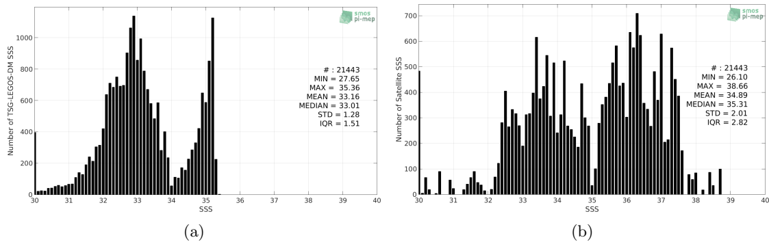
Figure 2: Histograms of SSS from TSG-LEGOS-DM (a) and SMAP-L3-RSS-V4-MONTHLY (b) considering all match-up pairs per bins of 0.1 over the Arctic Ocean Pi-MEP region and for the full satellite product period.
