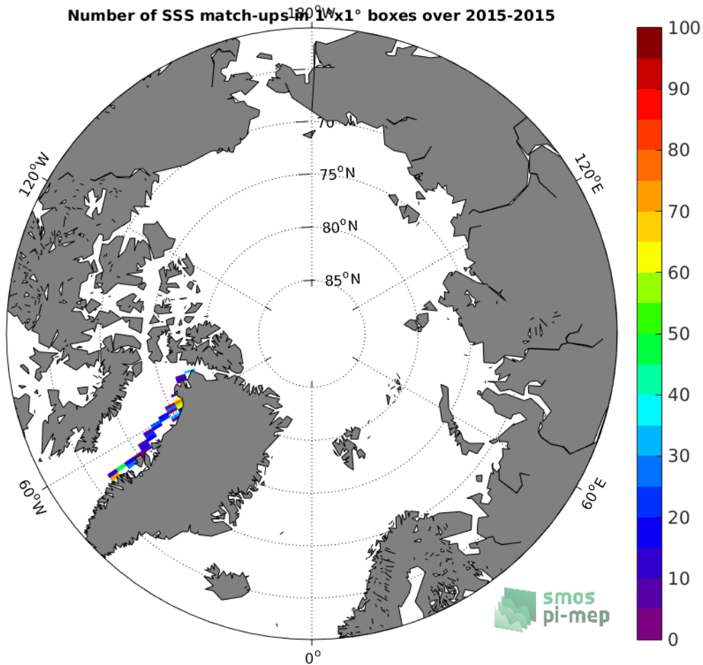
Figure 4: Number of SSS match-ups between TSG (GOSUD-Sailing-ship) SSS and the SMAP SSS L3 v4 - Monthly (RSS) SSS product for the Arctic Ocean Pi-MEP region over 1^\circ \times 1^\circ boxes and for the full satellite product period.
