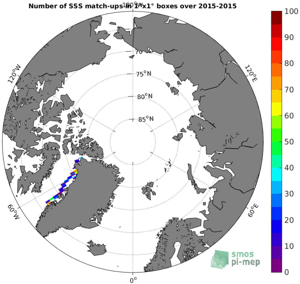
Figure 4: Number of SSS match-ups between TSG-GOSUD-Sailing-ship SSS and the SMAP-L3-RSS-V4-MONTHLY SSS product for the Arctic Ocean Pi-MEP region over 1°x1° boxes and for the full satellite product period.
