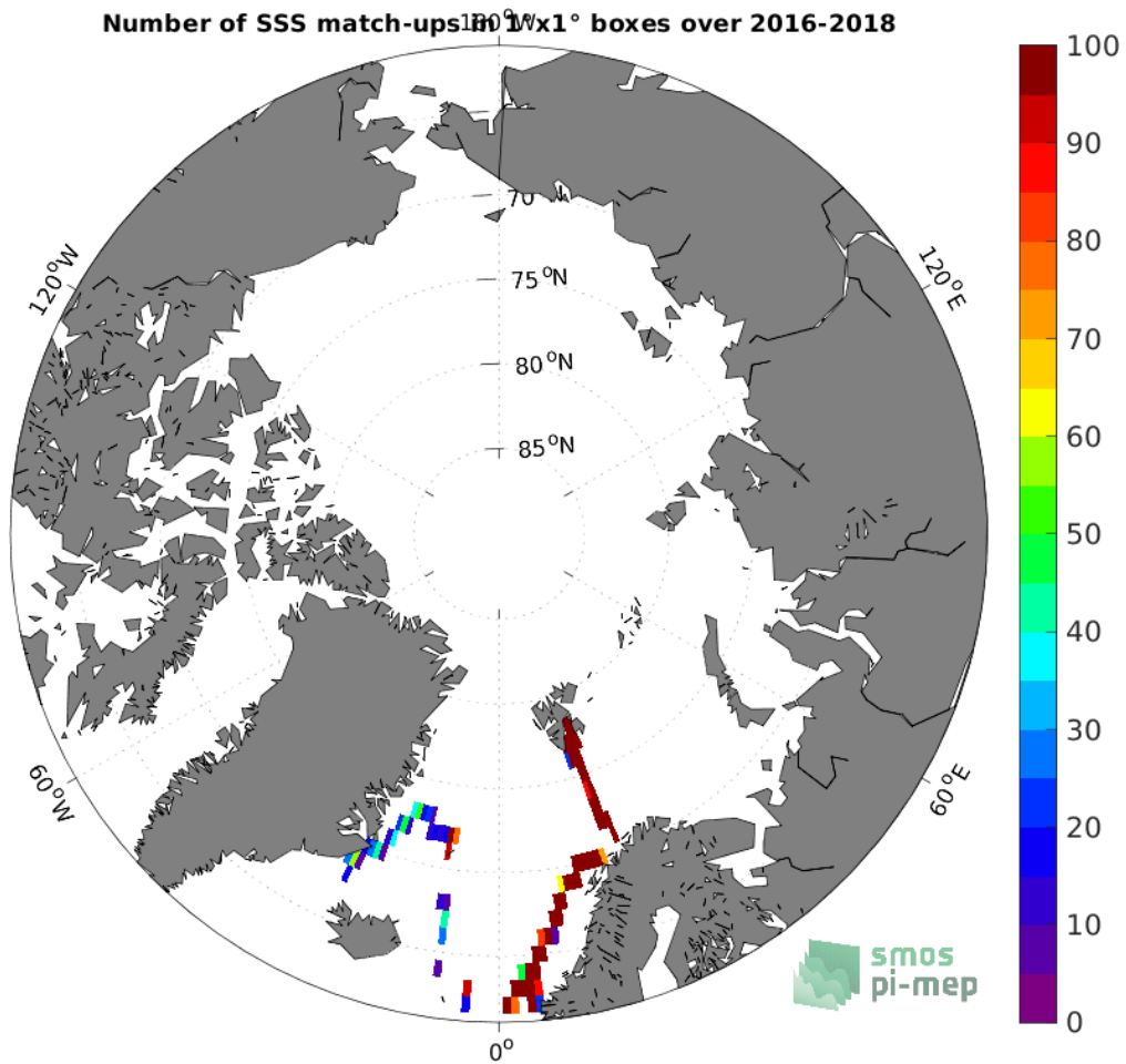
Figure 4: Number of SSS match-ups between TSG (GOSUD-Research-vessel) SSS and the SMAP SSS L3 v4 - Monthly (RSS) SSS product for the Arctic Ocean Pi-MEP region over 1^{\circ} \times 1^{\circ} boxes and for the full satellite product period.
