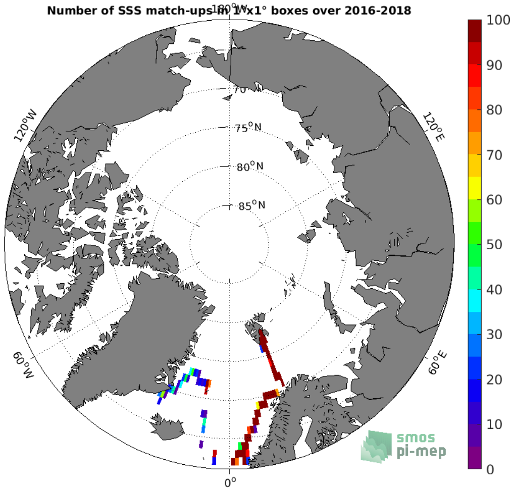
Figure 4: Number of SSS match-ups between TSG (GOSUD-Research-vessel) SSS and the SMAP SSS L3 v4 - Monthly (RSS) SSS product for the Arctic Ocean Pi-MEP region over 1^\circ \times 1^\circ boxes and for the full satellite product period.
