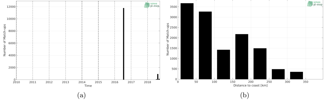
Figure 1: Number of match-ups between TSG (GOSUD-Research-vessel) and SMAP SSS L3 v4 - Monthly (RSS) SSS as a function of time (a) and as function of the distance to coast (b) over the Arctic Ocean Pi-MEP region and for the full satellite product period.
