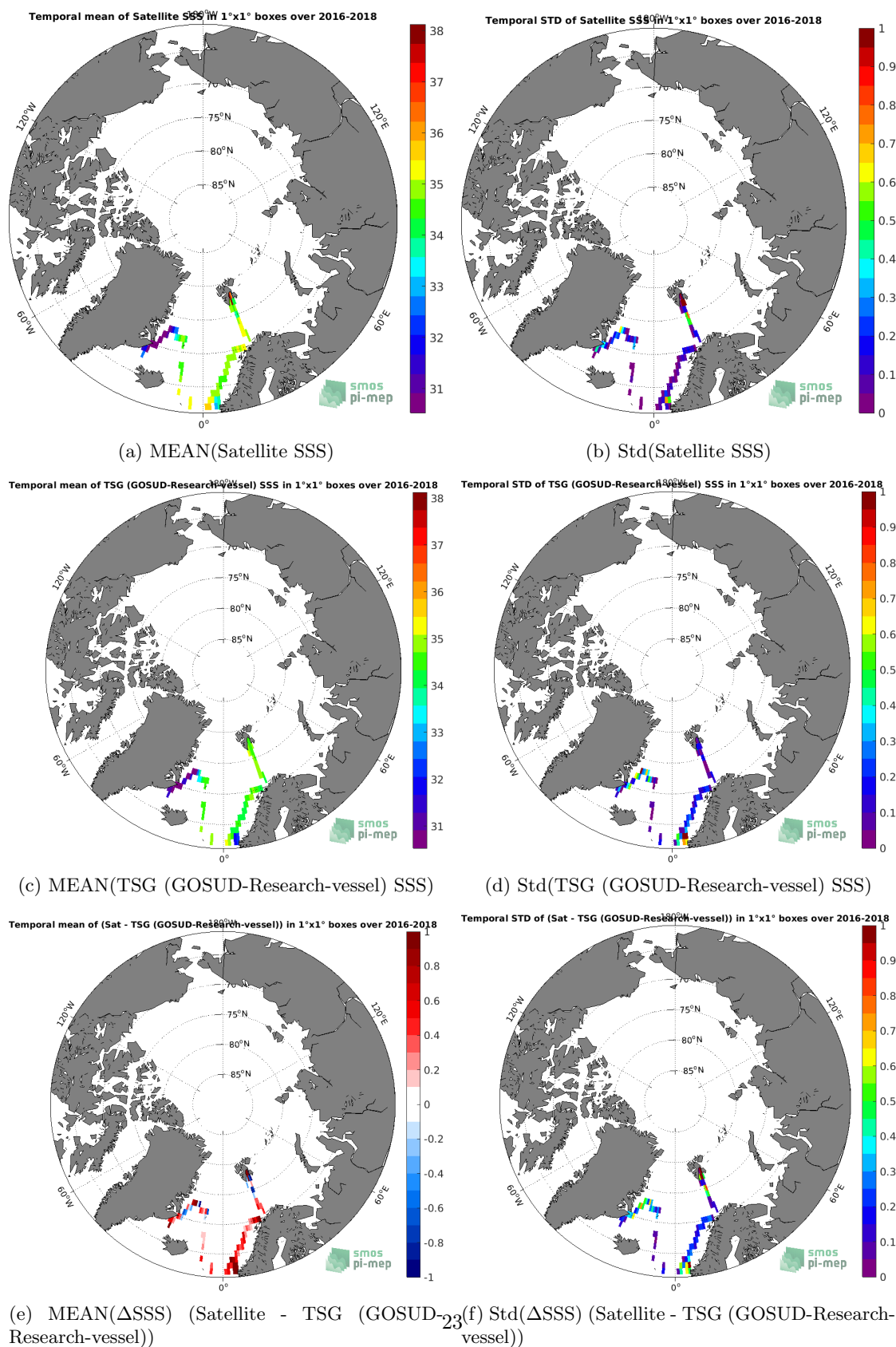
Figure 6: Temporal mean (left) and Std (right) of SSS from SMAP SSS L3 v4 - Monthly (RSS) (top), TSG (GOSUD-Research-vessel) (middle), and of \Delta SSS (Satellite - TSG (GOSUD-Research-vessel)). Only match-up pairs are used to generate these maps.
