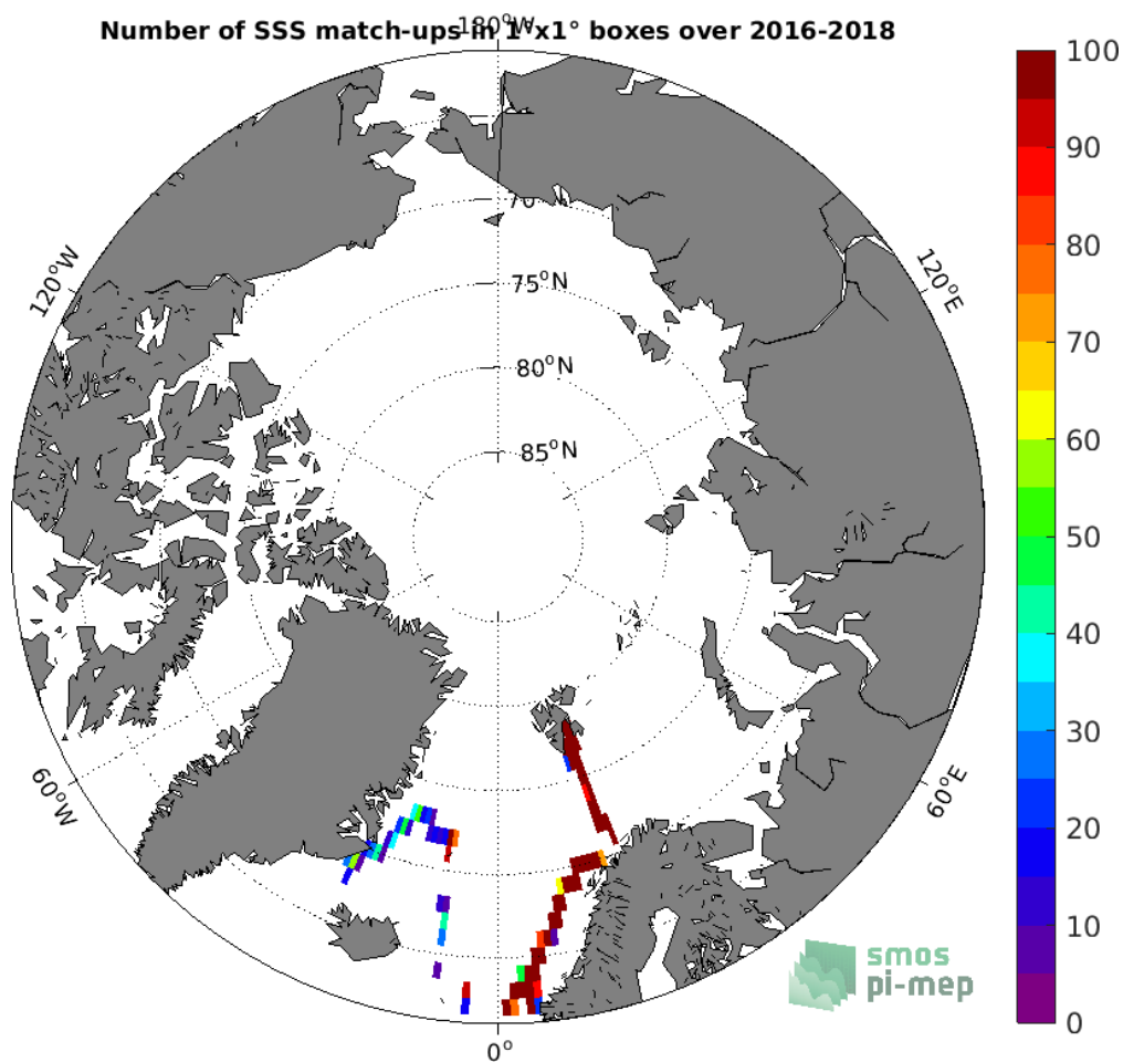
Figure 4: Number of SSS match-ups between TSG (GOSUD-Research-vessel) SSS and the SMAP SSS L3 v4 - Monthly (RSS) SSS product for the Arctic Ocean Pi-MEP region over 1°x1° boxes and for the full satellite product period.
