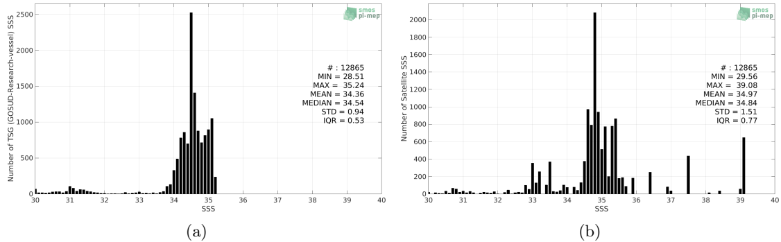
Figure 2: Histograms of SSS from TSG (GOSUD-Research-vessel) (a) and SMAP SSS L3 v4 - Monthly (RSS) (b) considering all match-up pairs per bins of 0.1 over the Arctic Ocean Pi-MEP region and for the full satellite product period.
