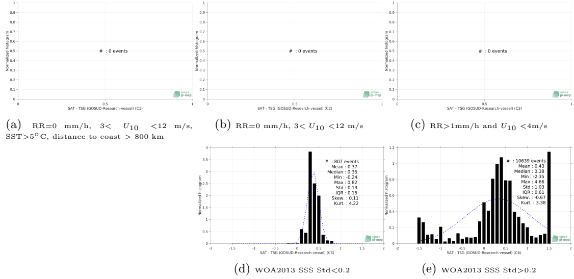
Figure 13: Normalized histogram of \Delta\text{SSS} (SMAP SSS L3 v4 - Monthly (RSS) - TSG (GOSUD-Research-vessel)) for 5 different subdatasets corresponding to: RR=0 mm/h, 3 < U_{10} < 12 m/s, SST > 5^\circ\text{C} , distance to coast > 800 km (a), RR=0 mm/h, 3 < U_{10} < 12 m/s (b), RR > 1\text{mm/h} and U_{10} < 4\text{m/s} (c), WOA2013 SSS Std <0.2 (d), WOA2013 SSS Std >0.2 (e).
