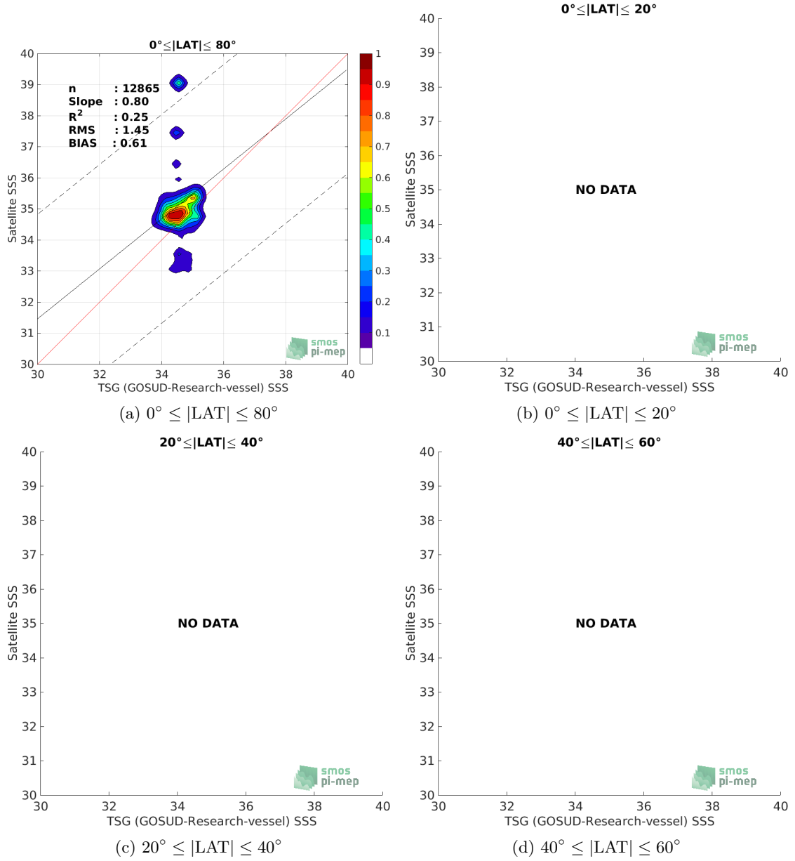
Figure 9: Contour maps of the concentration of SMAP SSS L3 v4 - Monthly (RSS) SSS (y-axis) versus TSG (GOSUD-Research-vessel) SSS (x-axis) at match-up pairs for different latitude bands. For each plot, the red line shows x=y . The black thin and dashed lines indicate a linear fit through the data cloud and the \pm 95\% confidence levels, respectively. The number match-up pairs n , the slope and R^2 coefficient of the linear fit, the root mean square (RMS) and the mean bias between satellite and in situ data are indicated for each latitude band in each plots.
