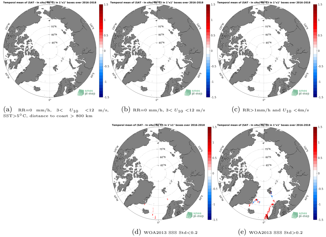
Figure 12: Temporal mean gridded over spatial boxes of size 1^\circ \times 1^\circ of \Delta\text{SSS} (SMAP SSS L3 v4 - Monthly (RSS) - TSG (GOSUD-Research-vessel)) for 5 different subdatasets corresponding to: RR=0 mm/h, 3 < U_{10} < 12 m/s, SST > 5^\circ\text{C} , distance to coast > 800 km (a), RR=0 mm/h, 3 < U_{10} < 12 m/s (b), RR > 1 mm/h and U_{10} < 4 m/s (c), WOA2013 SSS Std < 0.2 (d), WOA2013 SSS Std > 0.2 (e).
