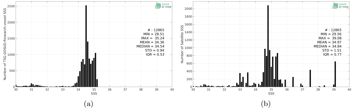
Figure 2: Histograms of SSS from TSG-GOSUD-Research-vessel (a) and SMAP-L3-RSS-V4-MONTHLY (b) considering all match-up pairs per bins of 0.1 over the Arctic Ocean Pi-MEP region and for the full satellite product period.
