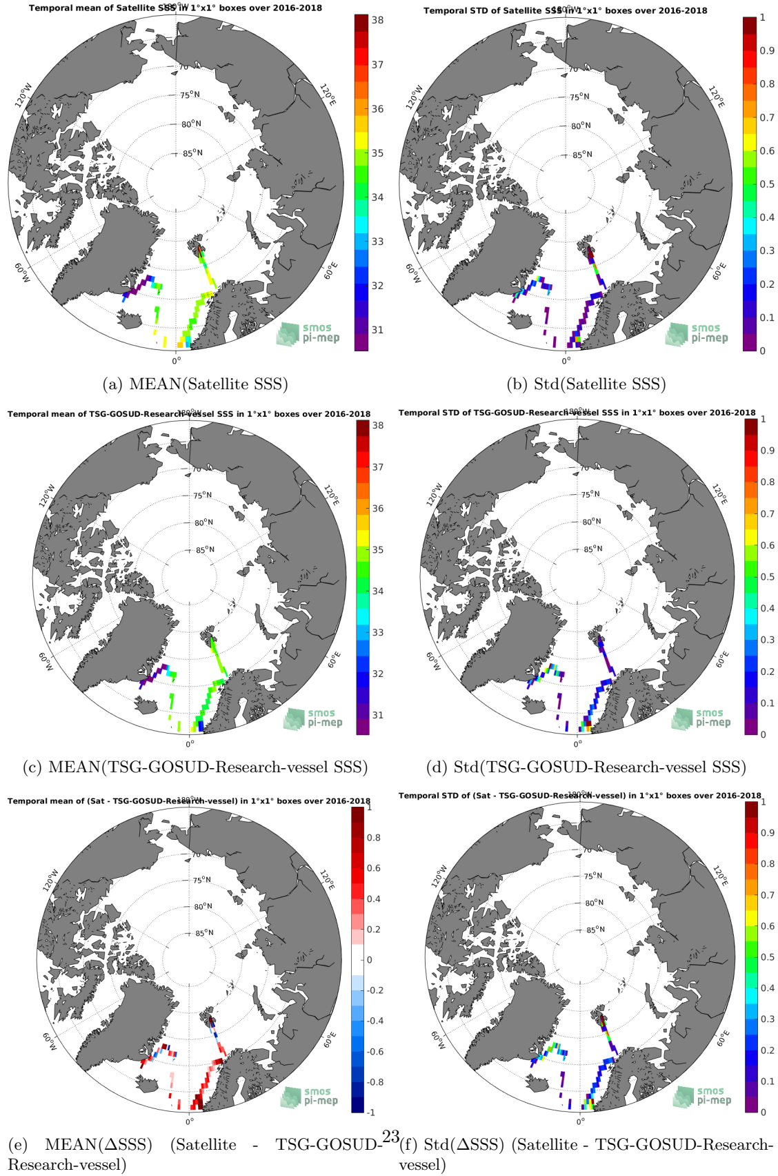
Figure 6: Temporal mean (left) and Std (right) of SSS from SMAP-L3-RSS-V4-MONTHLY (top), TSG-GOSUD-Research-vessel (middle), and of \Delta SSS (Satellite - TSG-GOSUD-Research-vessel). Only match-up pairs are used to generate these maps.
