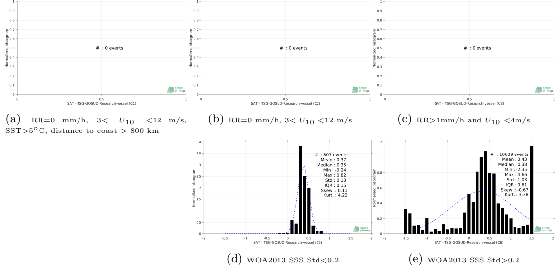
Figure 13: Normalized histogram of \Delta\text{SSS} (SMAP-L3-RSS-V4-MONTHLY - TSG-GOSUD-Research-vessel) for 5 different subdatasets corresponding to: RR=0 mm/h, 3 < U_{10} < 12 m/s, SST >5^{\circ}\text{C} , distance to coast > 800 km (a), RR=0 mm/h, 3 < U_{10} < 12 m/s (b), RR>1\text{mm/h} and U_{10} < 4\text{m/s} (c), WOA2013 SSS Std <0.2 (d), WOA2013 SSS Std >0.2 (e).
