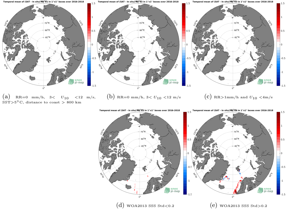
Figure 12: Temporal mean gridded over spatial boxes of size 1^\circ \times 1^\circ of \Delta\text{SSS} (SMAP-L3-RSS-V4-MONTHLY - TSG-GOSUD-Research-vessel) for 5 different subdatasets corresponding to: RR=0 mm/h, 3 < U_{10} < 12 m/s, SST > 5^\circ\text{C} , distance to coast > 800 km (a), RR=0 mm/h, 3 < U_{10} < 12 m/s (b), RR > 1 mm/h and U_{10} < 4 m/s (c), WOA2013 SSS Std < 0.2 (d), WOA2013 SSS Std > 0.2 (e).
