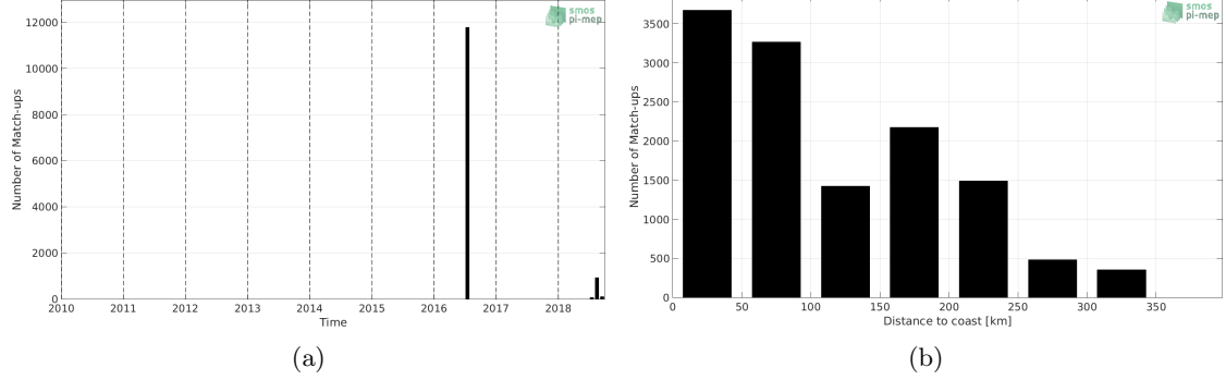
Figure 1: Number of match-ups between TSG-GOSUD-Research-vessel and SMAP-L3-RSS-V4-MONTHLY SSS as a function of time (a) and as function of the distance to coast (b) over the Arctic Ocean Pi-MEP region and for the full satellite product period.
