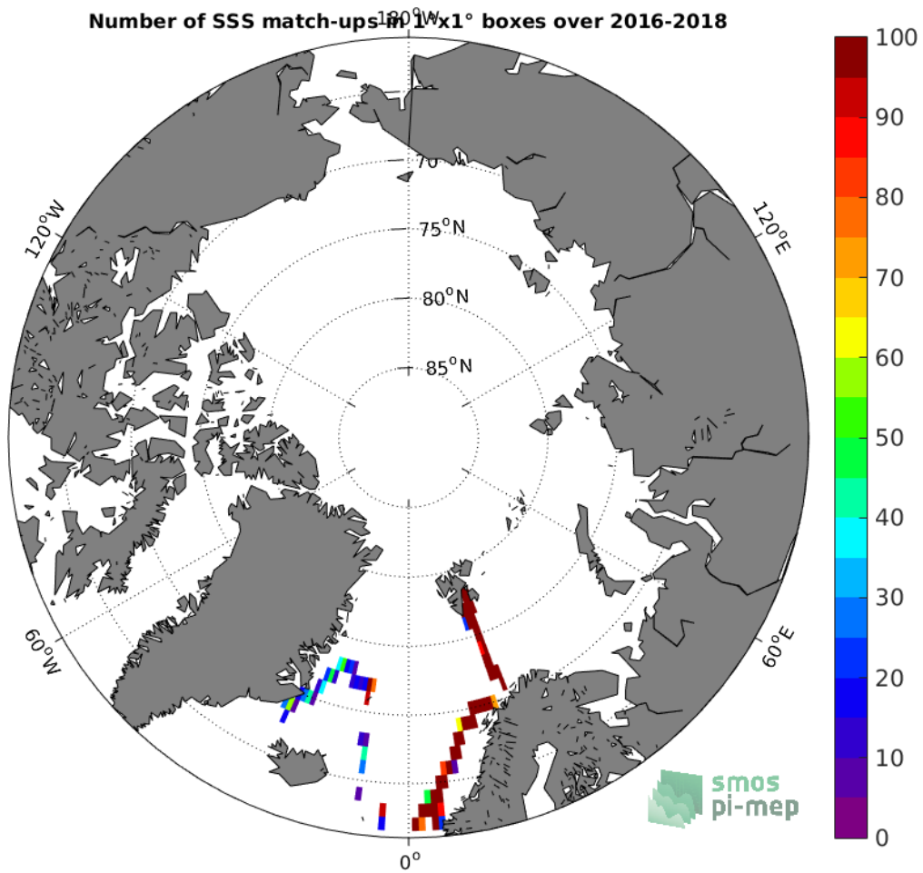
Figure 4: Number of SSS match-ups between TSG-GOSUD-Research-vessel SSS and the SMAP-L3-RSS-V4-MONTHLY SSS product for the Arctic Ocean Pi-MEP region over 1^\circ \times 1^\circ boxes and for the full satellite product period.
