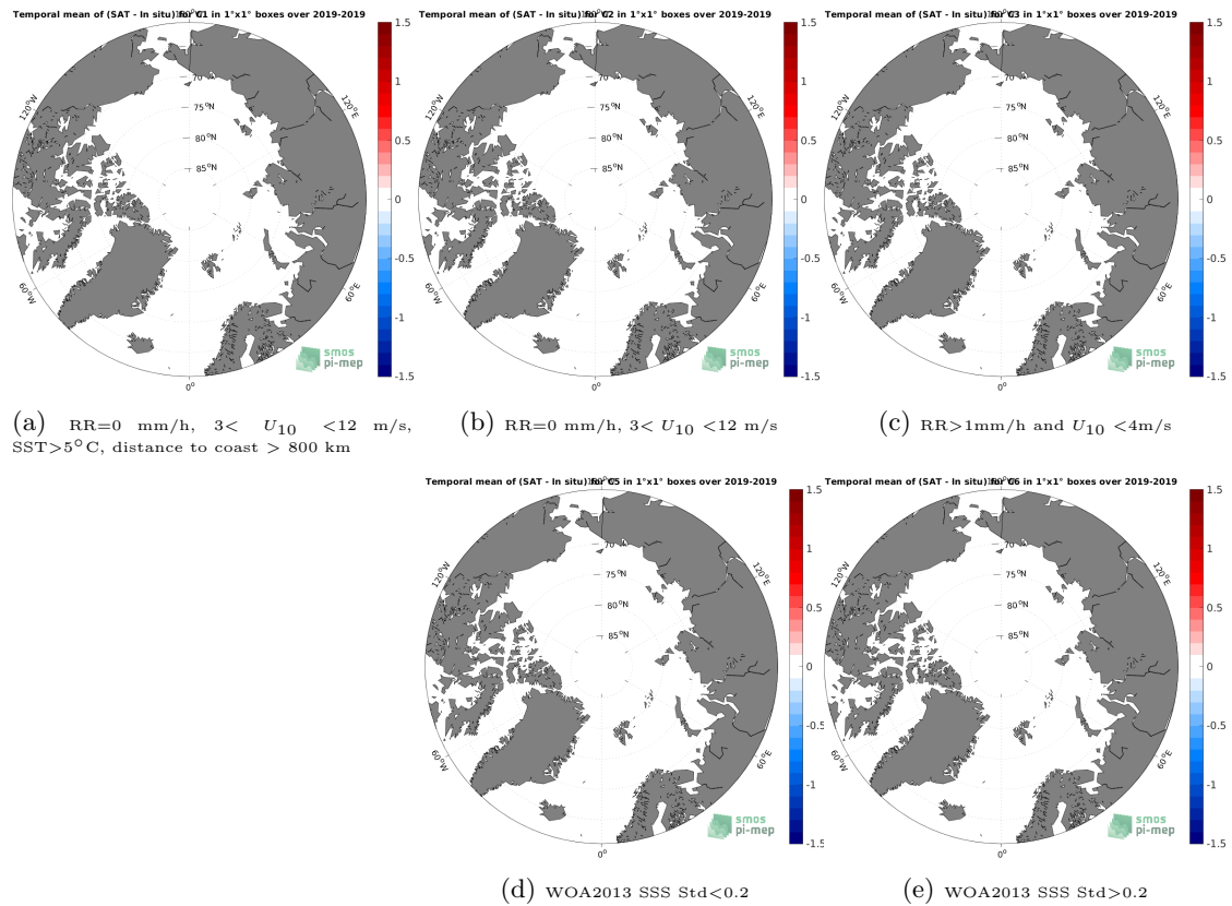
Figure 11: Temporal mean gridded over spatial boxes of size 1^{\circ}\times 1^{\circ} of \Delta\text{SSS} (SMAP SSS L3 v4 - Monthly (RSS) - Surface drifters) for 5 different subdatasets corresponding to:RR=0 mm/h, 3 < U_{10} < 12 m/s, SST >5^{\circ}\text{C} , distance to coast > 800 km (a), RR=0 mm/h, 3 < U_{10} < 12 m/s (b), RR >1 mm/h and U_{10} < 4 m/s (c), WOA2013 SSS Std <0.2 (d), WOA2013 SSS Std >0.2 (e).
