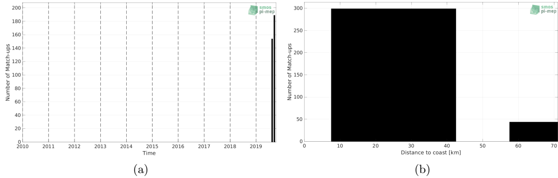
Figure 1: Number of match-ups between Surface drifters and SMAP SSS L3 v4 - Monthly (RSS) SSS as a function of time (a) and as function of the distance to coast (b) over the Arctic Ocean Pi-MEP region and for the full satellite product period.
