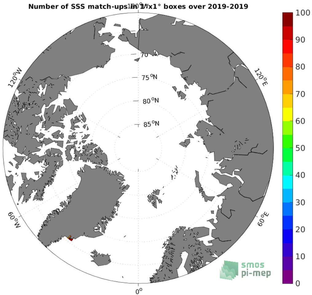
Figure 3: Number of SSS match-ups between Surface drifters SSS and the SMAP SSS L3 v4 - Monthly (RSS) SSS product for the Arctic Ocean Pi-MEP region over 1^\circ \times 1^\circ boxes and for the full satellite product period.
