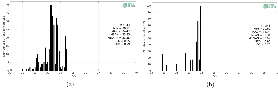
Figure 2: Histograms of SSS from Surface drifters (a) and SMAP SSS L3 v4 - Monthly (RSS) (b) considering all match-up pairs per bins of 0.1 over the Arctic Ocean Pi-MEP region and for the full satellite product period.
