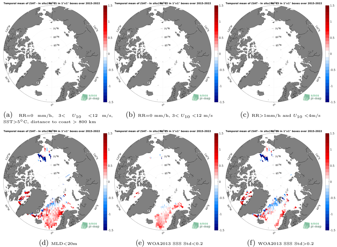
Figure 12: Temporal mean gridded over spatial boxes of size 1^{\circ}\times 1^{\circ} of \Delta\text{SSS} (SMAP SSS L3 v4 - Monthly (RSS) - Argo) for 6 different subdatasets corresponding to:RR=0 mm/h, 3 < U_{10} < 12 m/s, SST > 5^{\circ}\text{C} , distance to coast > 800 km (a), RR=0 mm/h, 3 < U_{10} < 12 m/s (b), RR > 1\text{mm/h} and U_{10} < 4\text{m/s} (c),MLD < 20\text{m} (d),WOA2013 SSS Std < 0.2 (e),WOA2013 SSS Std > 0.2 (f).
