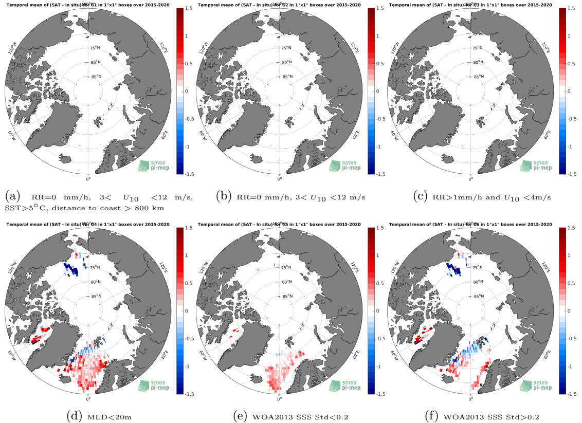
Figure 12: Temporal mean gridded over spatial boxes of size 1^{\circ}\times 1^{\circ} of \Delta\text{SSS} (SMAP-L3-RSS-V4-MONTHLY - Argo) for 6 different subdatasets corresponding to: RR=0 mm/h, 3 < U_{10} < 12 m/s, SST > 5^{\circ}\text{C} , distance to coast > 800 km (a), RR=0 mm/h, 3 < U_{10} < 12 m/s (b), RR > 1\text{mm/h} and U_{10} < 4\text{m/s} (c), MLD < 20\text{m} (d), WOA2013 SSS Std < 0.2 (e), WOA2013 SSS Std > 0.2 (f).
