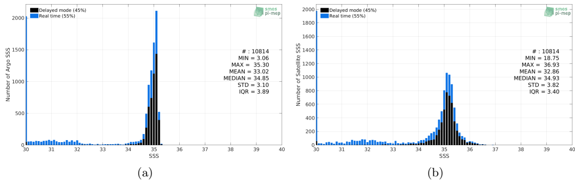
Figure 2: Histograms of SSS from Argo (a) and SMAP-L3-RSS-V4-MONTHLY (b) considering all match-up pairs per bins of 0.1 over the Arctic Ocean Pi-MEP region and for the full satellite product period.
