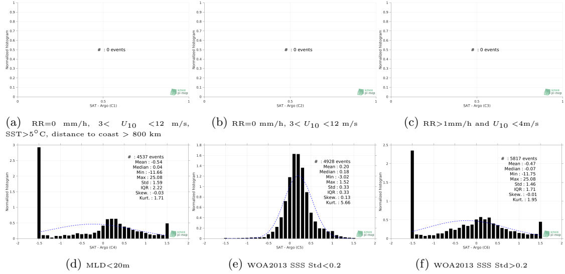
Figure 13: Normalized histogram of \Delta SSS (SMAP-L3-RSS-V4-MONTHLY - Argo) for 6 different subdatasets corresponding to: RR=0 mm/h, 3 < U_{10} < 12 m/s, SST > 5°C, distance to coast > 800 km (a), RR=0 mm/h, 3 < U_{10} < 12 m/s (b), RR > 1mm/h and U_{10} < 4 m/s (c), MLD < 20m (d), WOA2013 SSS Std < 0.2 (e), WOA2013 SSS Std > 0.2 (f).
