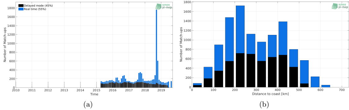
Figure 1: Number of match-ups between Argo and SMAP-L3-RSS-V4-MONTHLY SSS as a function of time (a) and as function of the distance to coast (b) over the Arctic Ocean Pi-MEP region and for the full satellite product period.
