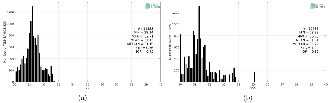
Figure 2: Histograms of SSS from TSG-SAMOS (a) and SMAP-L3-RSS-V3-8DAY-RUNNING-40KM (b) considering all match-up pairs per bins of 0.1 over the Arctic Ocean Pi-MEP region and for the full satellite product period.
