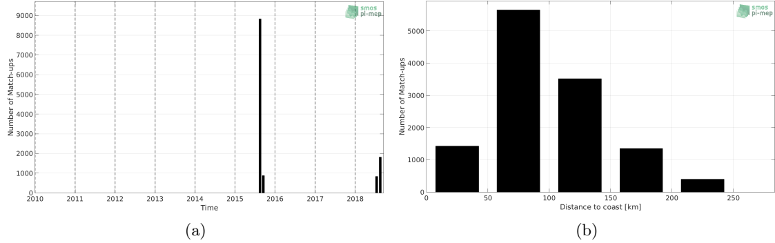
Figure 1: Number of match-ups between TSG-SAMOS and SMAP-L3-RSS-V3-8DAY-RUNNING-40KM SSS as a function of time (a) and as function of the distance to coast (b) over the Arctic Ocean Pi-MEP region and for the full satellite product period.
