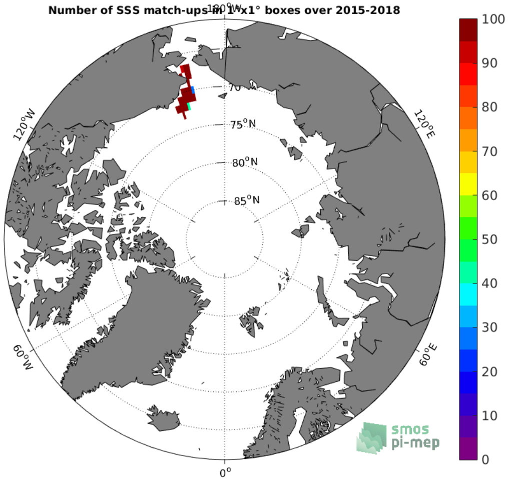
Figure 4: Number of SSS match-ups between TSG-SAMOS SSS and the SMAP-L3-RSS-V3-8DAY-RUNNING-40KM SSS product for the Arctic Ocean Pi-MEP region over 1°x1° boxes and for the full satellite product period.
