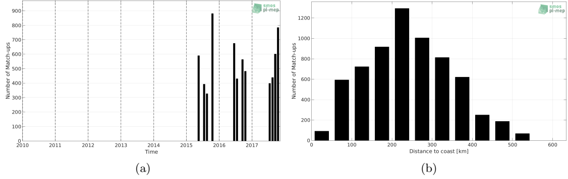
Figure 1: Number of match-ups between TSG-POLARSTERN and SMAP-L3-RSS-V3-8DAY-RUNNING-40KM SSS as a function of time (a) and as function of the distance to coast (b) over the Arctic Ocean Pi-MEP region and for the full satellite product period.
