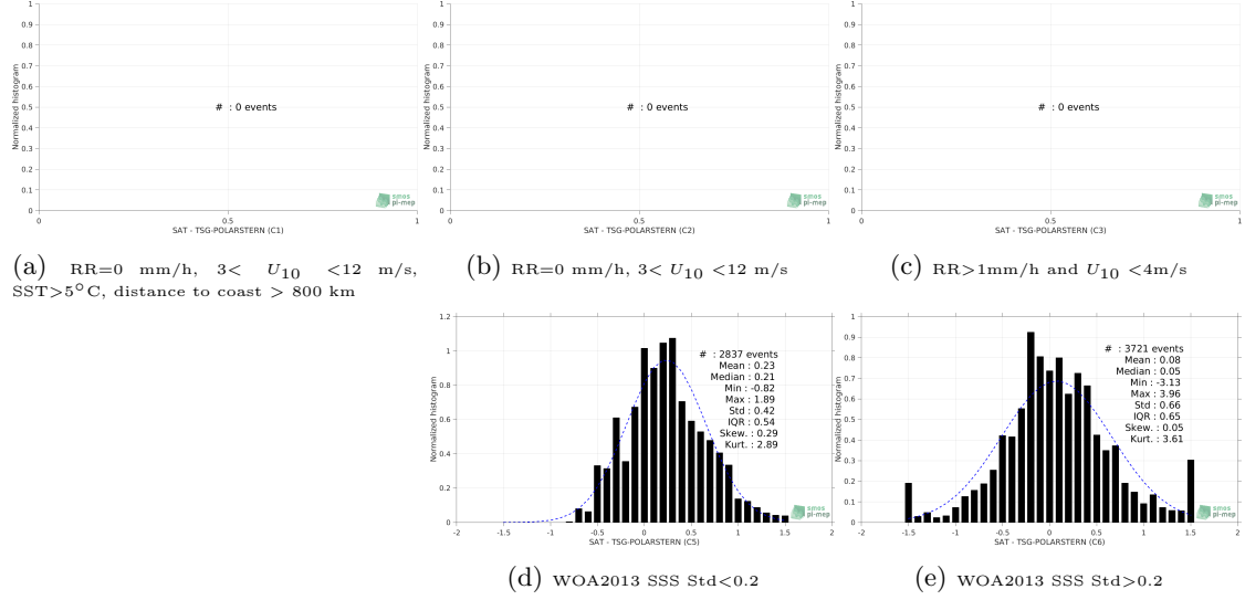
Figure 13: Normalized histogram of \Delta\text{SSS} (SMAP-L3-RSS-V3-8DAY-RUNNING-40KM - TSG-POLARSTERN) for 5 different subdatasets corresponding to: RR=0 mm/h, 3 < U_{10} < 12 m/s, SST > 5^\circ\text{C} , distance to coast > 800 km (a), RR=0 mm/h, 3 < U_{10} < 12 m/s (b), RR > 1 mm/h and U_{10} < 4 m/s (c), WOA2013 SSS Std < 0.2 (d), WOA2013 SSS Std > 0.2 (e).
