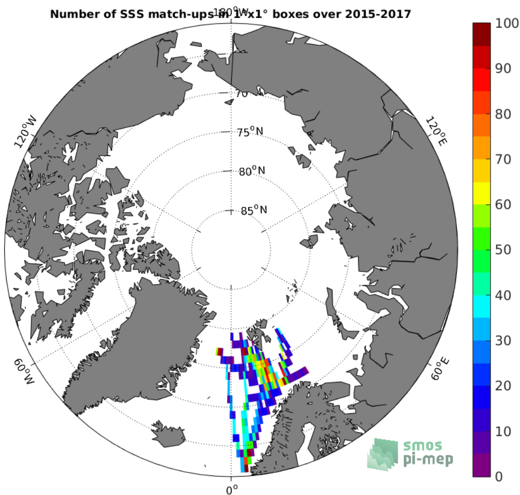
Figure 4: Number of SSS match-ups between TSG-POLARSTERN SSS and the SMAP-L3-RSS-V3-8DAY-RUNNING-40KM SSS product for the Arctic Ocean Pi-MEP region over 1^\circ \times 1^\circ boxes and for the full satellite product period.
