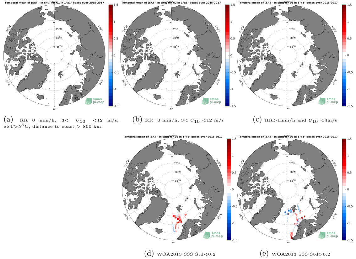
Figure 12: Temporal mean gridded over spatial boxes of size 1^\circ \times 1^\circ of \Delta SSS (SMAP-L3-RSS-V3-8DAY-RUNNING-40KM - TSG-POLARSTERN) for 5 different subdatasets corresponding to: RR=0 mm/h, 3 < U_{10} < 12 m/s, SST > 5^\circ C , distance to coast > 800 km (a), RR=0 mm/h, 3 < U_{10} < 12 m/s (b), RR > 1 mm/h and U_{10} < 4 m/s (c), WOA2013 SSS Std < 0.2 (d), WOA2013 SSS Std > 0.2 (e).
