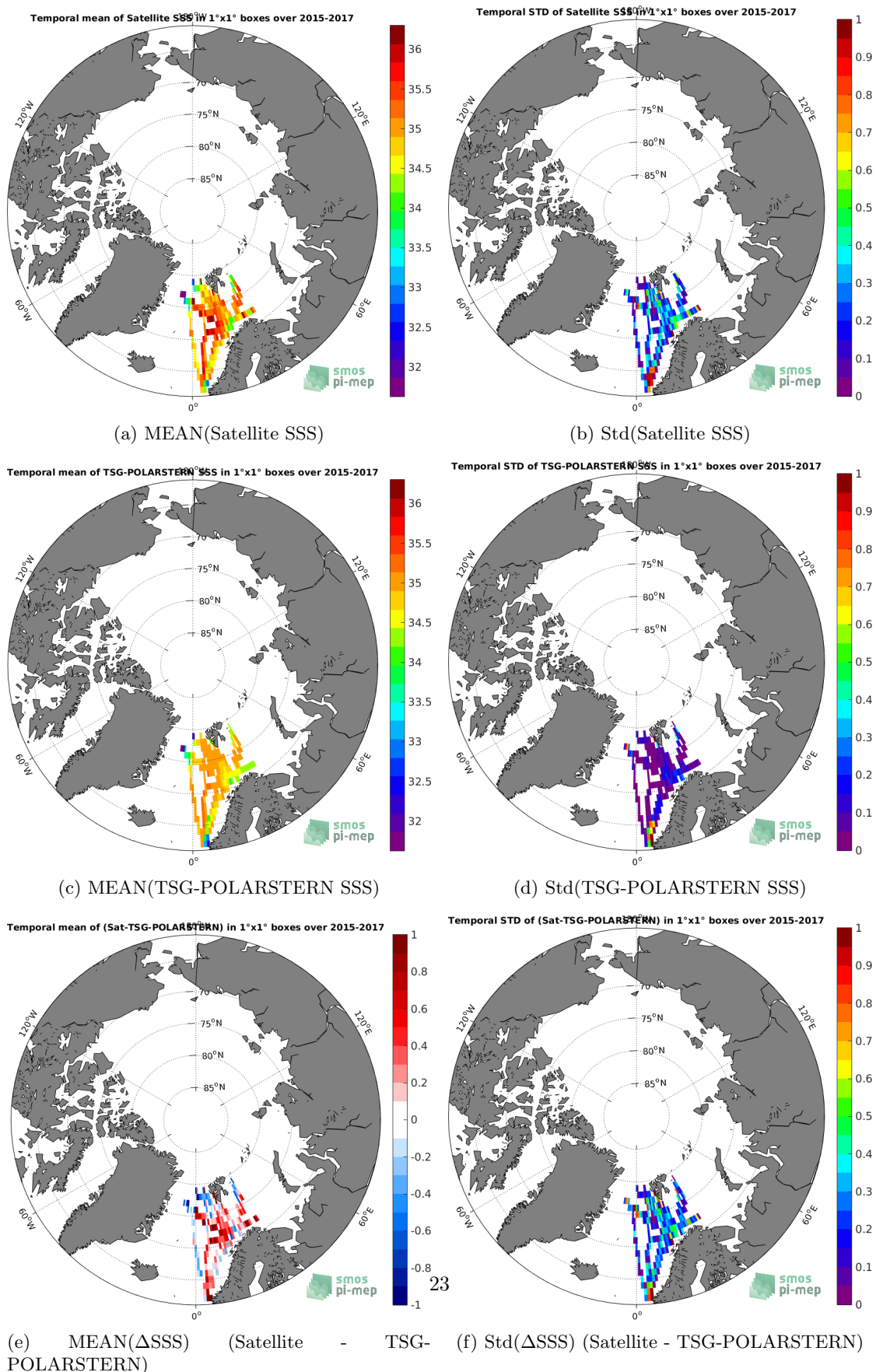
Figure 6: Temporal mean (left) and Std (right) of SSS from SMAP-L3-RSS-V3-8DAY-RUNNING-40KM (top), TSG-POLARSTERN (middle), and of \Delta SSS (Satellite - TSG-POLARSTERN). Only match-up pairs are used to generate these maps.
