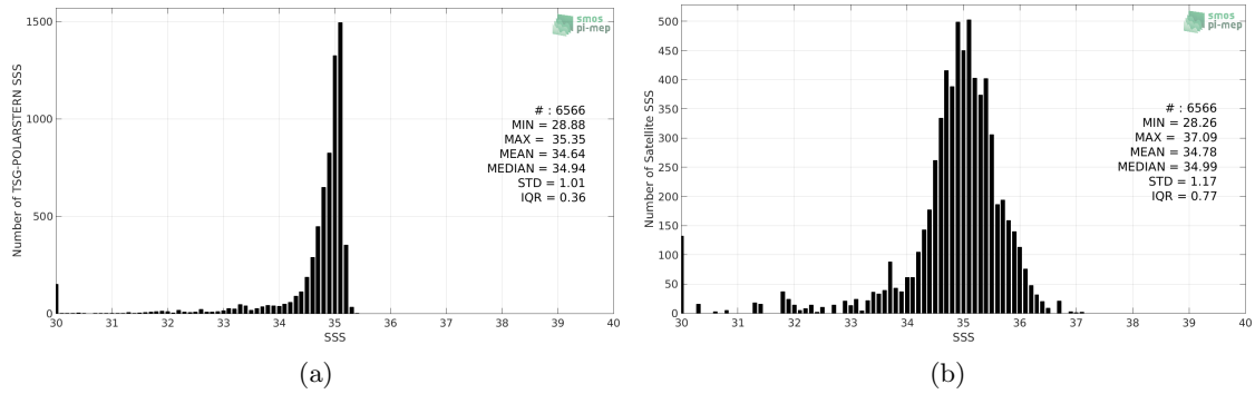
Figure 2: Histograms of SSS from TSG-POLARSTERN (a) and SMAP-L3-RSS-V3-8DAY-RUNNING-40KM (b) considering all match-up pairs per bins of 0.1 over the Arctic Ocean Pi-MEP region and for the full satellite product period.
