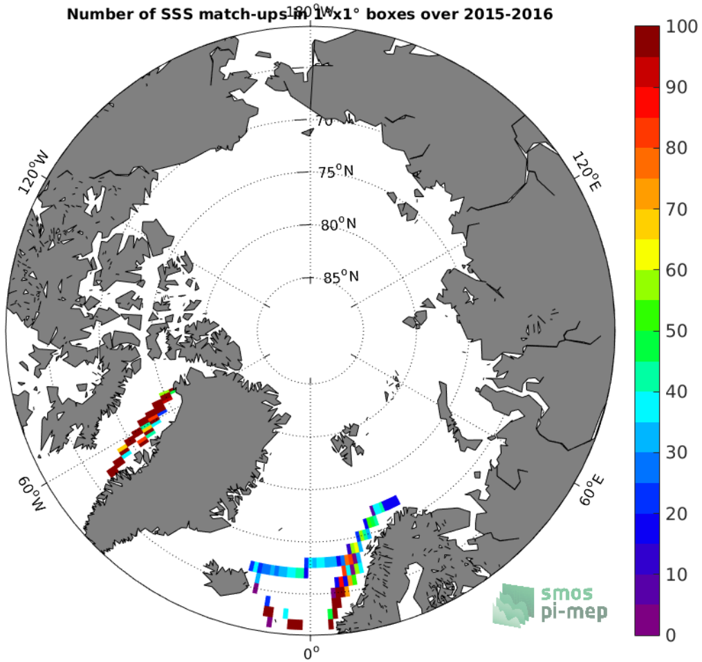
Figure 4: Number of SSS match-ups between TSG-LEGOS-DM SSS and the SMAP-L3-RSS-V3-8DAY-RUNNING-40KM SSS product for the Arctic Ocean Pi-MEP region over 1^\circ \times 1^\circ boxes and for the full satellite product period.
