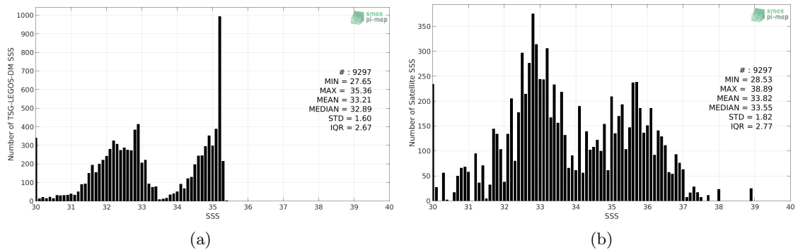
Figure 2: Histograms of SSS from TSG-LEGOS-DM (a) and SMAP-L3-RSS-V3-8DAY-RUNNING-40KM (b) considering all match-up pairs per bins of 0.1 over the Arctic Ocean Pi-MEP region and for the full satellite product period.
