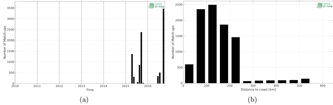
Figure 1: Number of match-ups between TSG-LEGOS-DM and SMAP-L3-RSS-V3-8DAY-RUNNING-40KM SSS as a function of time (a) and as function of the distance to coast (b) over the Arctic Ocean Pi-MEP region and for the full satellite product period.
