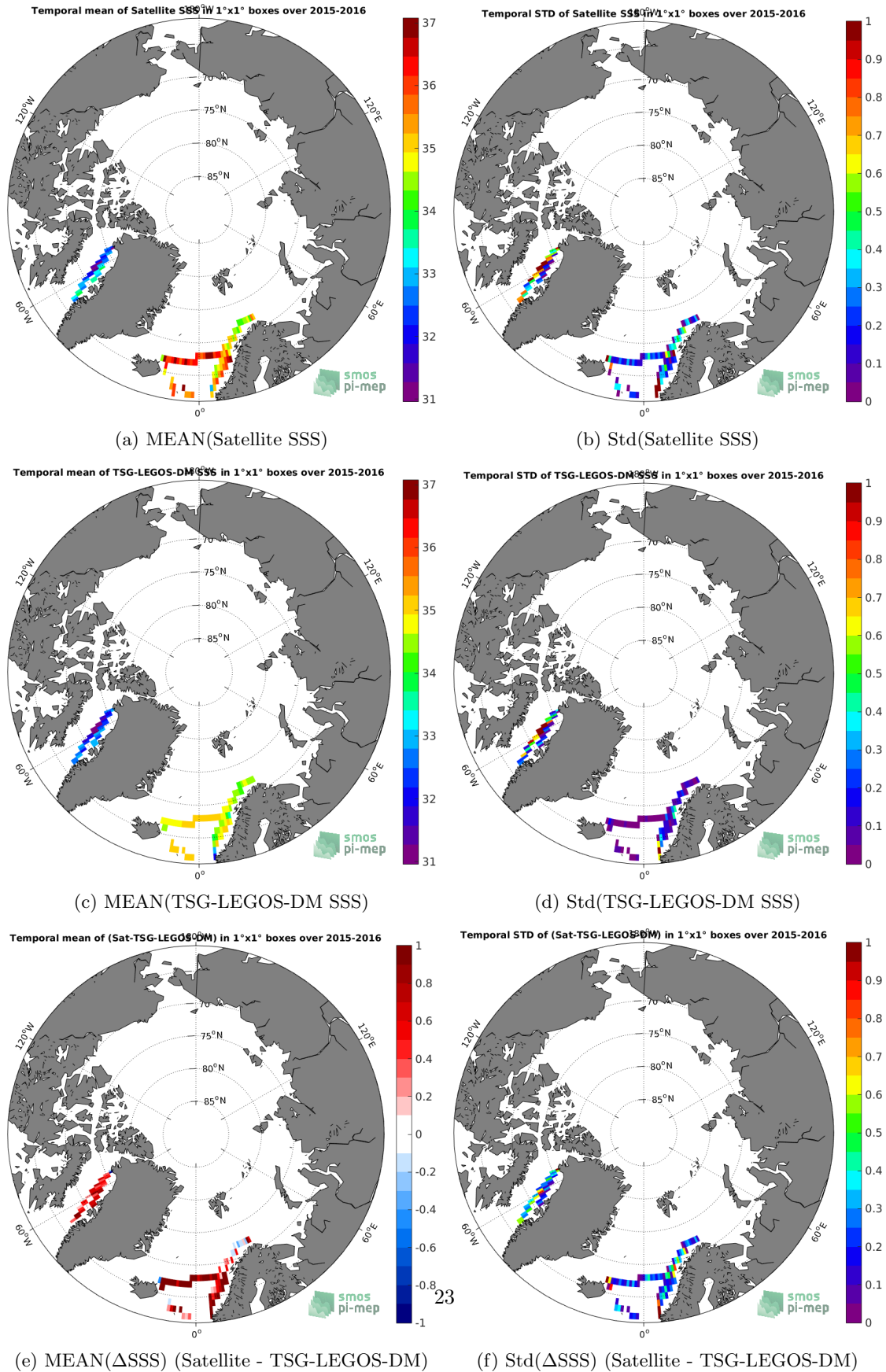
Figure 6: Temporal mean (left) and Std (right) of SSS from SMAP-L3-RSS-V3-8DAY-RUNNING-40KM (top), TSG-LEGOS-DM (middle), and of \Delta SSS (Satellite - TSG-LEGOS-DM). Only match-up pairs are used to generate these maps.
