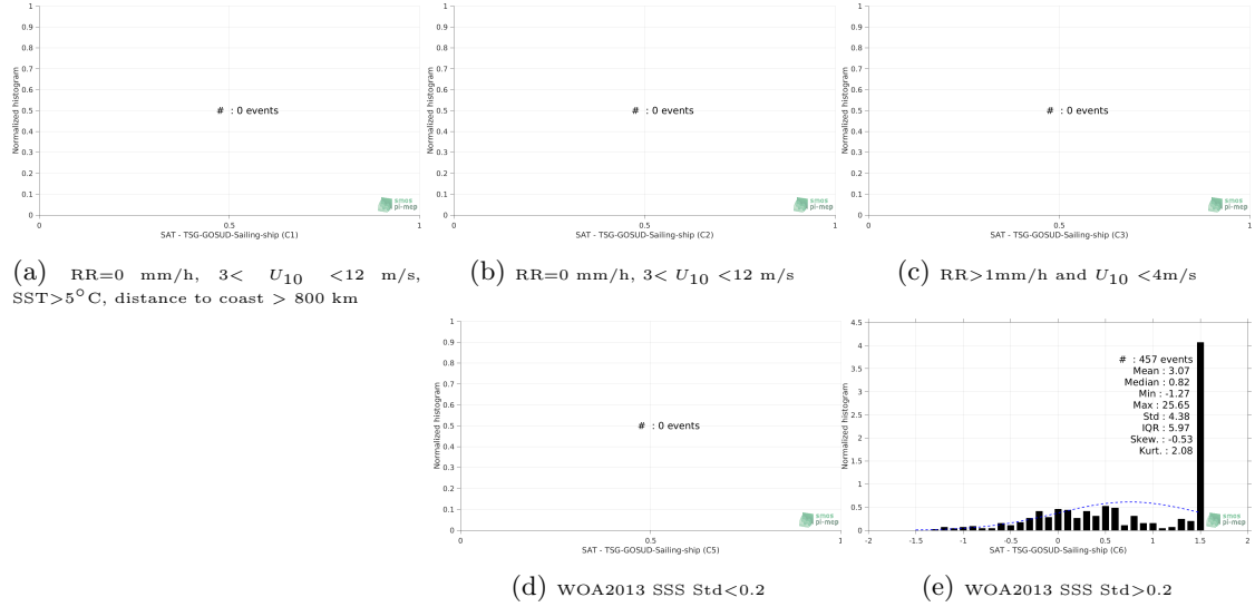
Figure 13: Normalized histogram of \Delta\text{SSS} (SMAP-L3-RSS-V3-8DAY-RUNNING-40KM - TSG-GOSUD-Sailing-ship) for 5 different subdatasets corresponding to: RR=0 mm/h, 3 < U_{10} < 12 m/s, SST > 5^{\circ}\text{C} , distance to coast > 800 km (a), RR=0 mm/h, 3 < U_{10} < 12 m/s (b), RR > 1\text{mm/h} and U_{10} < 4\text{m/s} (c), WOA2013 SSS Std < 0.2 (d), WOA2013 SSS Std > 0.2 (e).
