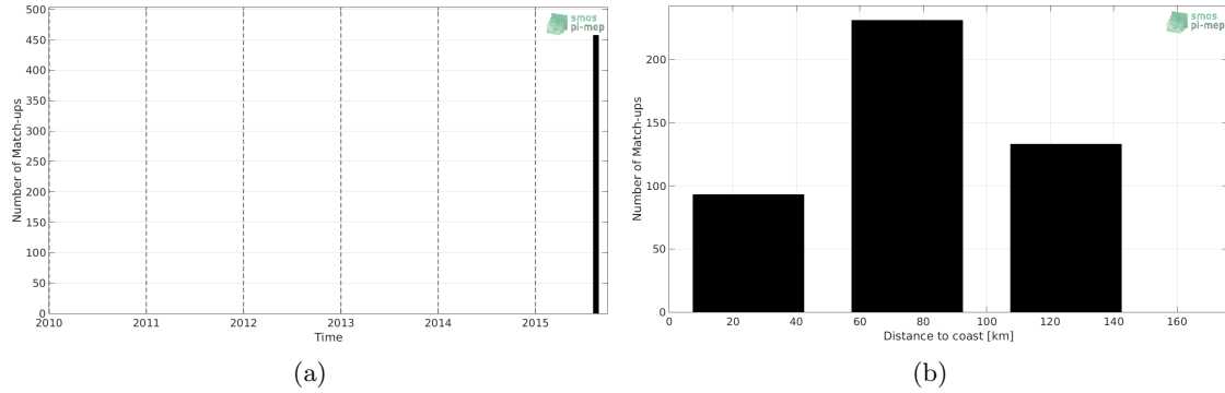
Figure 1: Number of match-ups between TSG-GOSUD-Sailing-ship and SMAP-L3-RSS-V3-8DAY-RUNNING-40KM SSS as a function of time (a) and as function of the distance to coast (b) over the Arctic Ocean Pi-MEP region and for the full satellite product period.
