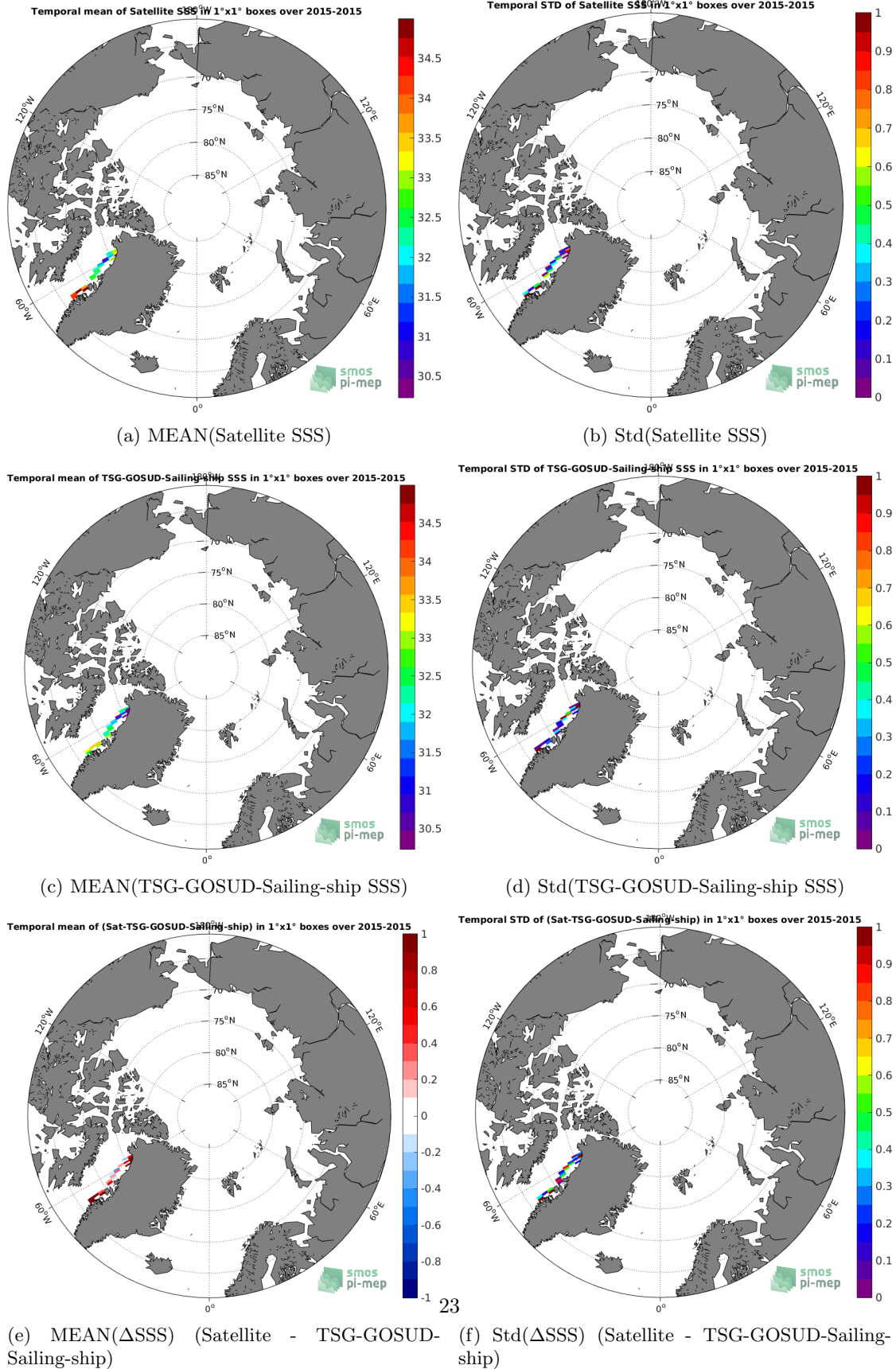
Figure 6: Temporal mean (left) and Std (right) of SSS from SMAP-L3-RSS-V3-8DAY-RUNNING-40KM (top), TSG-GOSUD-Sailing-ship (middle), and of \Delta SSS (Satellite - TSG-GOSUD-Sailing-ship). Only match-up pairs are used to generate these maps.
