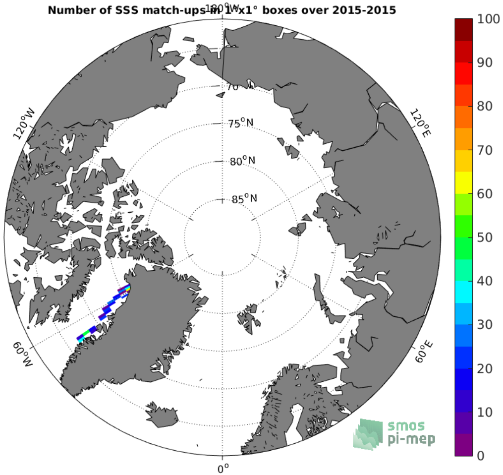
Figure 4: Number of SSS match-ups between TSG-GOSUD-Sailing-ship SSS and the SMAP-L3-RSS-V3-8DAY-RUNNING-40KM SSS product for the Arctic Ocean Pi-MEP region over 1°x1° boxes and for the full satellite product period.
