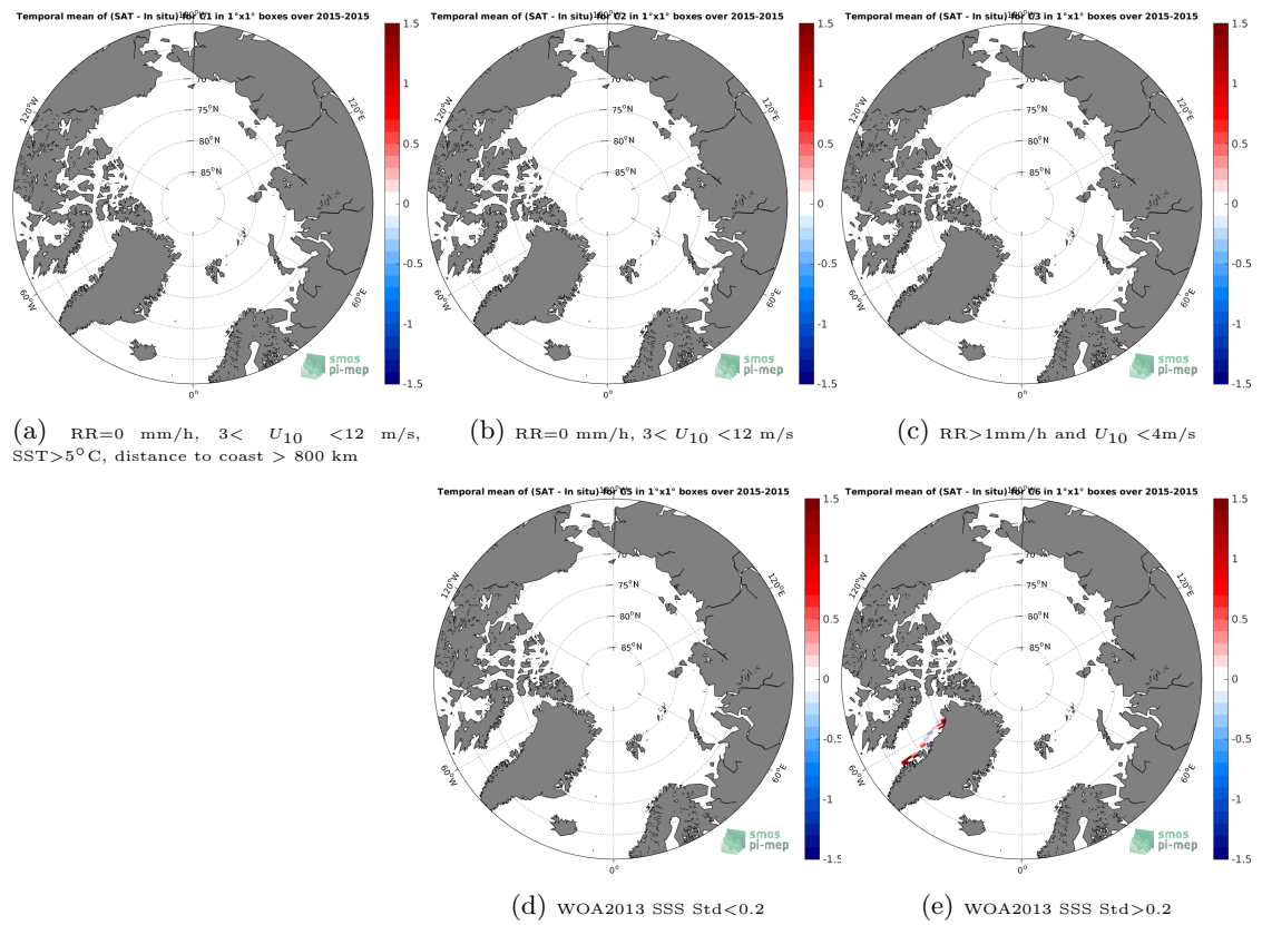
Figure 12: Temporal mean gridded over spatial boxes of size 1^\circ \times 1^\circ of \Delta SSS (SMAP-L3-RSS-V3-8DAY-RUNNING-40KM - TSG-GOSUD-Sailing-ship) for 5 different subdatasets corresponding to:RR=0 mm/h, 3 < U_{10} < 12 m/s, SST > 5^\circ\text{C} , distance to coast > 800 km (a), RR=0 mm/h, 3 < U_{10} < 12 m/s (b), RR > 1 mm/h and U_{10} < 4 m/s (c), WOA2013 SSS Std < 0.2 (d), WOA2013 SSS Std > 0.2 (e).
