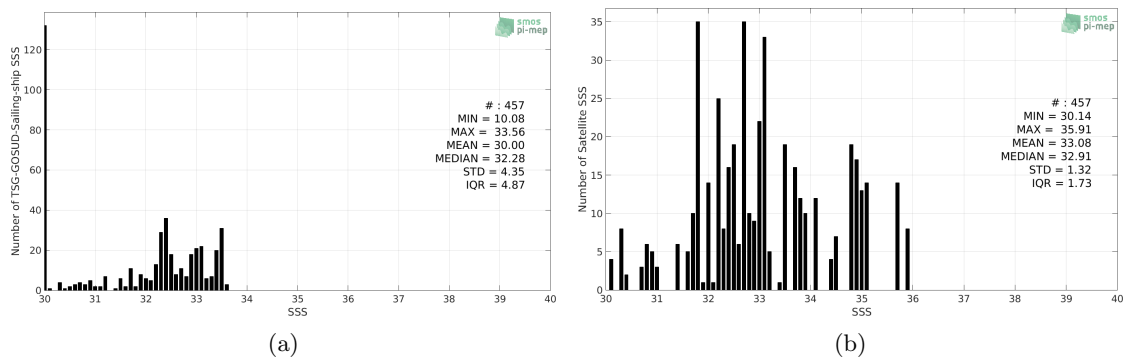
Figure 2: Histograms of SSS from TSG-GOSUD-Sailing-ship (a) and SMAP-L3-RSS-V3-8DAY-RUNNING-40KM (b) considering all match-up pairs per bins of 0.1 over the Arctic Ocean Pi-MEP region and for the full satellite product period.
