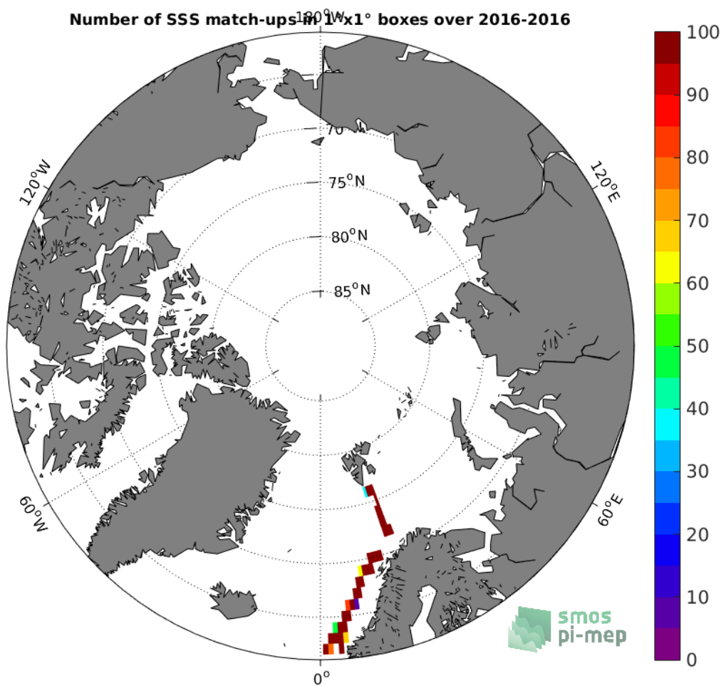
Figure 4: Number of SSS match-ups between TSG-GOSUD-Research-vessel SSS and the SMAP-L3-RSS-V3-8DAY-RUNNING-40KM SSS product for the Arctic Ocean Pi-MEP region over 1^\circ \times 1^\circ boxes and for the full satellite product period.
