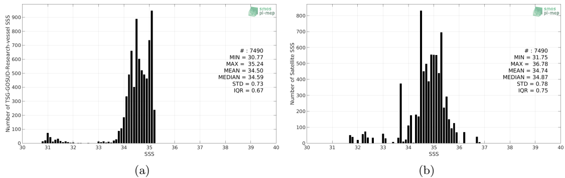
Figure 2: Histograms of SSS from TSG-GOSUD-Research-vessel (a) and SMAP-L3-RSS-V3-8DAY-RUNNING-40KM (b) considering all match-up pairs per bins of 0.1 over the Arctic Ocean Pi-MEP region and for the full satellite product period.
