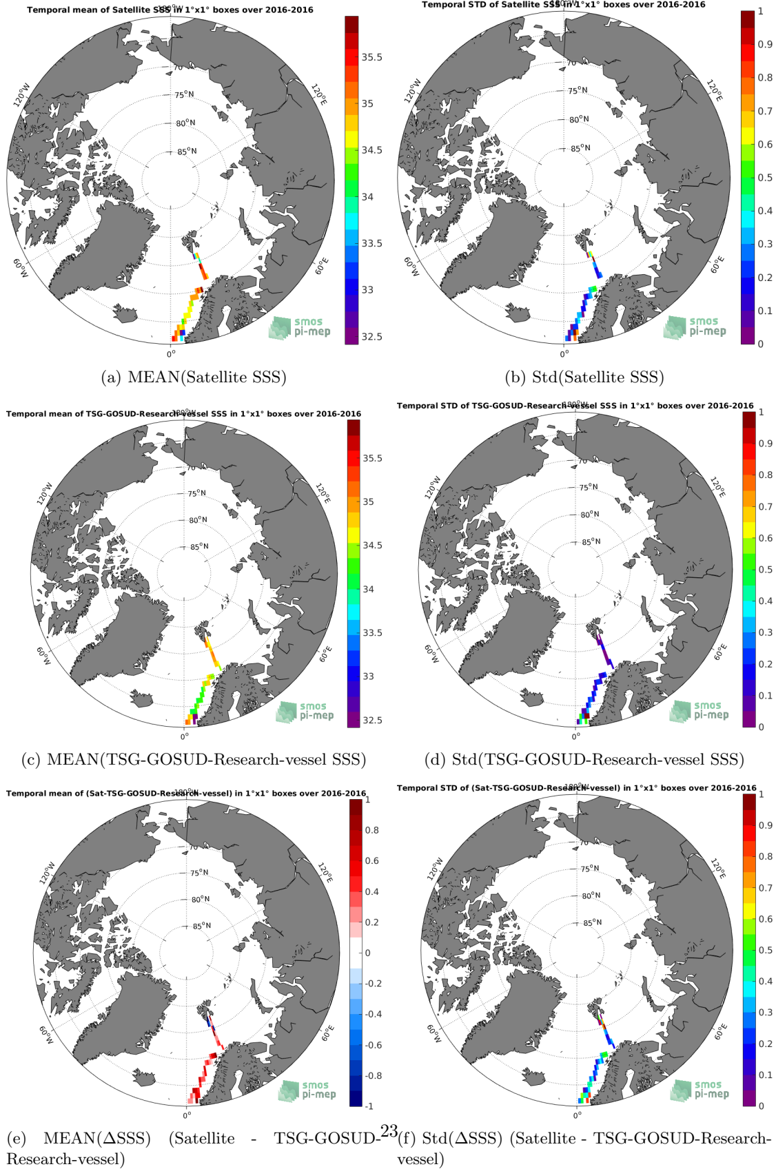
Figure 6: Temporal mean (left) and Std (right) of SSS from SMAP-L3-RSS-V3-8DAY-RUNNING-40KM (top), TSG-GOSUD-Research-vessel (middle), and of \Delta SSS (Satellite - TSG-GOSUD-Research-vessel). Only match-up pairs are used to generate these maps.
