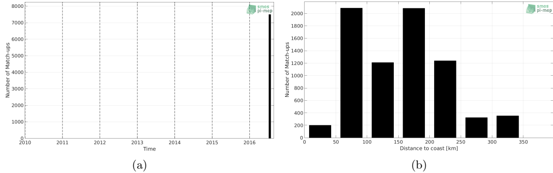
Figure 1: Number of match-ups between TSG-GOSUD-Research-vessel and SMAP-L3-RSS-V3-8DAY-RUNNING-40KM SSS as a function of time (a) and as function of the distance to coast (b) over the Arctic Ocean Pi-MEP region and for the full satellite product period.
