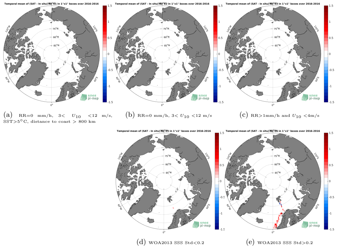
Figure 12: Temporal mean gridded over spatial boxes of size 1^\circ \times 1^\circ of \Delta SSS (SMAP-L3-RSS-V3-8DAY-RUNNING-40KM - TSG-GOSUD-Research-vessel) for 5 different subdatasets corresponding to:RR=0 mm/h, 3 < U_{10} < 12 m/s, SST > 5^\circ\text{C} , distance to coast > 800 km (a), RR=0 mm/h, 3 < U_{10} < 12 m/s (b), RR > 1 mm/h and U_{10} < 4 m/s (c), WOA2013 SSS Std < 0.2 (d), WOA2013 SSS Std > 0.2 (e).
