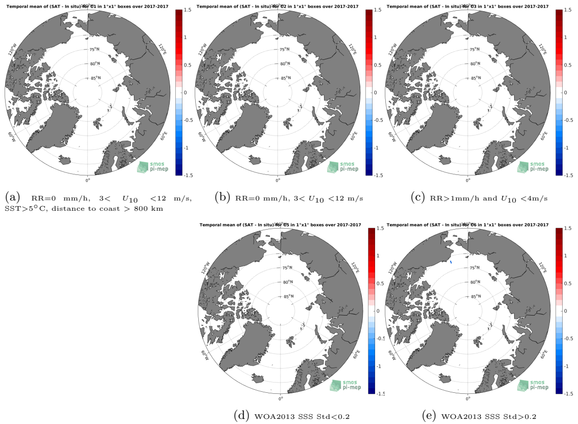
Figure 11: Temporal mean gridded over spatial boxes of size 1^\circ \times 1^\circ of \Delta SSS (SMAP-L3-RSS-V3-8DAY-RUNNING-40KM - Surface drifters) for 5 different subdatasets corresponding to: RR=0 mm/h, 3 < U_{10} < 12 m/s, SST > 5^\circ C , distance to coast > 800 km (a), RR=0 mm/h, 3 < U_{10} < 12 m/s (b), RR > 1 mm/h and U_{10} < 4 m/s (c), WOA2013 SSS Std < 0.2 (d), WOA2013 SSS Std > 0.2 (e).
