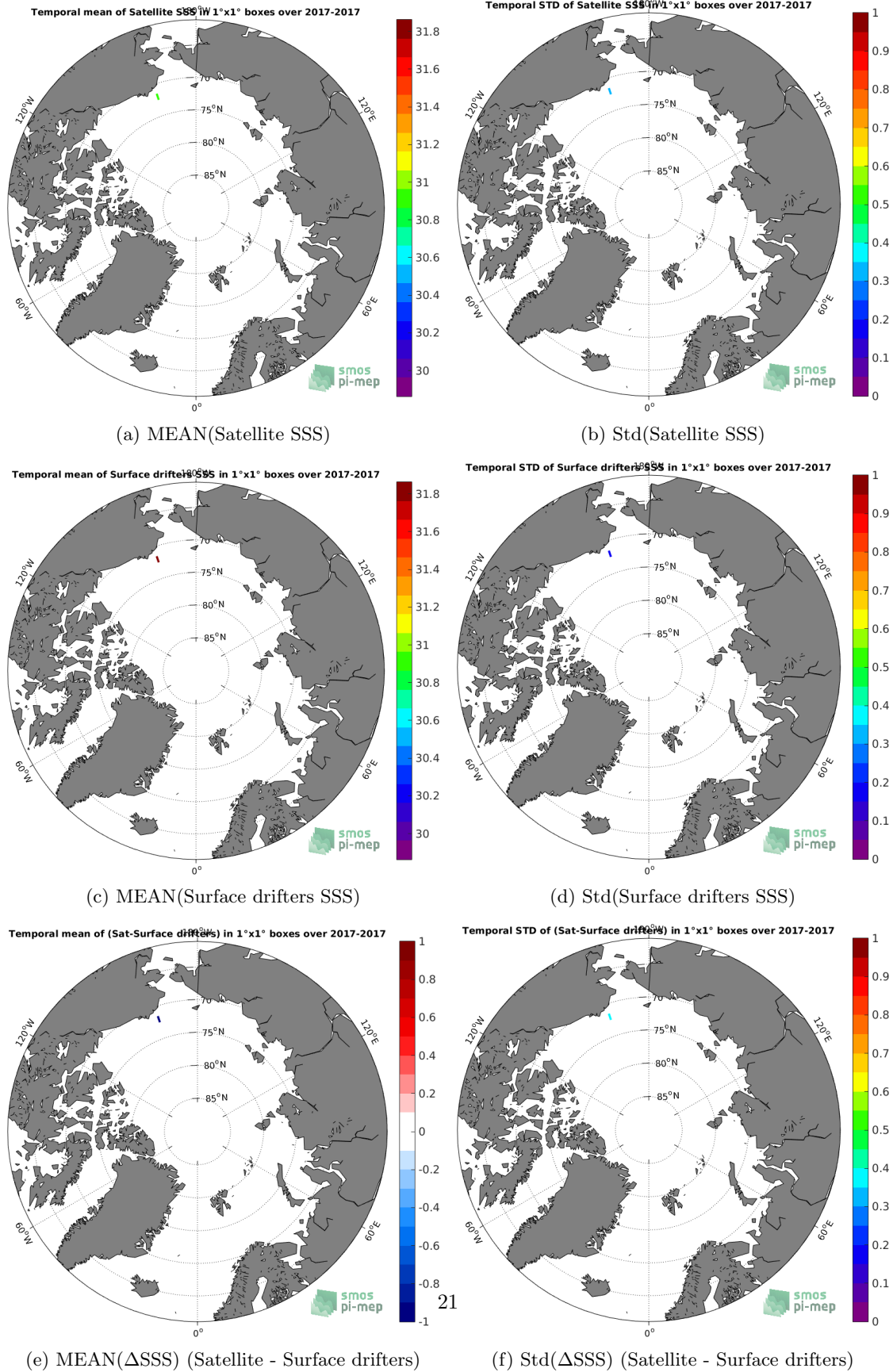
Figure 5: Temporal mean (left) and Std (right) of SSS from SMAP-L3-RSS-V3-8DAY-RUNNING-40KM (top), Surface drifters (middle), and of \Delta SSS (Satellite - Surface drifters). Only match-up pairs are used to generate these maps.
