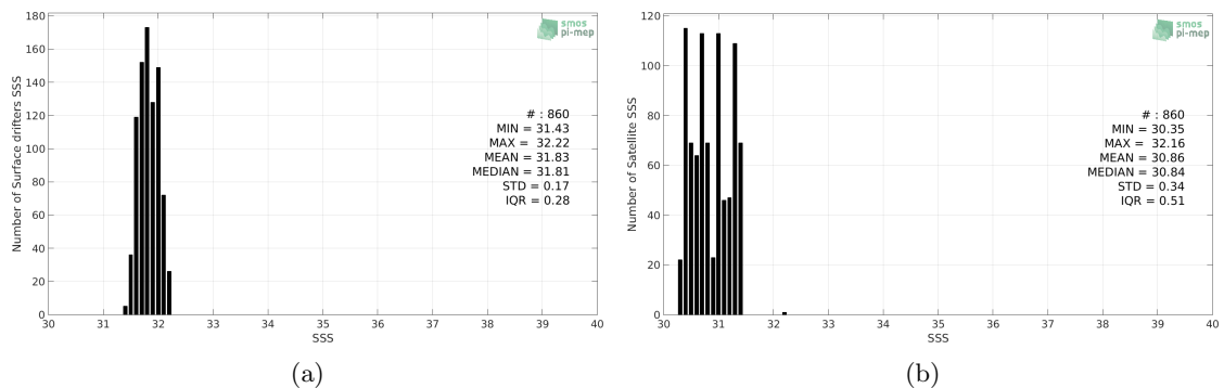
Figure 2: Histograms of SSS from Surface drifters (a) and SMAP-L3-RSS-V3-8DAY-RUNNING-40KM (b) considering all match-up pairs per bins of 0.1 over the Arctic Ocean Pi-MEP region and for the full satellite product period.
