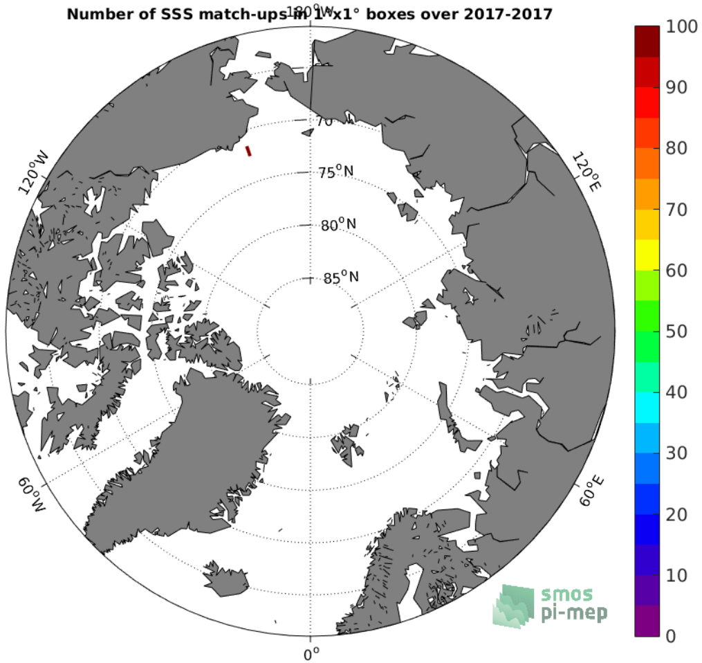
Figure 3: Number of SSS match-ups between Surface drifters SSS and the SMAP-L3-RSS-V3-8DAY-RUNNING-40KM SSS product for the Arctic Ocean Pi-MEP region over 1°x1° boxes and for the full satellite product period.
