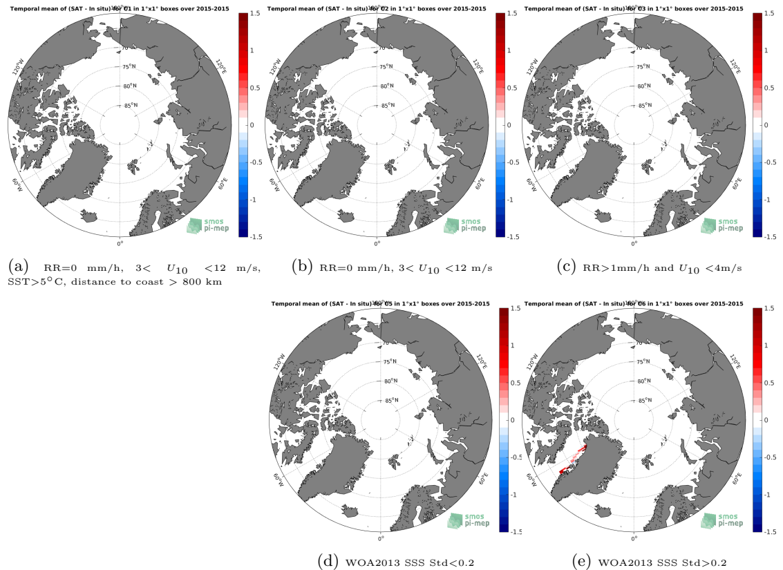
Figure 12: Temporal mean gridded over spatial boxes of size 1^\circ \times 1^\circ of \Delta SSS (SMAP-L3-RSS-V3-MONTHLY-0.25DEG-40KM - TSG-GOSUD-Sailing-ship) for 5 different subdatasets corresponding to:RR=0 mm/h, 3 < U_{10} < 12 m/s, SST >5^\circ C, distance to coast > 800 km (a), RR=0 mm/h, 3 < U_{10} < 12 m/s (b), RR >1 mm/h and U_{10} < 4 m/s (c), WOA2013 SSS Std <0.2 (d), WOA2013 SSS Std >0.2 (e).
