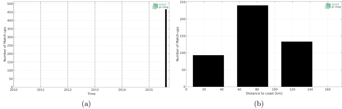
Figure 1: Number of match-ups between TSG-GOSUD-Sailing-ship and SMAP-L3-RSS-V3-MONTHLY-0.25DEG-40KM SSS as a function of time (a) and as function of the distance to coast (b) over the Arctic Ocean Pi-MEP region and for the full satellite product period.
