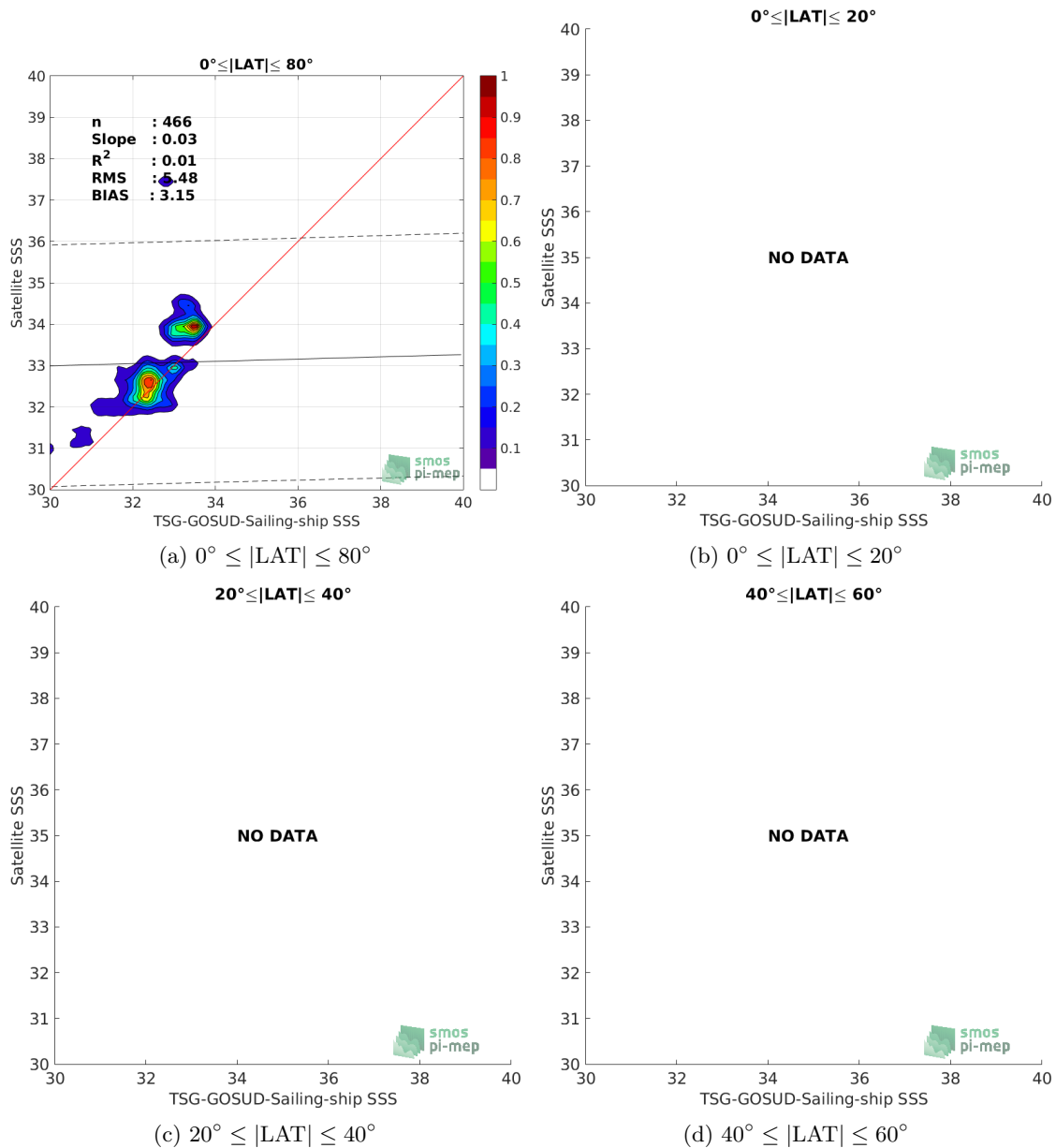
Figure 9: Contour maps of the concentration of SMAP-L3-RSS-V3-MONTHLY-0.25DEG-40KM SSS (y-axis) versus TSG-GOSUD-Sailing-ship SSS (x-axis) at match-up pairs for different latitude bands. For each plot, the red line shows x=y . The black thin and dashed lines indicate a linear fit through the data cloud and the \pm 95\% confidence levels, respectively. The number match-up pairs n , the slope and R^2 coefficient of the linear fit, the root mean square (RMS) and the mean bias between satellite and in situ data are indicated for each latitude band in each plots.
