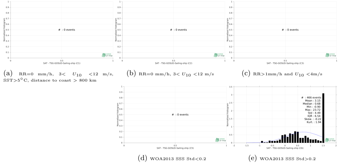
Figure 13: Normalized histogram of \Delta\text{SSS} (SMAP-L3-RSS-V3-MONTHLY-0.25DEG-40KM - TSG-GOSUD-Sailing-ship) for 5 different subdatasets corresponding to: RR=0 mm/h, 3 < U_{10} < 12 m/s, SST > 5^{\circ}\text{C} , distance to coast > 800 km (a), RR=0 mm/h, 3 < U_{10} < 12 m/s (b), RR > 1\text{mm/h} and U_{10} < 4\text{m/s} (c), WOA2013 SSS Std < 0.2 (d), WOA2013 SSS Std > 0.2 (e).
