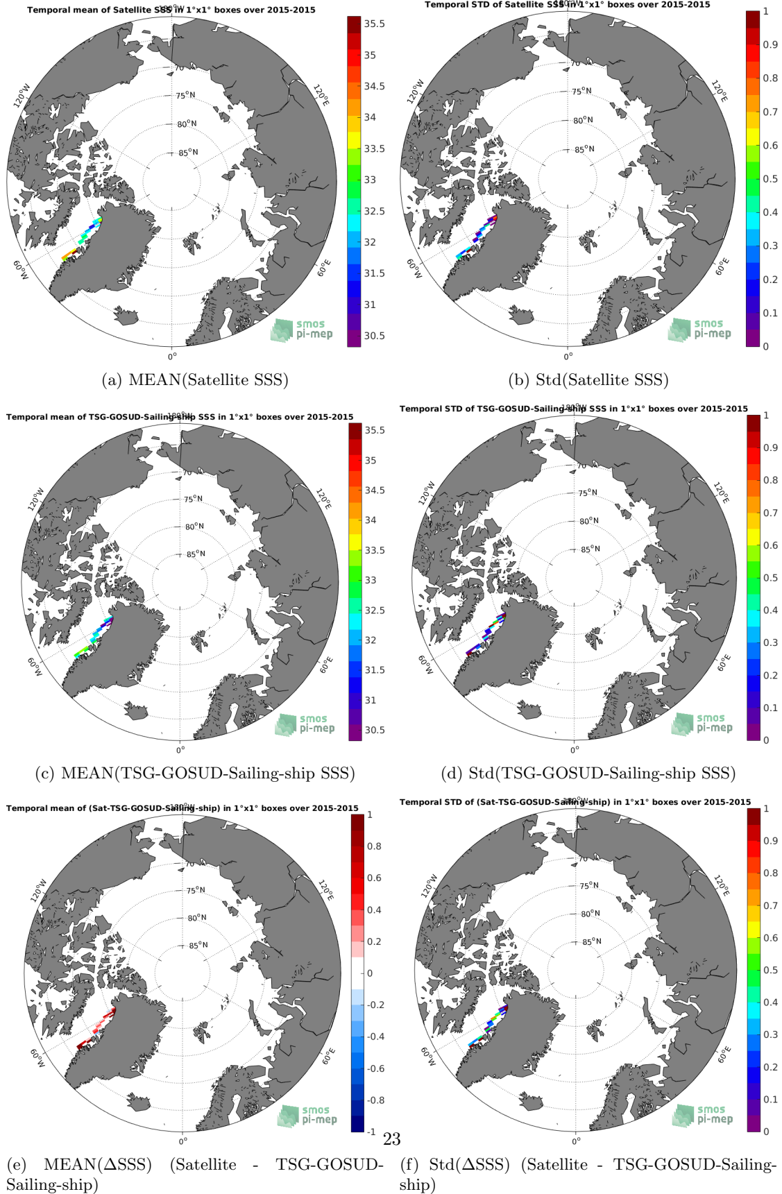
Figure 6: Temporal mean (left) and Std (right) of SSS from SMAP-L3-RSS-V3-MONTHLY-0.25DEG-40KM (top), TSG-GOSUD-Sailing-ship (middle), and of \Delta SSS (Satellite - TSG-GOSUD-Sailing-ship). Only match-up pairs are used to generate these maps.
