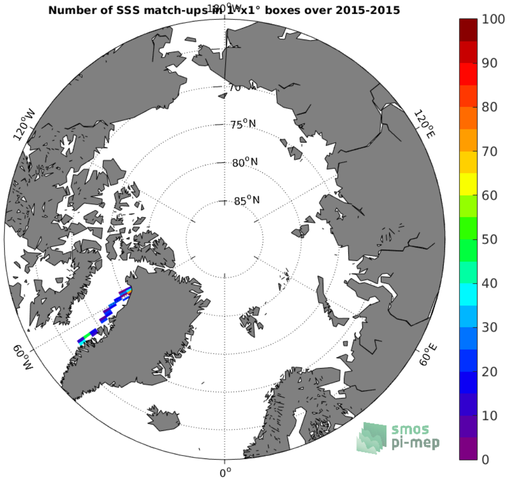
Figure 4: Number of SSS match-ups between TSG-GOSUD-Sailing-ship SSS and the SMAP-L3-RSS-V3-MONTHLY-0.25DEG-40KM SSS product for the Arctic Ocean Pi-MEP region over 1^\circ \times 1^\circ boxes and for the full satellite product period.
