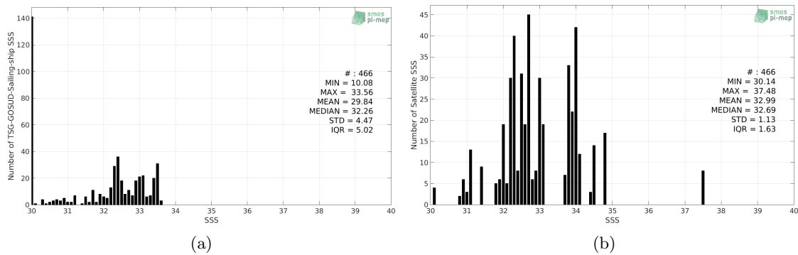
Figure 2: Histograms of SSS from TSG-GOSUD-Sailing-ship (a) and SMAP-L3-RSS-V3-MONTHLY-0.25DEG-40KM (b) considering all match-up pairs per bins of 0.1 over the Arctic Ocean Pi-MEP region and for the full satellite product period.
