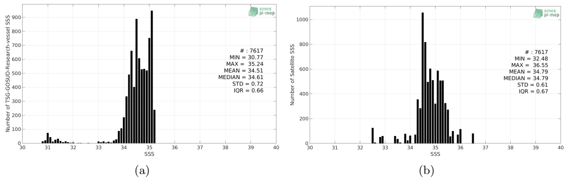
Figure 2: Histograms of SSS from TSG-GOSUD-Research-vessel (a) and SMAP-L3-RSS-V3-MONTHLY-0.25DEG-40KM (b) considering all match-up pairs per bins of 0.1 over the Arctic Ocean Pi-MEP region and for the full satellite product period.
