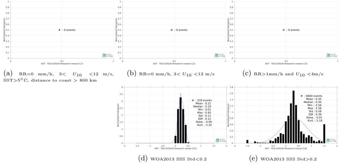
Figure 13: Normalized histogram of \Delta SSS (SMAP-L3-RSS-V3-MONTHLY-0.25DEG-40KM - TSG-GOSUD-Research-vessel) for 5 different subdatasets corresponding to: RR=0 mm/h, 3 < U_{10} < 12 m/s, SST > 5°C, distance to coast > 800 km (a), RR=0 mm/h, 3 < U_{10} < 12 m/s (b), RR > 1mm/h and U_{10} < 4 m/s (c), WOA2013 SSS Std < 0.2 (d), WOA2013 SSS Std > 0.2 (e).
