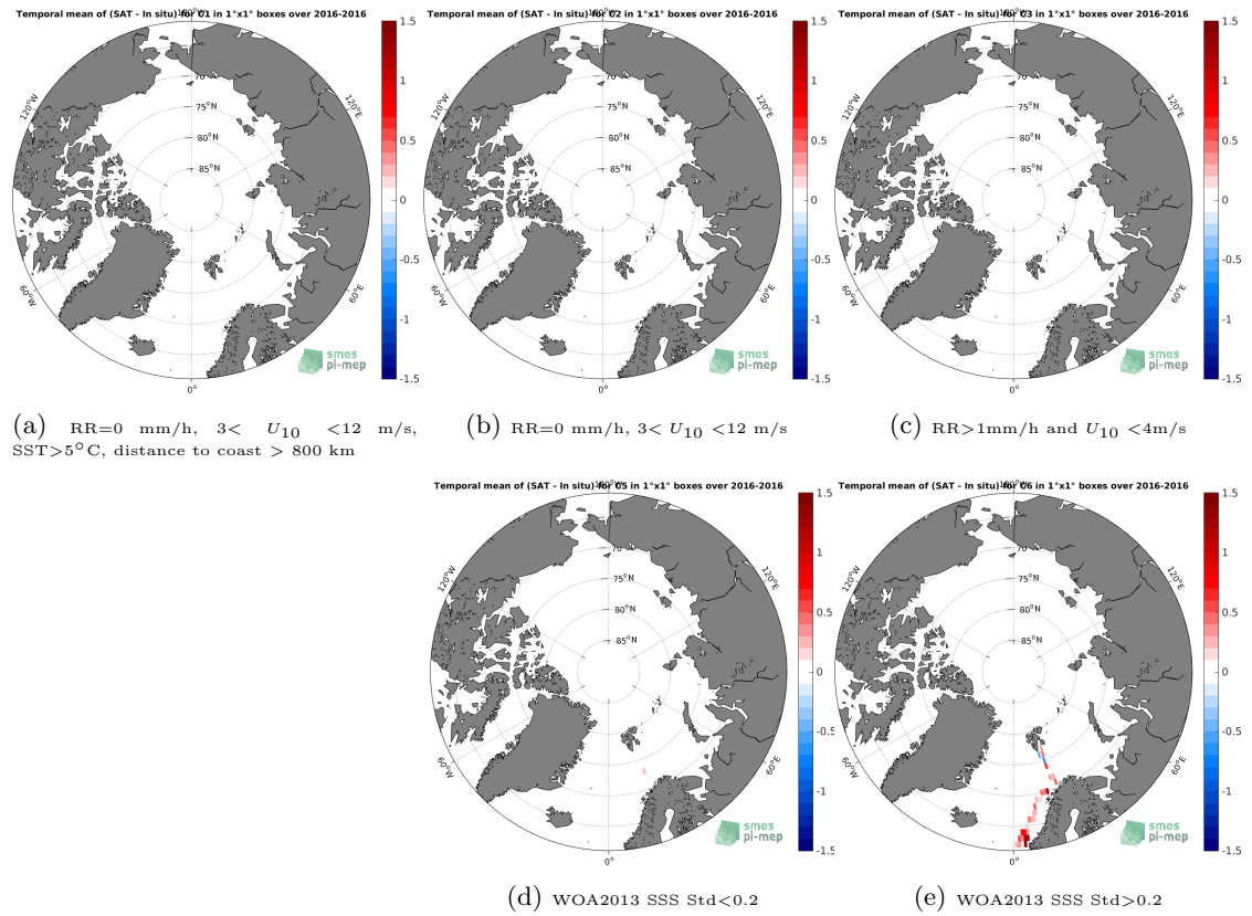
Figure 12: Temporal mean gridded over spatial boxes of size 1^\circ \times 1^\circ of \Delta SSS (SMAP-L3-RSS-V3-MONTHLY-0.25DEG-40KM - TSG-GOSUD-Research-vessel) for 5 different subdatasets corresponding to:RR=0 mm/h, 3 < U_{10} < 12 m/s, SST > 5^\circ\text{C} , distance to coast > 800 km (a), RR=0 mm/h, 3 < U_{10} < 12 m/s (b), RR > 1 mm/h and U_{10} < 4 m/s (c), WOA2013 SSS Std < 0.2 (d), WOA2013 SSS Std > 0.2 (e).
