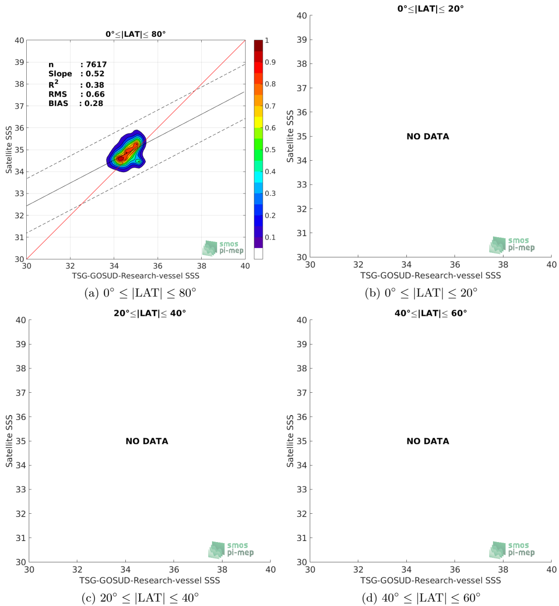
Figure 9: Contour maps of the concentration of SMAP-L3-RSS-V3-MONTHLY-0.25DEG-40KM SSS (y-axis) versus TSG-GOSUD-Research-vessel SSS (x-axis) at match-up pairs for different latitude bands. For each plot, the red line shows x=y . The black thin and dashed lines indicate a linear fit through the data cloud and the \pm 95\% confidence levels, respectively. The number match-up pairs n , the slope and R^2 coefficient of the linear fit, the root mean square (RMS) and the mean bias between satellite and in situ data are indicated for each latitude band in each plots.
