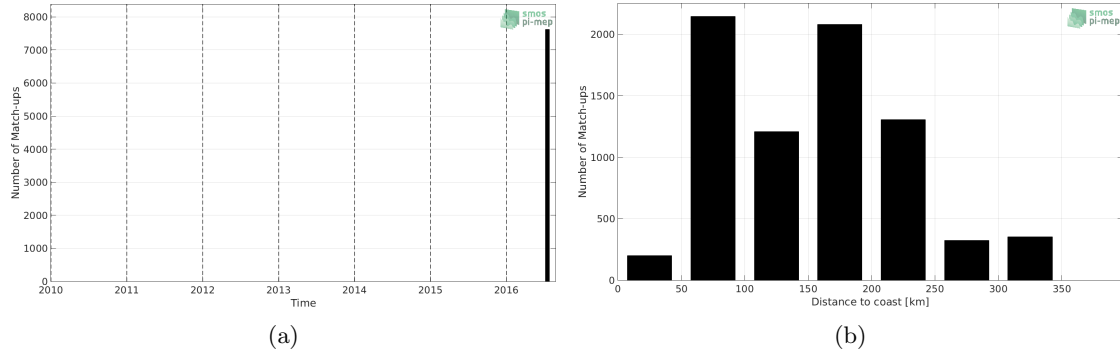
Figure 1: Number of match-ups between TSG-GOSUD-Research-vessel and SMAP-L3-RSS-V3-MONTHLY-0.25DEG-40KM SSS as a function of time (a) and as function of the distance to coast (b) over the Arctic Ocean Pi-MEP region and for the full satellite product period.
