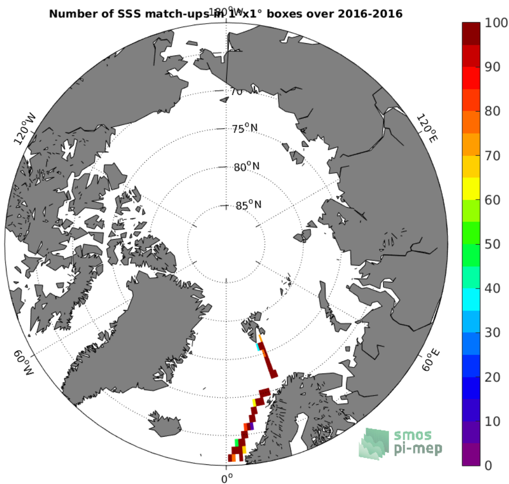
Figure 4: Number of SSS match-ups between TSG-GOSUD-Research-vessel SSS and the SMAP-L3-RSS-V3-MONTHLY-0.25DEG-40KM SSS product for the Arctic Ocean Pi-MEP region over 1°x1° boxes and for the full satellite product period.
