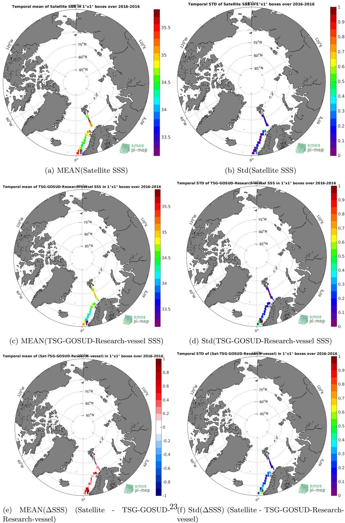
Figure 6: Temporal mean (left) and Std (right) of SSS from SMAP-L3-RSS-V3-MONTHLY-0.25DEG-40KM (top), TSG-GOSUD-Research-vessel (middle), and of \Delta SSS (Satellite - TSG-GOSUD-Research-vessel). Only match-up pairs are used to generate these maps.
