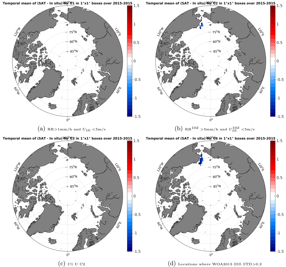
Figure 12: Temporal mean gridded over spatial boxes of size 1°x1° of \Delta SSS (SMAP-L3-RSS-V2-8DAY-RUNNING-70KM - TSG-SAMOS) for 4 different subdatasets corresponding to:RR>1mm/h and U_{10} < 5\text{m/s} (a), RR^{10d} > 5\text{mm/h} and U_{10}^{10d} < 5\text{m/s} (b), C1 U C2 (c),Locations where WOA2013 SSS STD>0.2 (d).
