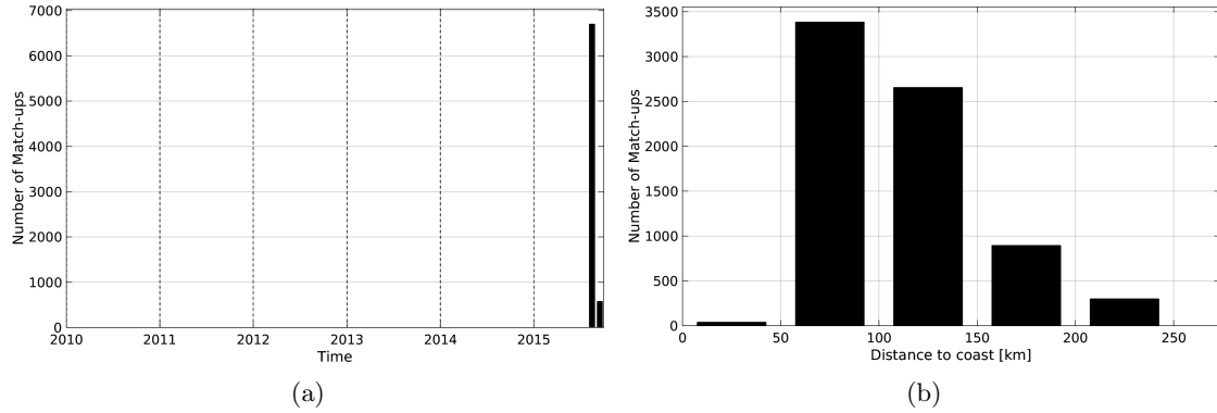
Figure 1: Number of match-ups between TSG-SAMOS and SMAP-L3-RSS-V2-8DAY-RUNNING-70KM SSS as a function of time (a) and as function of the distance to coast (b) over the Arctic Ocean Pi-MEP region and for the full satellite product period.
