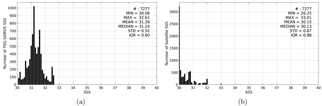
Figure 2: Histograms of SSS from TSG-SAMOS (a) and SMAP-L3-RSS-V2-8DAY-RUNNING-70KM (b) considering all match-up pairs per bins of 0.1 over the Arctic Ocean Pi-MEP region and for the full satellite product period.
