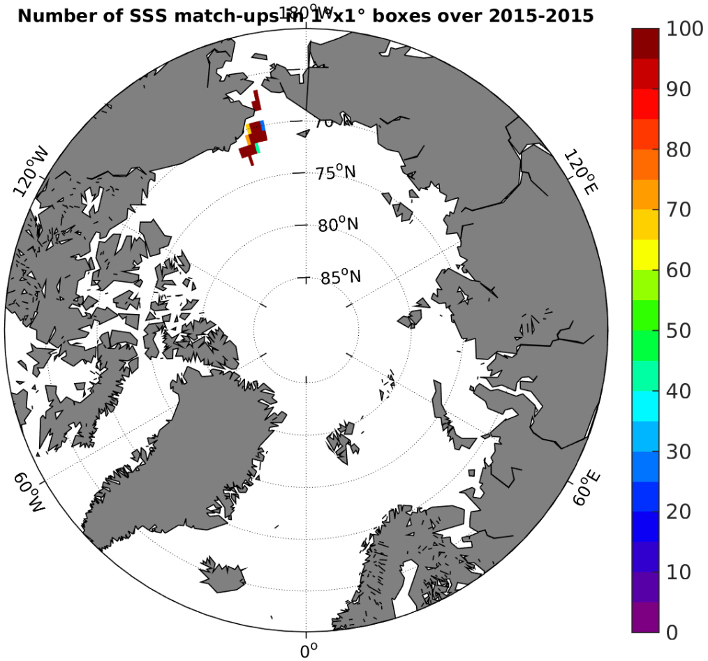
Figure 4: Number of SSS match-ups between TSG-SAMOS SSS and the SMAP-L3-RSS-V2-8DAY-RUNNING-70KM SSS product for the Arctic Ocean Pi-MEP region over 1°x1° boxes and for the full satellite product period.
