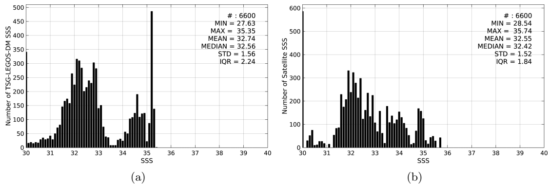
Figure 2: Histograms of SSS from TSG-LEGOS-DM (a) and SMAP-L3-RSS-V2-8DAY-RUNNING-70KM (b) considering all match-up pairs per bins of 0.1 over the Arctic Ocean Pi-MEP region and for the full satellite product period.
