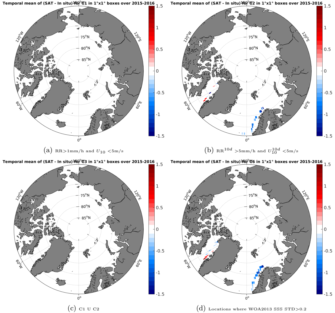
Figure 12: Temporal mean gridded over spatial boxes of size 1°x1° of \Delta SSS (SMAP-L3-RSS-V2-8DAY-RUNNING-70KM - TSG-LEGOS-DM) for 4 different subdatasets corresponding to: RR > 1mm/h and U_{10} < 5m/s (a), RR 10d > 5mm/h and U_{10}^{10d} < 5m/s (b), C1 U C2 (c), Locations where WOA2013 SSS STD > 0.2 (d).
