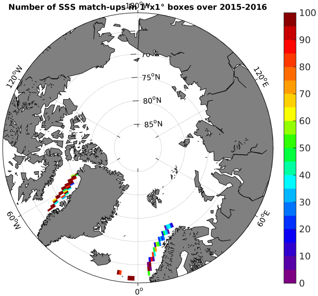
Figure 4: Number of SSS match-ups between TSG-LEGOS-DM SSS and the SMAP-L3-RSS-V2-8DAY-RUNNING-70KM SSS product for the Arctic Ocean Pi-MEP region over 1°x1° boxes and for the full satellite product period.
