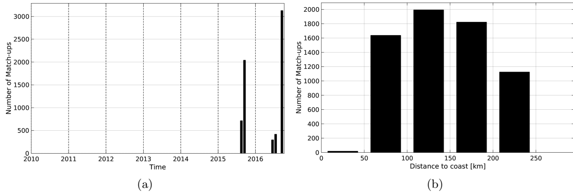
Figure 1: Number of match-ups between TSG-LEGOS-DM and SMAP-L3-RSS-V2-8DAY-RUNNING-70KM SSS as a function of time (a) and as function of the distance to coast (b) over the Arctic Ocean Pi-MEP region and for the full satellite product period.
