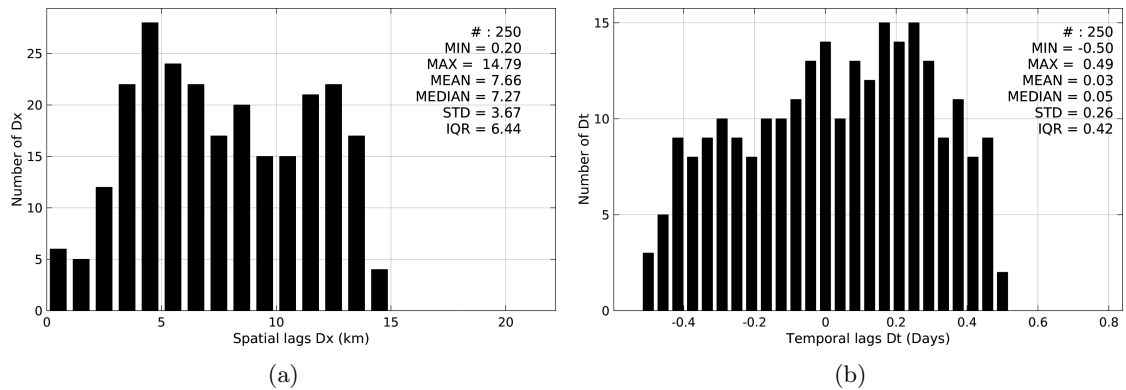
Figure 5: Histograms of the spatial (a) and temporal (b) lags between the time of the TSG-GOSUD-Sailing-ship measurements and the date of the corresponding SMAP-L3-RSS-V2-8DAY-RUNNING-70KM SSS product.
