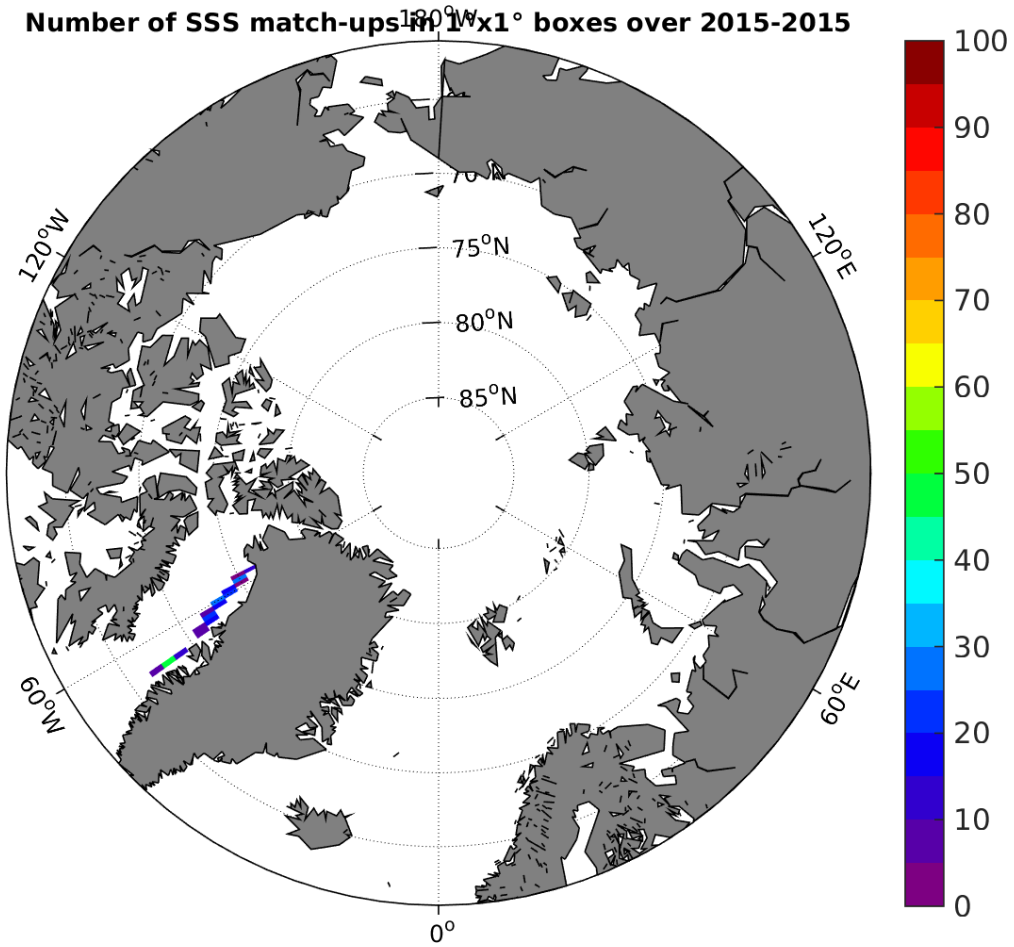
Figure 4: Number of SSS match-ups between TSG-GOSUD-Sailing-ship SSS and the SMAP-L3-RSS-V2-8DAY-RUNNING-70KM SSS product for the Arctic Ocean Pi-MEP region over 1°x1° boxes and for the full satellite product period.
