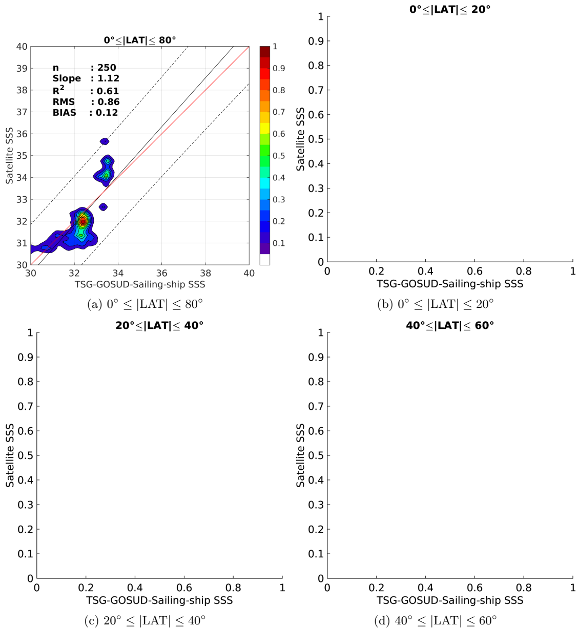
Figure 9: Contour maps of the concentration of SMAP-L3-RSS-V2-8DAY-RUNNING-70KM SSS (y-axis) versus TSG-GOSUD-Sailing-ship SSS (x-axis) at match-up pairs for different latitude bands. For each plot, the red line shows x=y . The black thin and dashed lines indicate a linear fit through the data cloud and the \pm 95\% confidence levels, respectively. The number match-up pairs n , the slope and R^2 coefficient of the linear fit, the root mean square (RMS) and the mean bias between satellite and in situ data are indicated for each latitude band in each plots.
