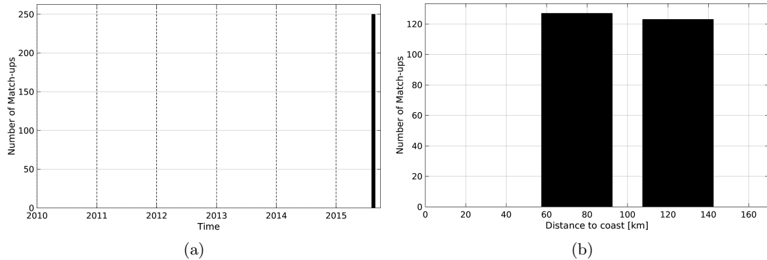
Figure 1: Number of match-ups between TSG-GOSUD-Sailing-ship and SMAP-L3-RSS-V2-8DAY-RUNNING-70KM SSS as a function of time (a) and as function of the distance to coast (b) over the Arctic Ocean Pi-MEP region and for the full satellite product period.
