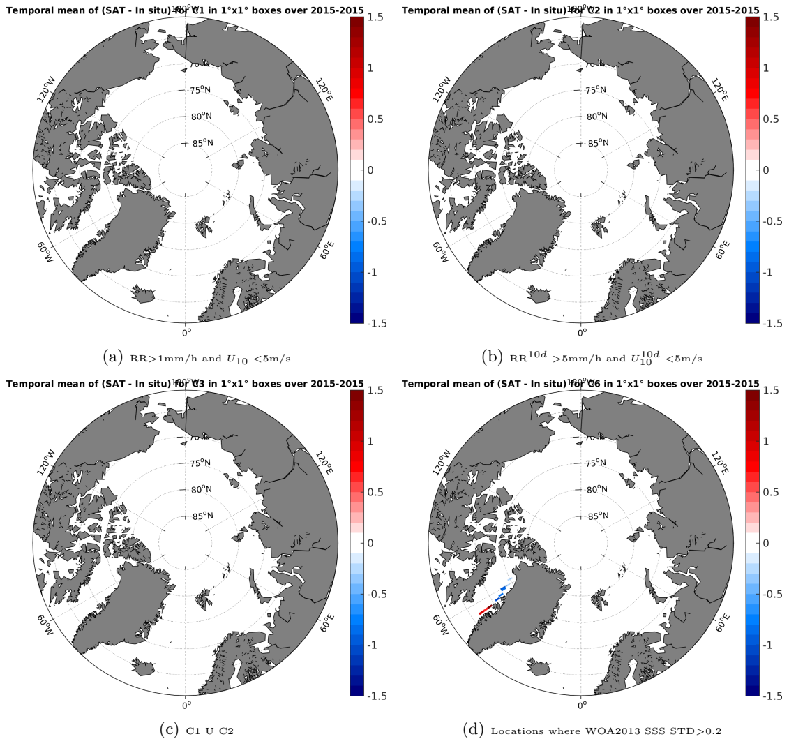
Figure 12: Temporal mean gridded over spatial boxes of size 1^\circ \times 1^\circ of \Delta SSS (SMAP-L3-RSS-V2-8DAY-RUNNING-70KM - TSG-GOSUD-Sailing-ship) for 4 different subdatasets corresponding to:RR > 1 mm/h and U_{10} < 5 m/s (a), RR^{10d} > 5 mm/h and U_{10}^{10d} < 5 m/s (b), C1 U C2 (c),Locations where WOA2013 SSS STD > 0.2 (d).
