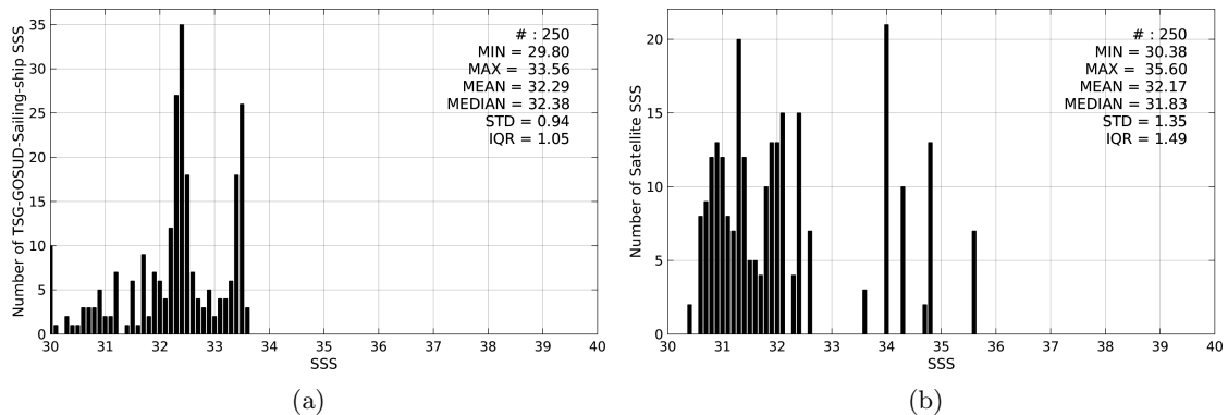
Figure 2: Histograms of SSS from TSG-GOSUD-Sailing-ship (a) and SMAP-L3-RSS-V2-8DAY-RUNNING-70KM (b) considering all match-up pairs per bins of 0.1 over the Arctic Ocean Pi-MEP region and for the full satellite product period.
