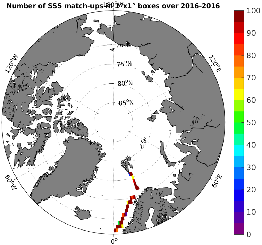
Figure 4: Number of SSS match-ups between TSG-GOSUD-Research-vessel SSS and the SMAP-L3-RSS-V2-8DAY-RUNNING-70KM SSS product for the Arctic Ocean Pi-MEP region over 1°x1° boxes and for the full satellite product period.
