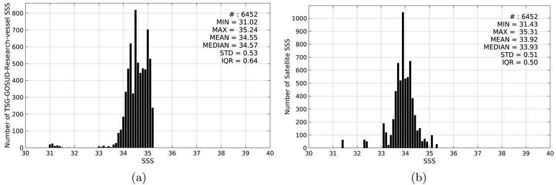
Figure 2: Histograms of SSS from TSG-GOSUD-Research-vessel (a) and SMAP-L3-RSS-V2-8DAY-RUNNING-70KM (b) considering all match-up pairs per bins of 0.1 over the Arctic Ocean Pi-MEP region and for the full satellite product period.
