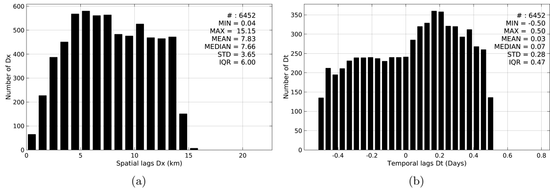
Figure 5: Histograms of the spatial (a) and temporal (b) lags between the time of the TSG-GOSUD-Research-vessel measurements and the date of the corresponding SMAP-L3-RSS-V2-8DAY-RUNNING-70KM SSS product.
