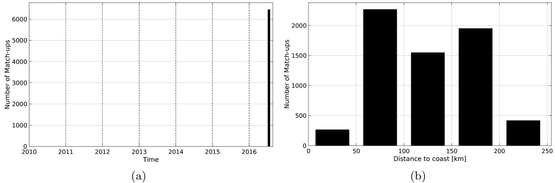
Figure 1: Number of match-ups between TSG-GOSUD-Research-vessel and SMAP-L3-RSS-V2-8DAY-RUNNING-70KM SSS as a function of time (a) and as function of the distance to coast (b) over the Arctic Ocean Pi-MEP region and for the full satellite product period.
