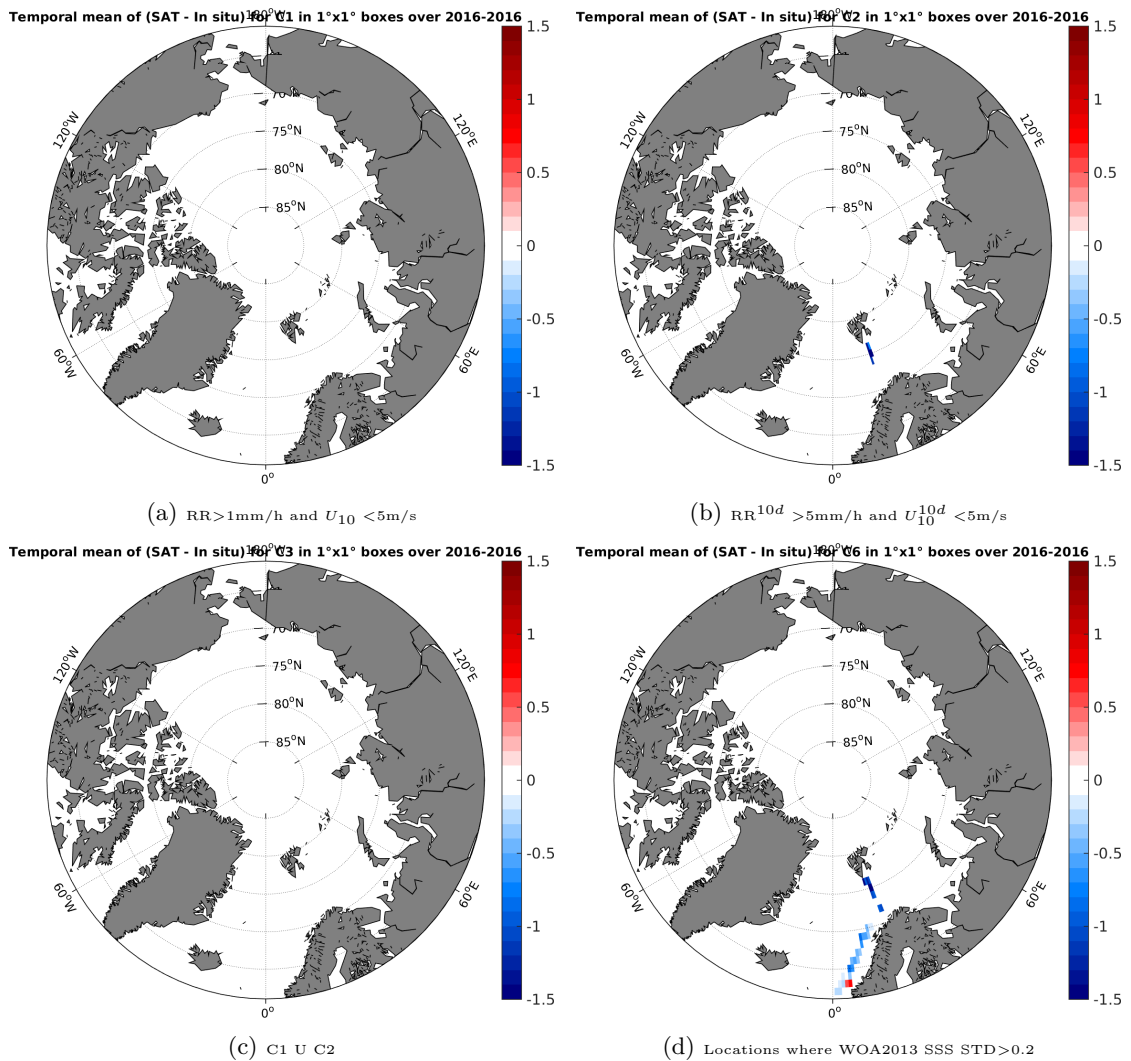
Figure 12: Temporal mean gridded over spatial boxes of size 1^\circ \times 1^\circ of \Delta SSS (SMAP-L3-RSS-V2-8DAY-RUNNING-70KM - TSG-GOSUD-Research-vessel) for 4 different subdatasets corresponding to:RR >1 mm/h and U_{10} < 5 m/s (a), RR^{10d} > 5 mm/h and U_{10}^{10d} < 5 m/s (b), C1 U C2 (c),Locations where WOA2013 SSS STD >0.2 (d).
