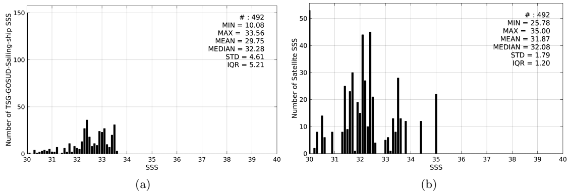
Figure 2: Histograms of SSS from TSG-GOSUD-Sailing-ship (a) and SMAP-L3-RSS-V2-MONTHLY-0.25DEG-40KM (b) considering all match-up pairs per bins of 0.1 over the Arctic Ocean Pi-MEP region and for the full satellite product period.
