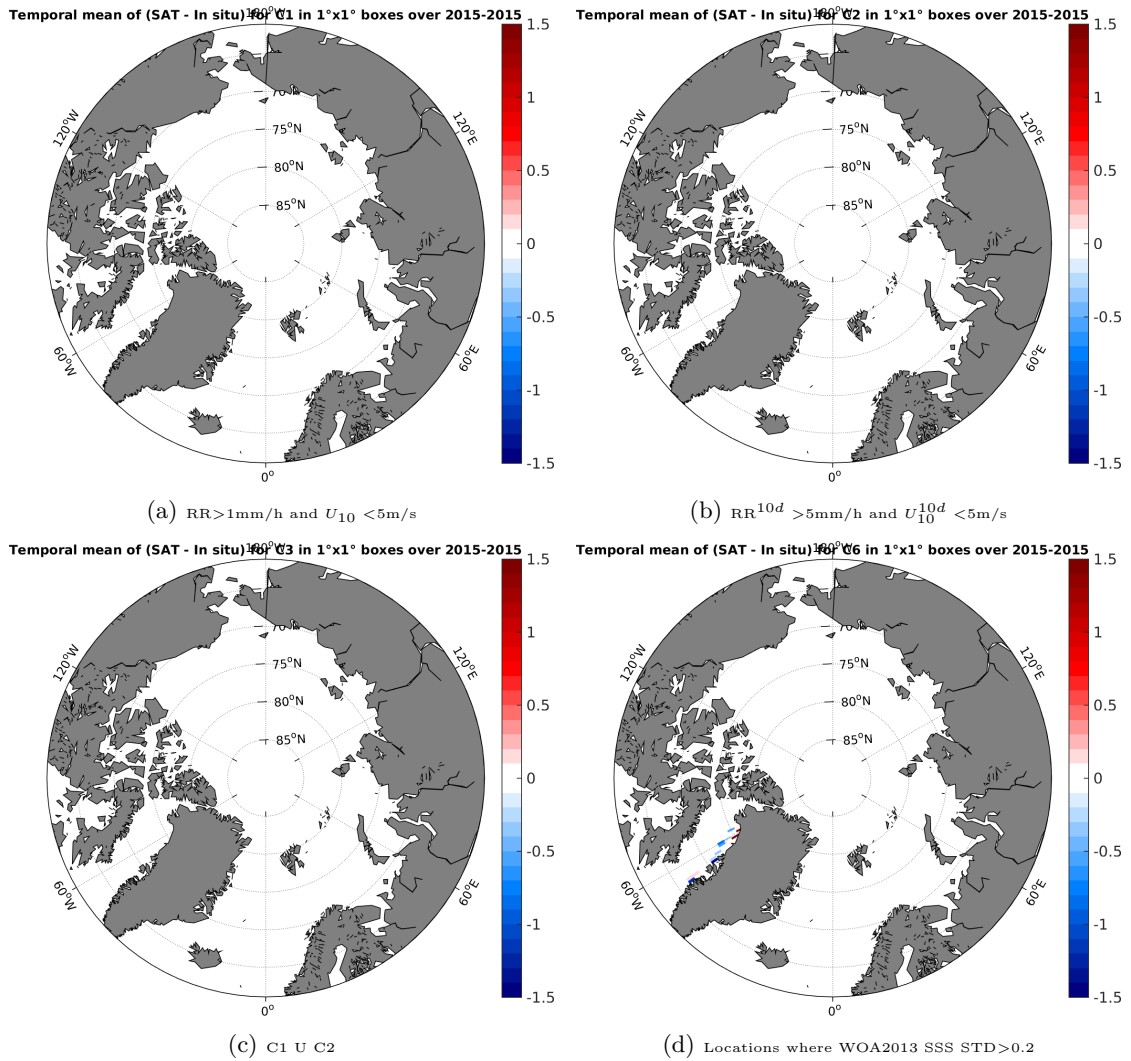
Figure 12: Temporal mean gridded over spatial boxes of size 1^\circ \times 1^\circ of \Delta SSS (SMAP-L3-RSS-V2-MONTHLY-0.25DEG-40KM - TSG-GOSUD-Sailing-ship) for 4 different subdatasets corresponding to:RR >1 mm/h and U_{10} < 5 m/s (a), RR^{10d} > 5 mm/h and U_{10}^{10d} < 5 m/s (b), C1 U C2 (c),Locations where WOA2013 SSS STD >0.2 (d).
