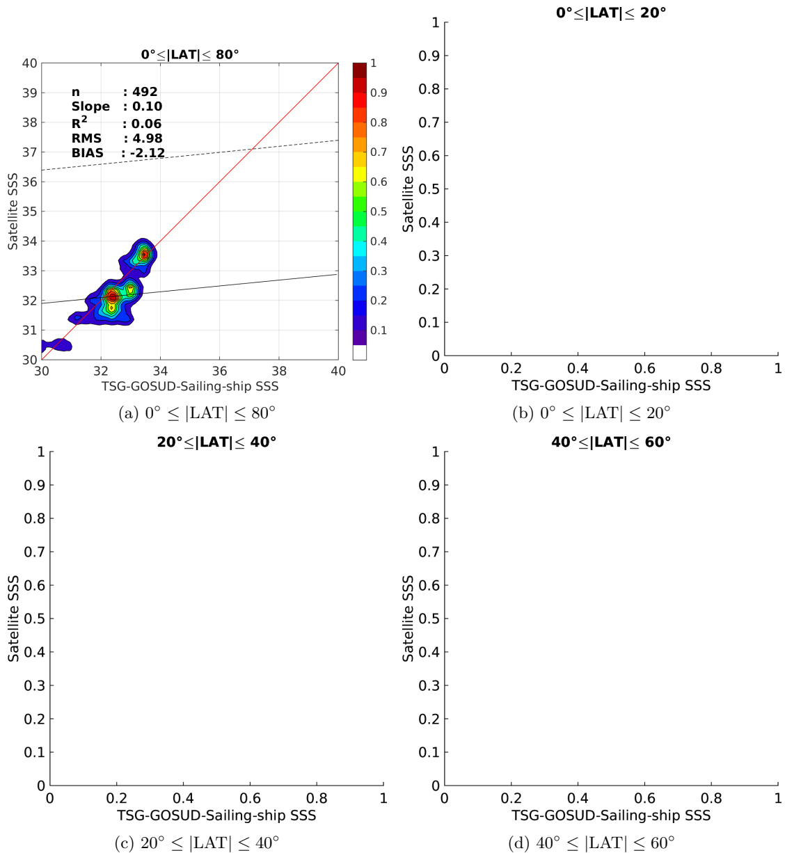
Figure 9: Contour maps of the concentration of SMAP-L3-RSS-V2-MONTHLY-0.25DEG-40KM SSS (y-axis) versus TSG-GOSUD-Sailing-ship SSS (x-axis) at match-up pairs for different latitude bands. For each plot, the red line shows x=y . The black thin and dashed lines indicate a linear fit through the data cloud and the \pm 95\% confidence levels, respectively. The number match-up pairs n , the slope and R^2 coefficient of the linear fit, the root mean square (RMS) and the mean bias between satellite and in situ data are indicated for each latitude band in each plots.
