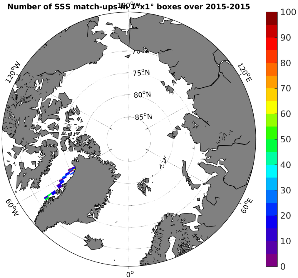
Figure 4: Number of SSS match-ups between TSG-GOSUD-Sailing-ship SSS and the SMAP-L3-RSS-V2-MONTHLY-0.25DEG-40KM SSS product for the Arctic Ocean Pi-MEP region over 1°x1° boxes and for the full satellite product period.
