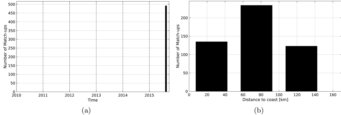
Figure 1: Number of match-ups between TSG-GOSUD-Sailing-ship and SMAP-L3-RSS-V2-MONTHLY-0.25DEG-40KM SSS as a function of time (a) and as function of the distance to coast (b) over the Arctic Ocean Pi-MEP region and for the full satellite product period.
