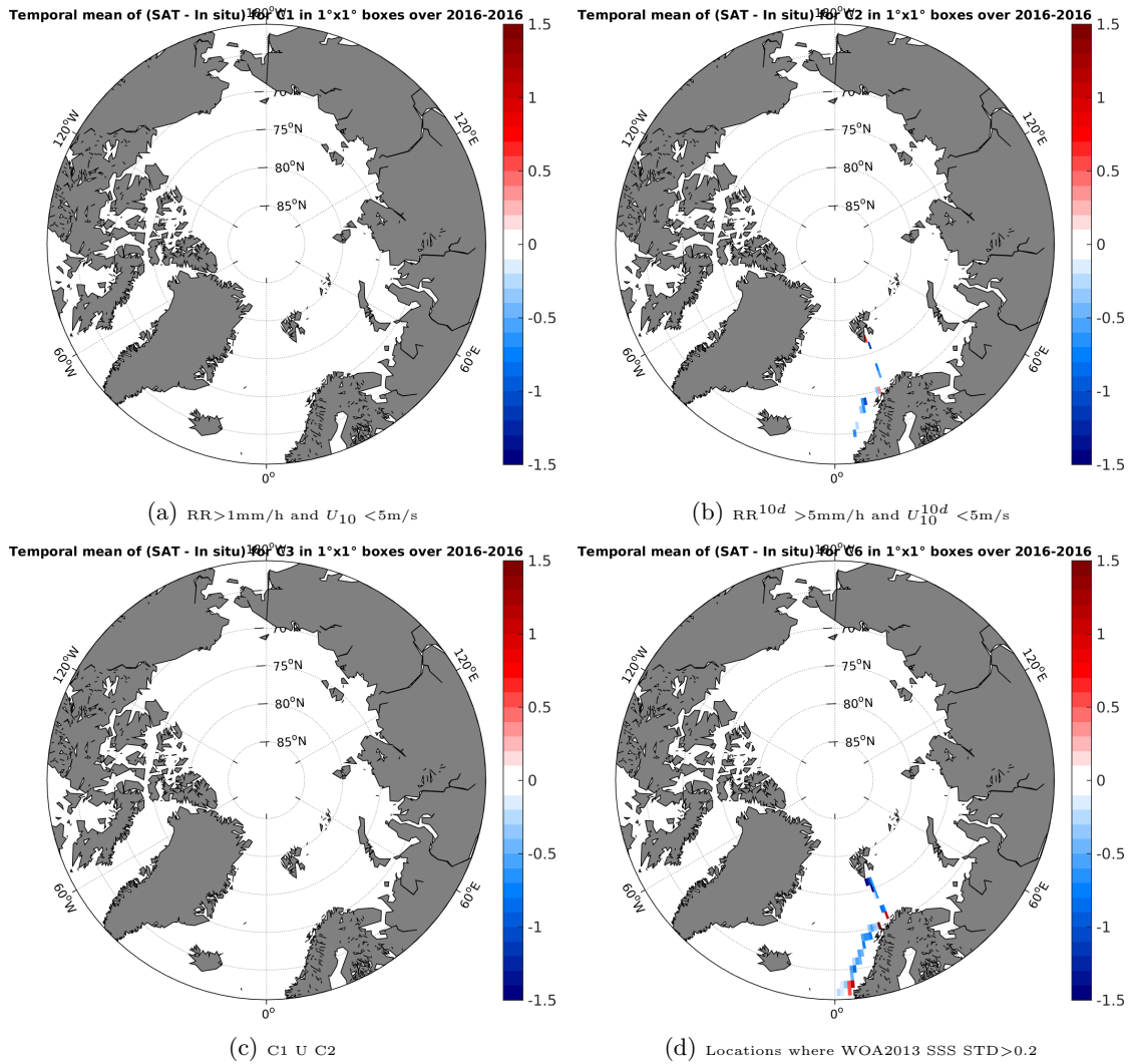
Figure 12: Temporal mean gridded over spatial boxes of size 1^\circ \times 1^\circ of \Delta SSS (SMAP-L3-RSS-V2-MONTHLY-0.25DEG-40KM - TSG-GOSUD-Research-vessel) for 4 different subdatasets corresponding to:RR >1 mm/h and U_{10} < 5 m/s (a), RR 10d > 5 mm/h and U_{10}^{10d} < 5 m/s (b), C1 U C2 (c),Locations where WOA2013 SSS STD >0.2 (d).
