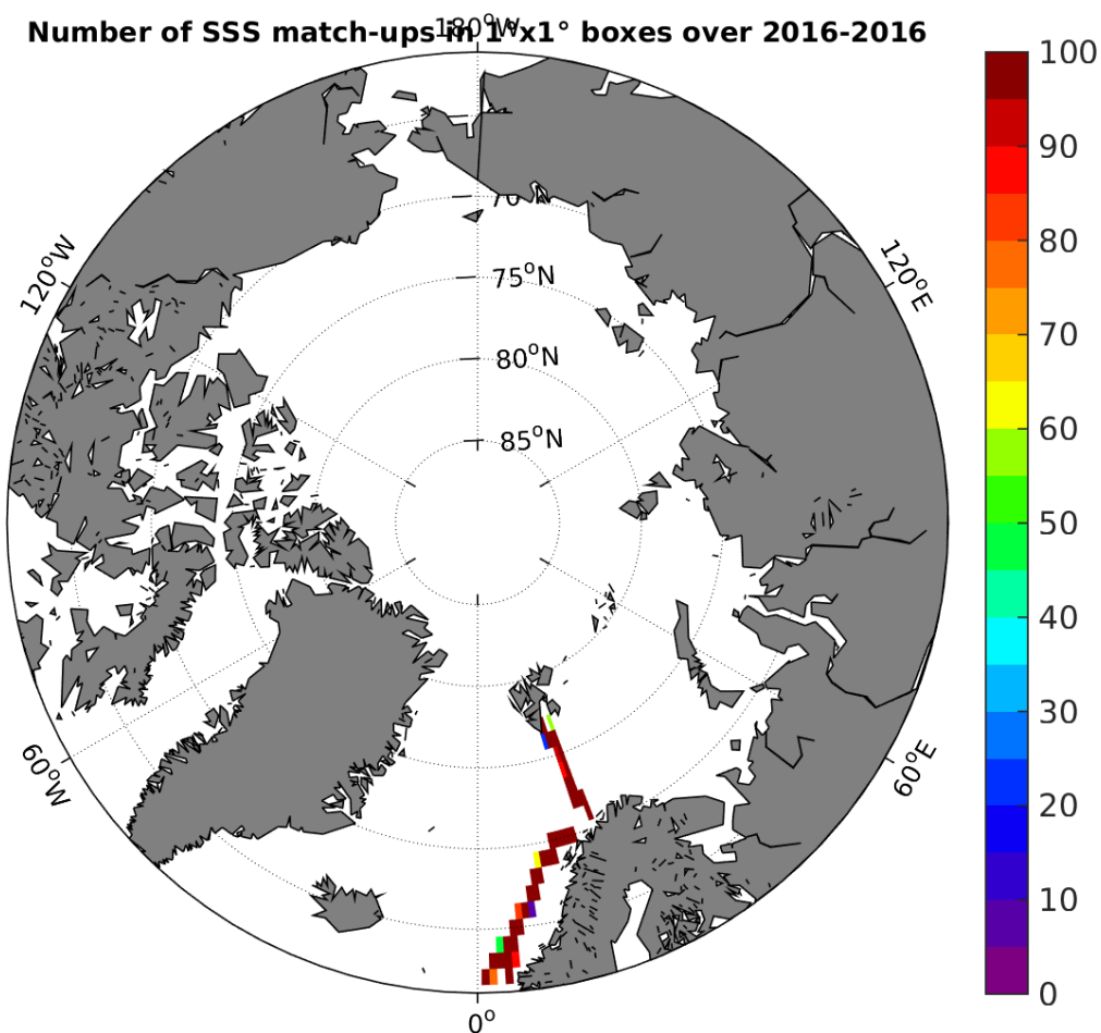
Figure 4: Number of SSS match-ups between TSG-GOSUD-Research-vessel SSS and the SMAP-L3-RSS-V2-MONTHLY-0.25DEG-40KM SSS product for the Arctic Ocean Pi-MEP region over 1°x1° boxes and for the full satellite product period.
