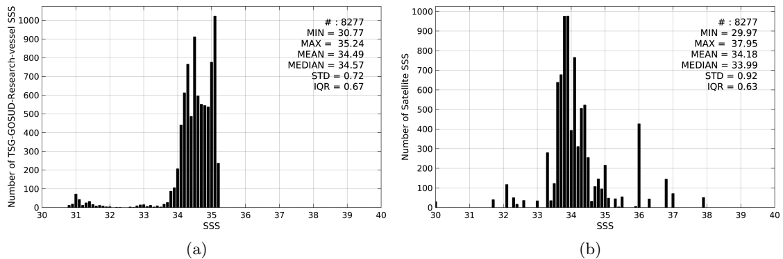
Figure 2: Histograms of SSS from TSG-GOSUD-Research-vessel (a) and SMAP-L3-RSS-V2-MONTHLY-0.25DEG-40KM (b) considering all match-up pairs per bins of 0.1 over the Arctic Ocean Pi-MEP region and for the full satellite product period.
