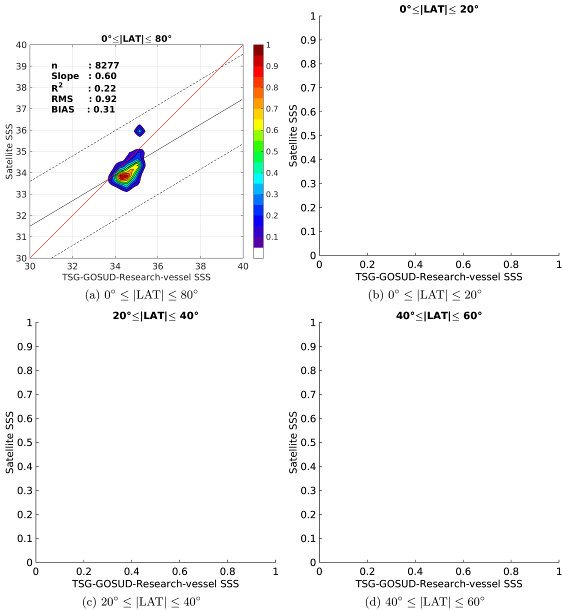
Figure 9: Contour maps of the concentration of SMAP-L3-RSS-V2-MONTHLY-0.25DEG-40KM SSS (y-axis) versus TSG-GOSUD-Research-vessel SSS (x-axis) at match-up pairs for different latitude bands. For each plot, the red line shows x=y . The black thin and dashed lines indicate a linear fit through the data cloud and the \pm 95\% confidence levels, respectively. The number match-up pairs n , the slope and R^2 coefficient of the linear fit, the root mean square (RMS) and the mean bias between satellite and in situ data are indicated for each latitude band in each plots.
