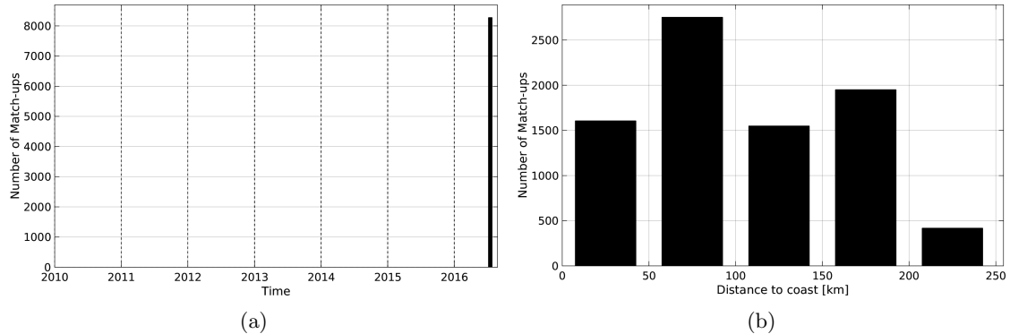
Figure 1: Number of match-ups between TSG-GOSUD-Research-vessel and SMAP-L3-RSS-V2-MONTHLY-0.25DEG-40KM SSS as a function of time (a) and as function of the distance to coast (b) over the Arctic Ocean Pi-MEP region and for the full satellite product period.
