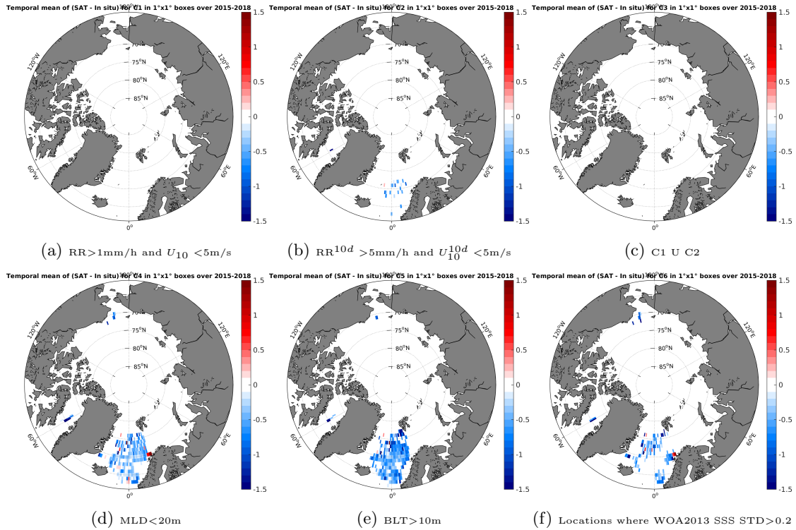
Figure 12: Temporal mean gridded over spatial boxes of size 1^\circ \times 1^\circ of \Delta SSS (SMAP-L3-RSS-V2-MONTHLY-0.25DEG-40KM - Argo) for 6 different subdatasets corresponding to:RR > 1mm/h and U_{10} < 5 m/s (a), RR^{10d} > 5 mm/h and U_{10}^{10d} < 5 m/s (b), C1 U C2 (c),MLD < 20m (d),BLT > 10m (e),Locations where WOA2013 SSS STD > 0.2 (f).
