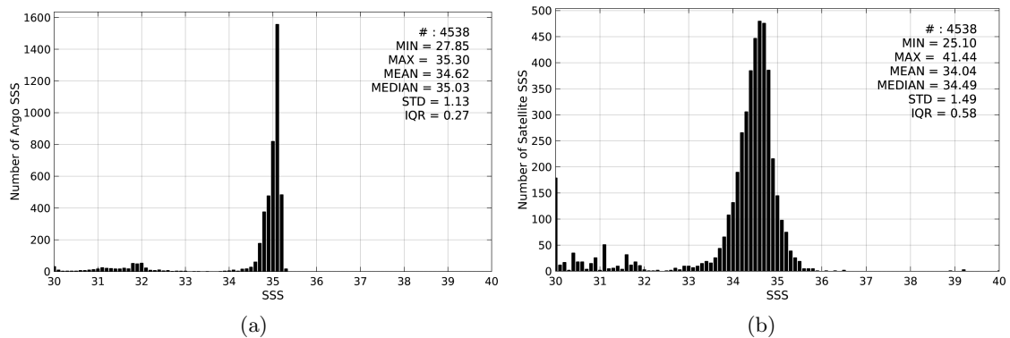
Figure 2: Histograms of SSS from Argo (a) and SMAP-L3-RSS-V2-MONTHLY-0.25DEG-40KM (b) considering all match-up pairs per bins of 0.1 over the Arctic Ocean Pi-MEP region and for the full satellite product period.
