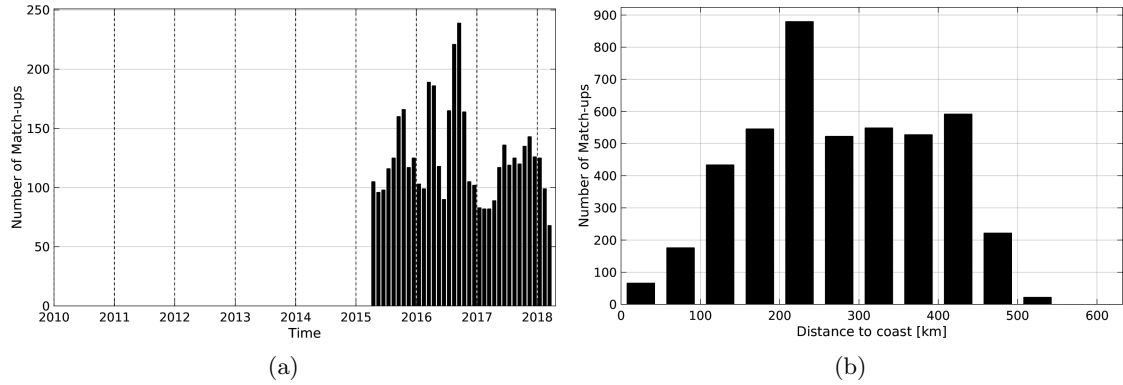
Figure 1: Number of match-ups between Argo and SMAP-L3-RSS-V2-MONTHLY-0.25DEG-40KM SSS as a function of time (a) and as function of the distance to coast (b) over the Arctic Ocean Pi-MEP region and for the full satellite product period.
