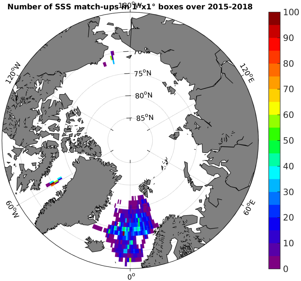
Figure 4: Number of SSS match-ups between Argo SSS and the SMAP-L3-RSS-V2-MONTHLY-0.25DEG-40KM SSS product for the Arctic Ocean Pi-MEP region over 1°x1° boxes and for the full satellite product period.
