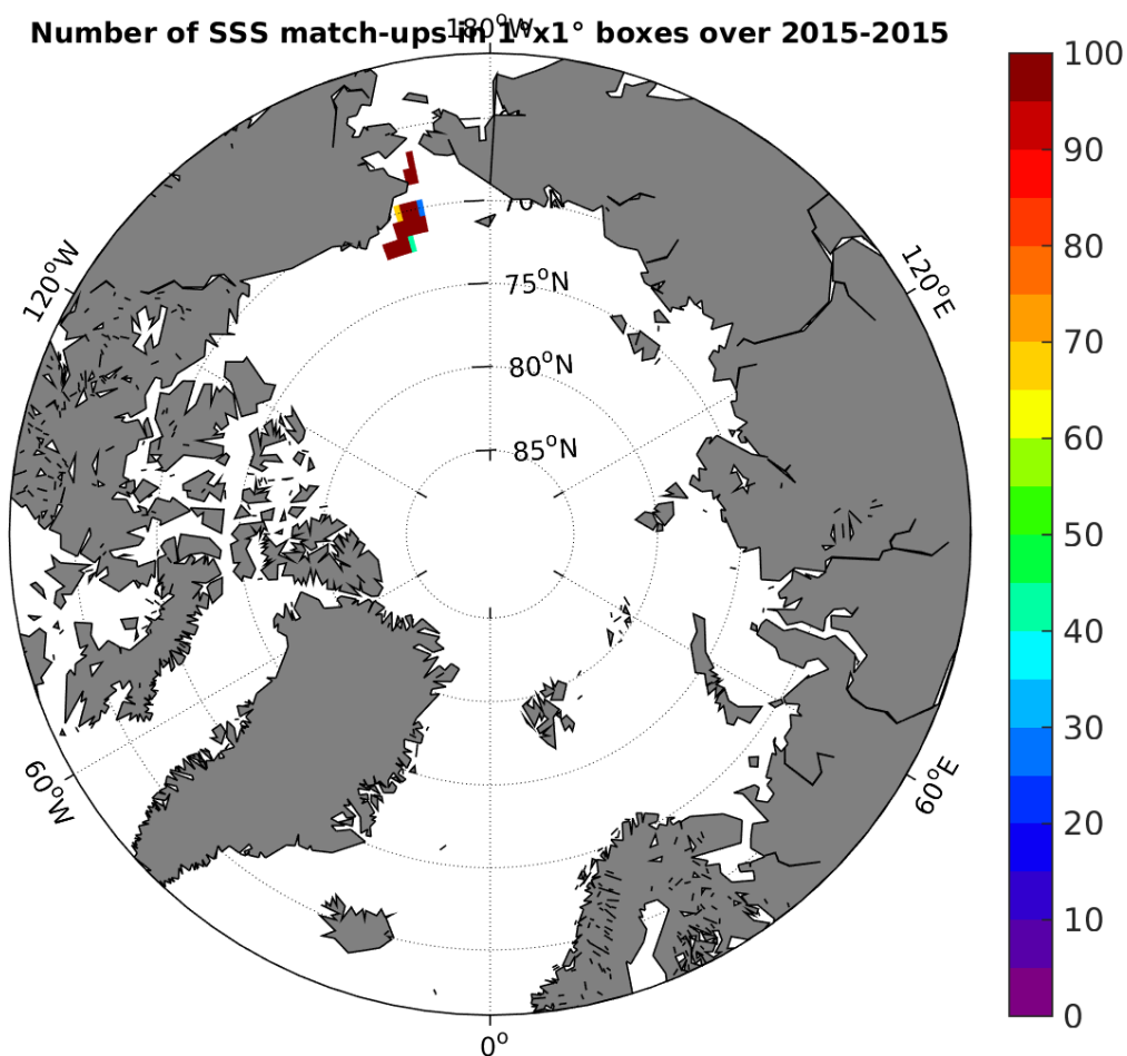
Figure 4: Number of SSS match-ups between TSG-SAMOS SSS and the SMAP-L3-RSS-V2-MONTHLY-70KM SSS product for the Arctic Ocean Pi-MEP region over 1°x1° boxes and for the full satellite product period.
