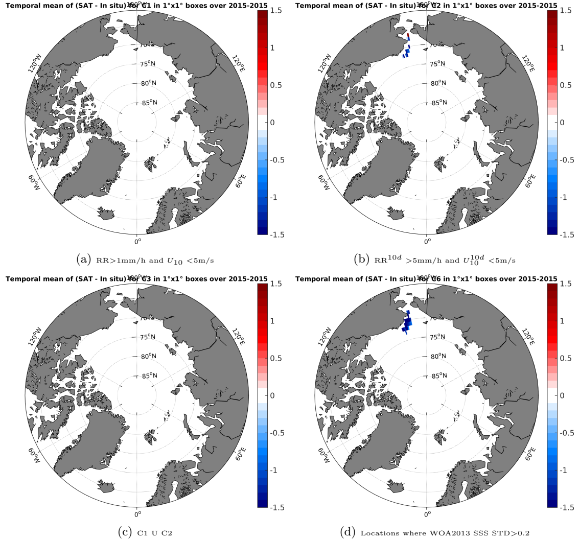
Figure 12: Temporal mean gridded over spatial boxes of size 1^\circ \times 1^\circ of \Delta SSS (SMAP-L3-RSS-V2-MONTHLY-70KM - TSG-SAMOS) for 4 different subdatasets corresponding to: RR > 1\text{mm/h} and U_{10} < 5\text{m/s} (a), RR^{10d} > 5\text{mm/h} and U_{10}^{10d} < 5\text{m/s} (b), C1 U C2 (c), Locations where WOA2013 SSS STD > 0.2 (d).
