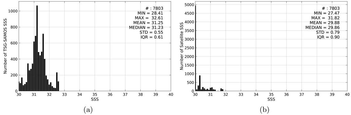
Figure 2: Histograms of SSS from TSG-SAMOS (a) and SMAP-L3-RSS-V2-MONTHLY-70KM (b) considering all match-up pairs per bins of 0.1 over the Arctic Ocean Pi-MEP region and for the full satellite product period.
