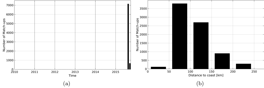
Figure 1: Number of match-ups between TSG-SAMOS and SMAP-L3-RSS-V2-MONTHLY-70KM SSS as a function of time (a) and as function of the distance to coast (b) over the Arctic Ocean Pi-MEP region and for the full satellite product period.
