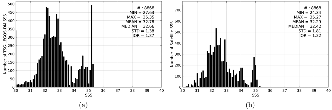
Figure 2: Histograms of SSS from TSG-LEGOS-DM (a) and SMAP-L3-RSS-V2-MONTHLY-70KM (b) considering all match-up pairs per bins of 0.1 over the Arctic Ocean Pi-MEP region and for the full satellite product period.
