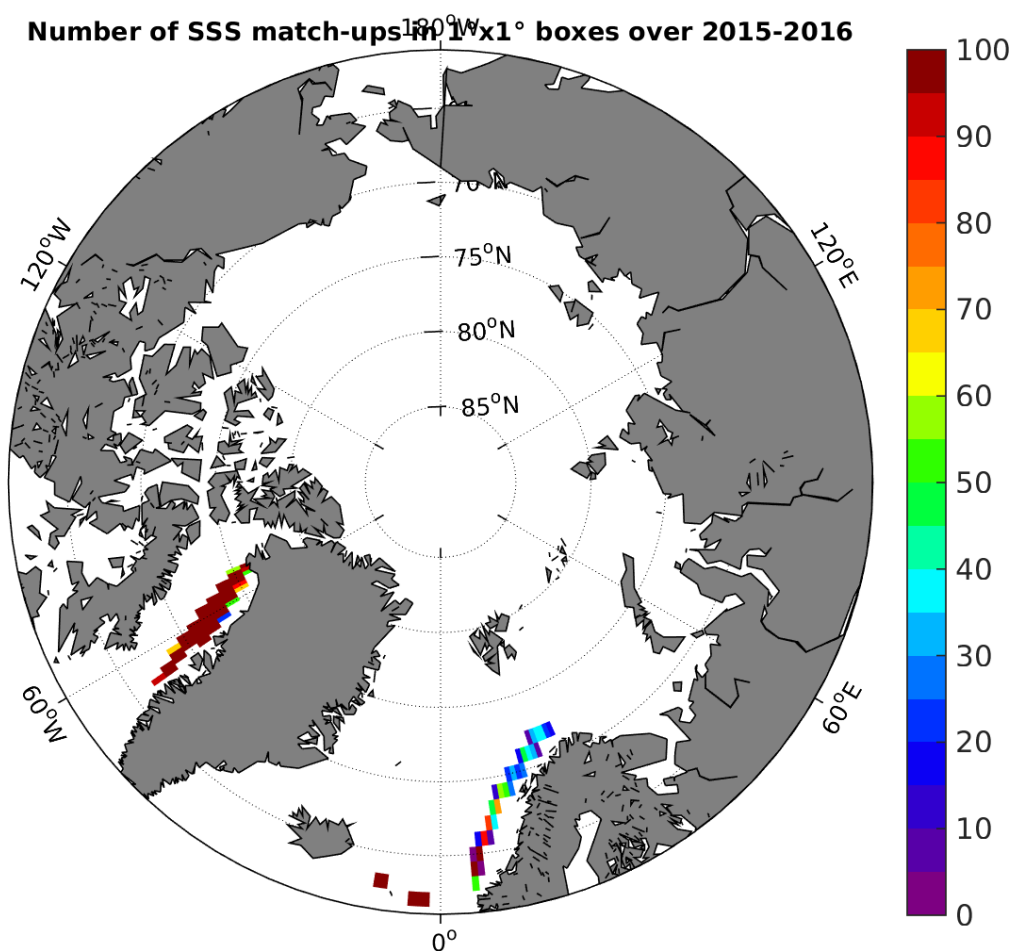
Figure 4: Number of SSS match-ups between TSG-LEGOS-DM SSS and the SMAP-L3-RSS-V2-MONTHLY-70KM SSS product for the Arctic Ocean Pi-MEP region over 1°x1° boxes and for the full satellite product period.
