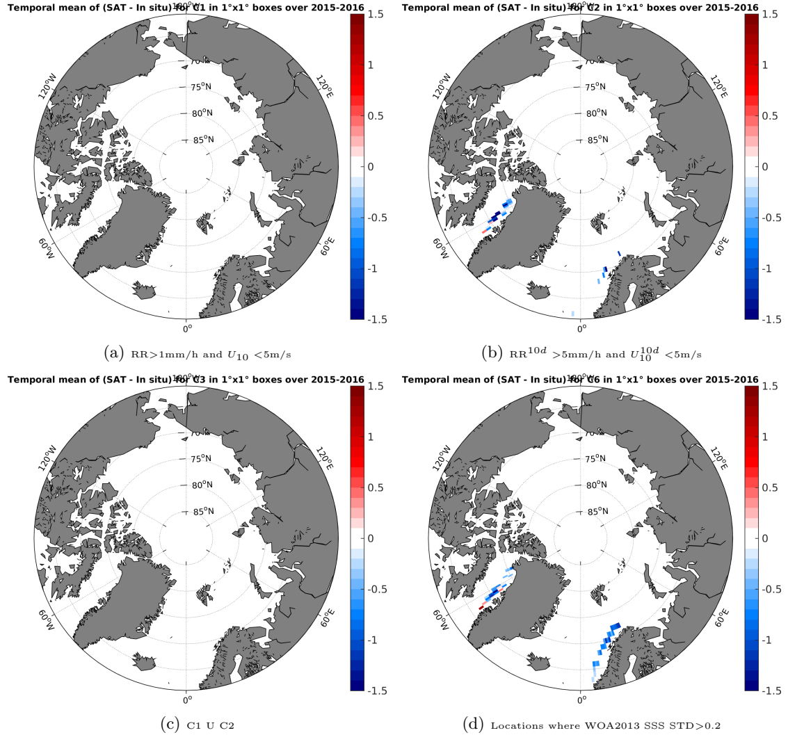
Figure 12: Temporal mean gridded over spatial boxes of size 1^\circ \times 1^\circ of \Delta SSS (SMAP-L3-RSS-V2-MONTHLY-70KM - TSG-LEGOS-DM) for 4 different subdatasets corresponding to: RR > 1\text{mm/h} and U_{10} < 5\text{m/s} (a), RR^{10d} > 5\text{mm/h} and U_{10}^{10d} < 5\text{m/s} (b), C1 U C2 (c), Locations where WOA2013 SSS STD > 0.2 (d).
