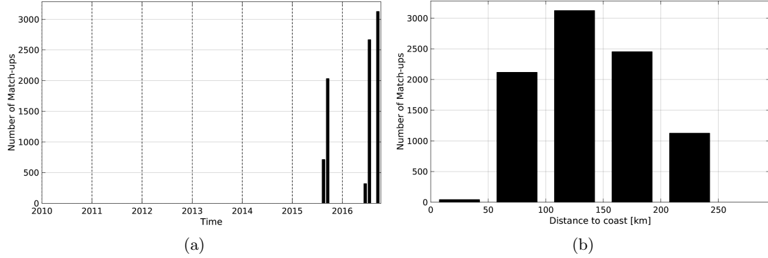
Figure 1: Number of match-ups between TSG-LEGOS-DM and SMAP-L3-RSS-V2-MONTHLY-70KM SSS as a function of time (a) and as function of the distance to coast (b) over the Arctic Ocean Pi-MEP region and for the full satellite product period.
