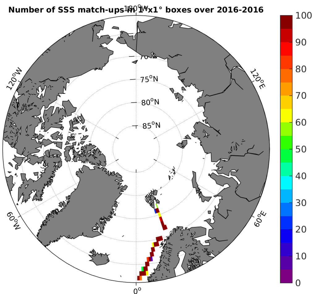
Figure 4: Number of SSS match-ups between TSG-GOSUD-Research-vessel SSS and the SMAP-L3-RSS-V2-MONTHLY-70KM SSS product for the Arctic Ocean Pi-MEP region over 1°x1° boxes and for the full satellite product period.
