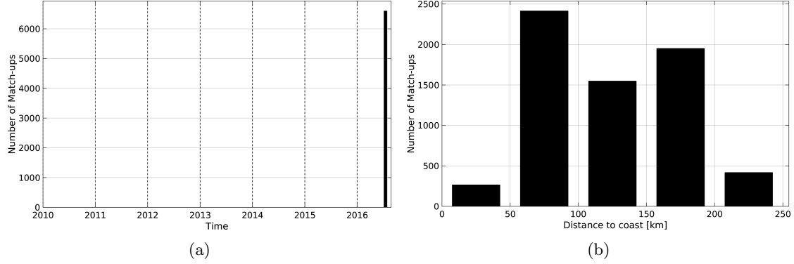
Figure 1: Number of match-ups between TSG-GOSUD-Research-vessel and SMAP-L3-RSS-V2-MONTHLY-70KM SSS as a function of time (a) and as function of the distance to coast (b) over the Arctic Ocean Pi-MEP region and for the full satellite product period.
