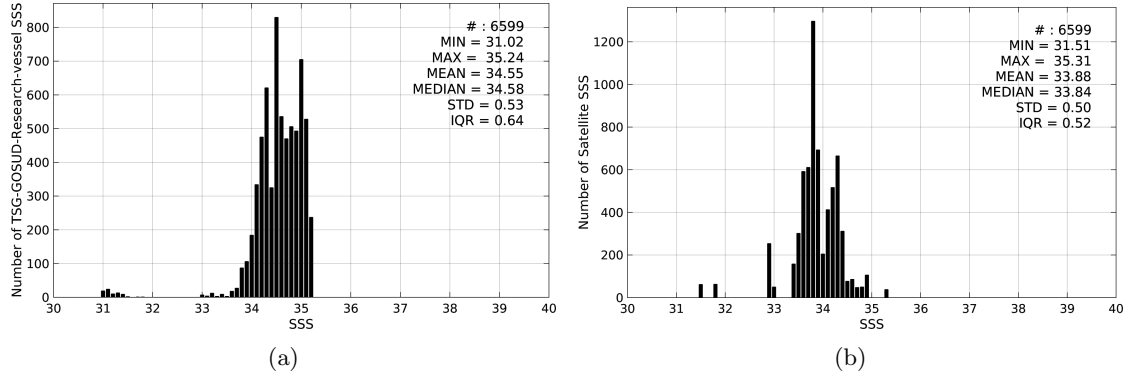
Figure 2: Histograms of SSS from TSG-GOSUD-Research-vessel (a) and SMAP-L3-RSS-V2-MONTHLY-70KM (b) considering all match-up pairs per bins of 0.1 over the Arctic Ocean Pi-MEP region and for the full satellite product period.
