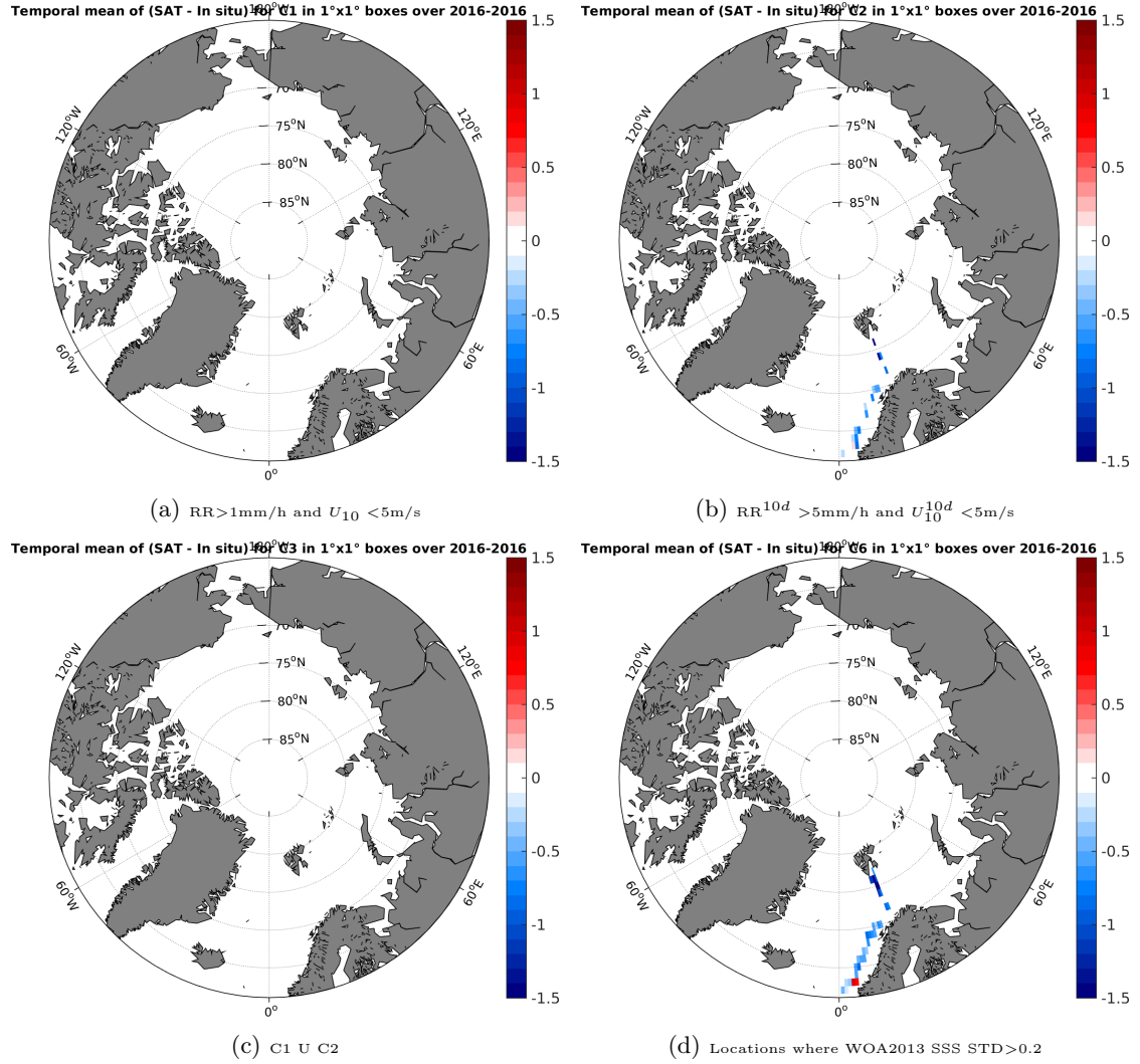
Figure 12: Temporal mean gridded over spatial boxes of size 1^\circ \times 1^\circ of \Delta SSS (SMAP-L3-RSS-V2-MONTHLY-70KM - TSG-GOSUD-Research-vessel) for 4 different subdatasets corresponding to: RR > 1\text{mm/h} and U_{10} < 5\text{m/s} (a), RR^{10d} > 5\text{mm/h} and U_{10}^{10d} < 5\text{m/s} (b), C1 U C2 (c), Locations where WOA2013 SSS STD > 0.2 (d).
