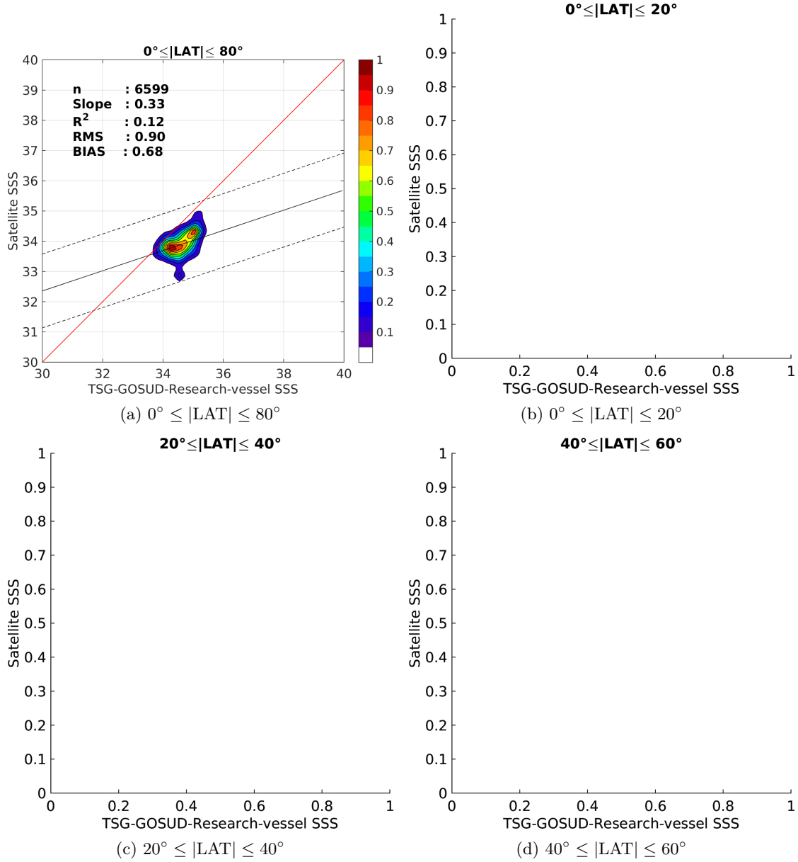
Figure 9: Contour maps of the concentration of SMAP-L3-RSS-V2-MONTHLY-70KM SSS (y-axis) versus TSG-GOSUD-Research-vessel SSS (x-axis) at match-up pairs for different latitude bands. For each plot, the red line shows x=y . The black thin and dashed lines indicate a linear fit through the data cloud and the \pm 95\% confidence levels, respectively. The number match-up pairs n , the slope and R^2 coefficient of the linear fit, the root mean square (RMS) and the mean bias between satellite and in situ data are indicated for each latitude band in each plots.
