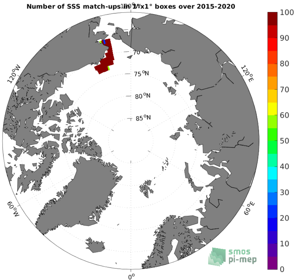
Figure 4: Number of SSS match-ups between TSG (SAMOS) SSS and the SMAP SSS L3 v5.0 - 8-Day running (JPL) SSS product for the Arctic Ocean Pi-MEP region over 1^\circ \times 1^\circ boxes and for the full satellite product period.
